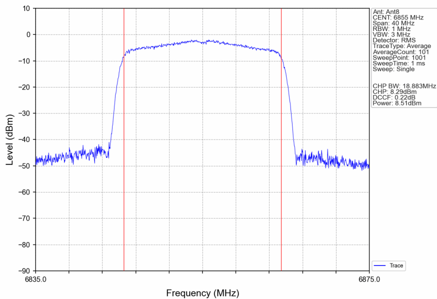
802.11ax(HEW20)_HCH_6855MHz_RU242_Left_Ant8_NTNV
