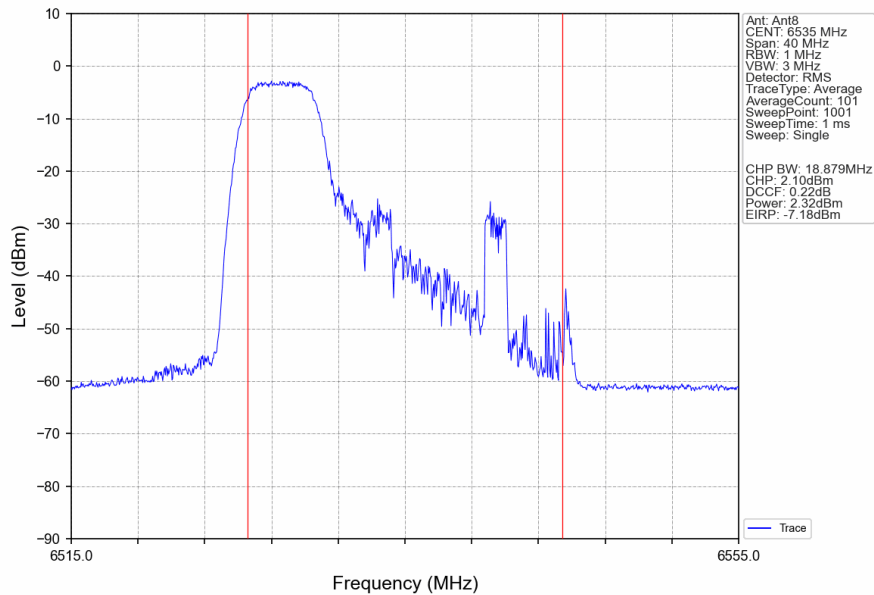
802.11ax(HEW20)_LCH_6535MHz_RU52_Left_Ant8_NTNV
