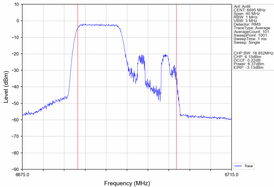
802.11ax(HEW20)_MCH_6695MHz_RU106_Left_Ant8_NTNV
