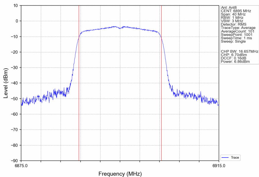
802.11a_LCH_6895MHz_Ant8_NTNV
