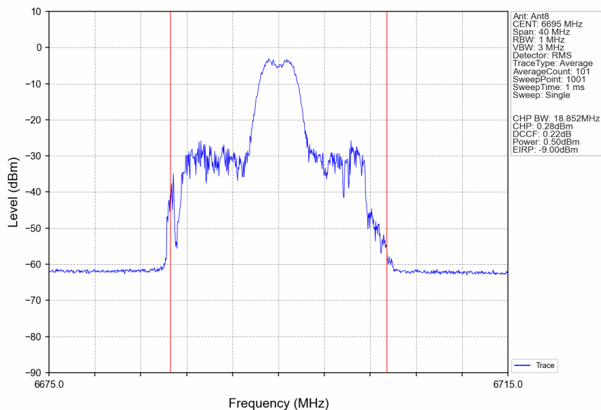
802.11ax(HEW20)_MCH_6695MHz_RU26_Mid_Ant8_NTNV
