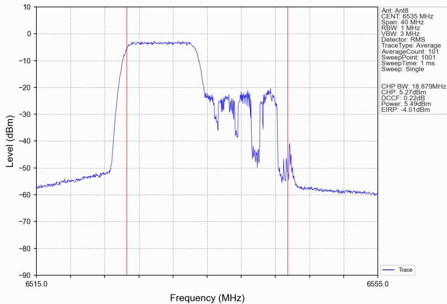
802.11ax(HEW20)_LCH_6535MHz_RU106_Left_Ant8_NTNV
