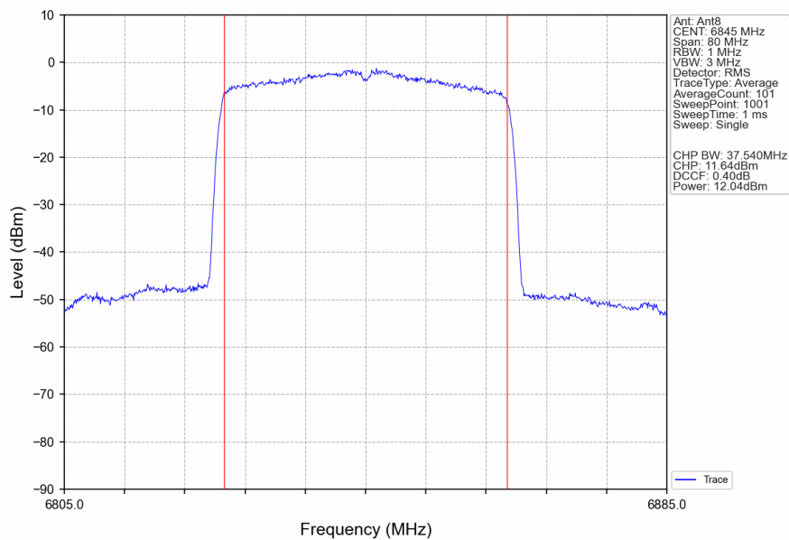
802.11ax(HEW40)_HCH_6845MHz_RU484_Left_Ant8_NTNV
