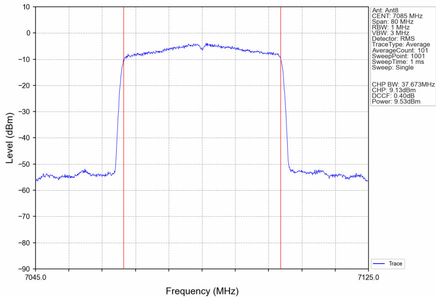
802.11ax(HEW40)_HCH_7085MHz_RU484_Left_Ant8_NTNV
