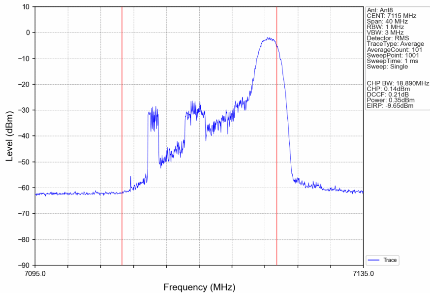
802.11ax(HEW20)_HCH_7115MHz_RU26_Right_Ant8_NTNV
