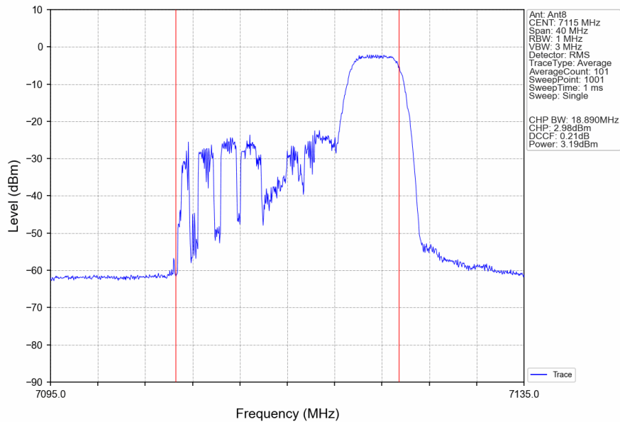
802.11ax(HEW20)_HCH_7115MHz_RU52_Right_Ant8_NTNV
