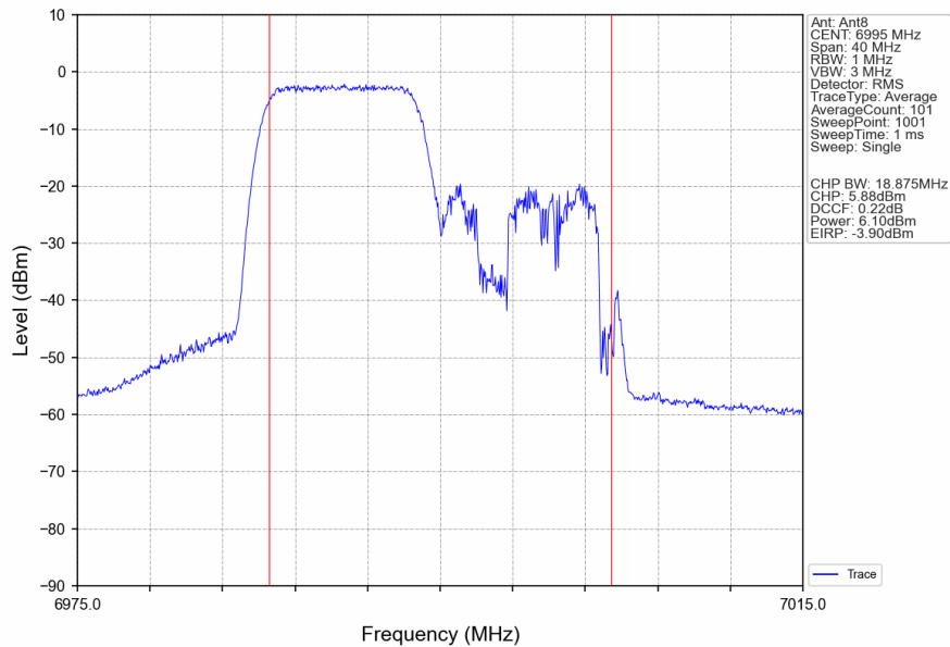
802.11ax(HEW20)_MCH_6995MHz_RU106_Left_Ant8_NTNV
