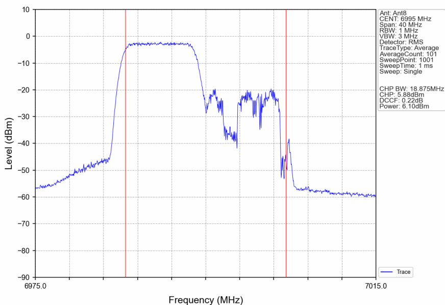
802.11ax(HEW20)_MCH_6995MHz_RU106_Left_Ant8_NTNV
