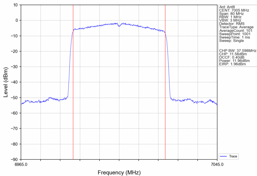
802.11ax(HEW40)_MCH_7005MHz_RU484_Left_Ant8_NTNV
