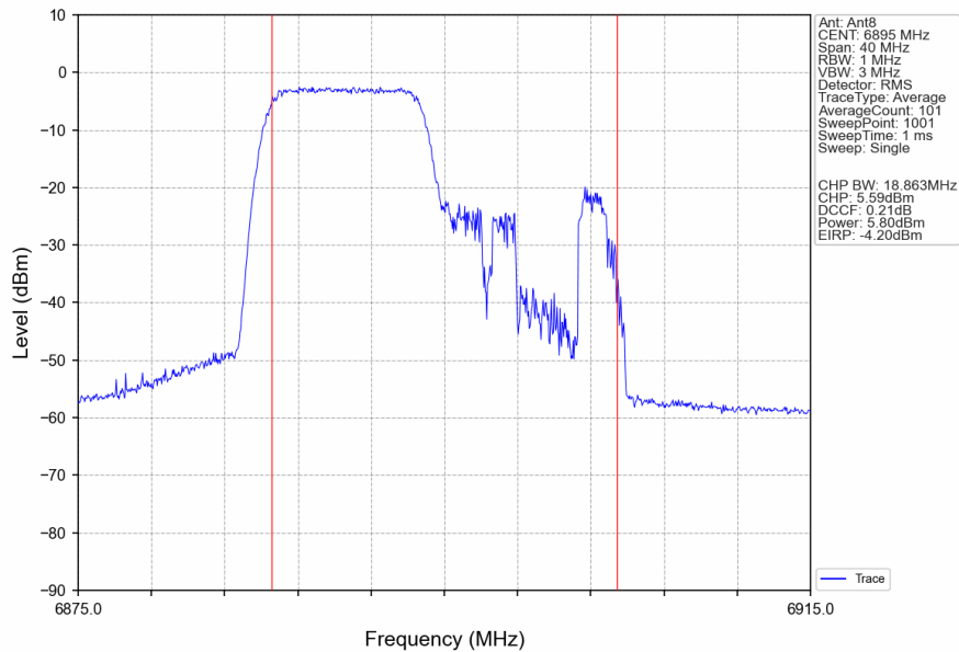
802.11ax(HEW20)_LCH_6895MHz_RU106_Left_Ant8_NTNV
