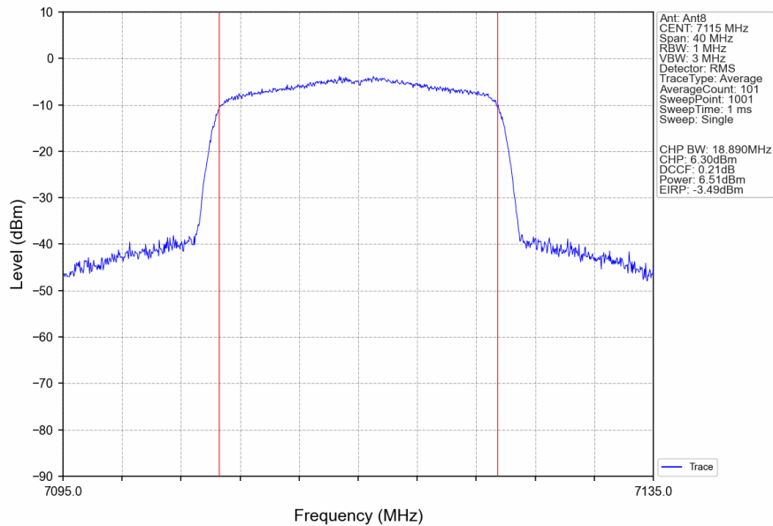
802.11ax(HEW20)_HCH_7115MHz_RU242_Left_Ant8_NTNV
