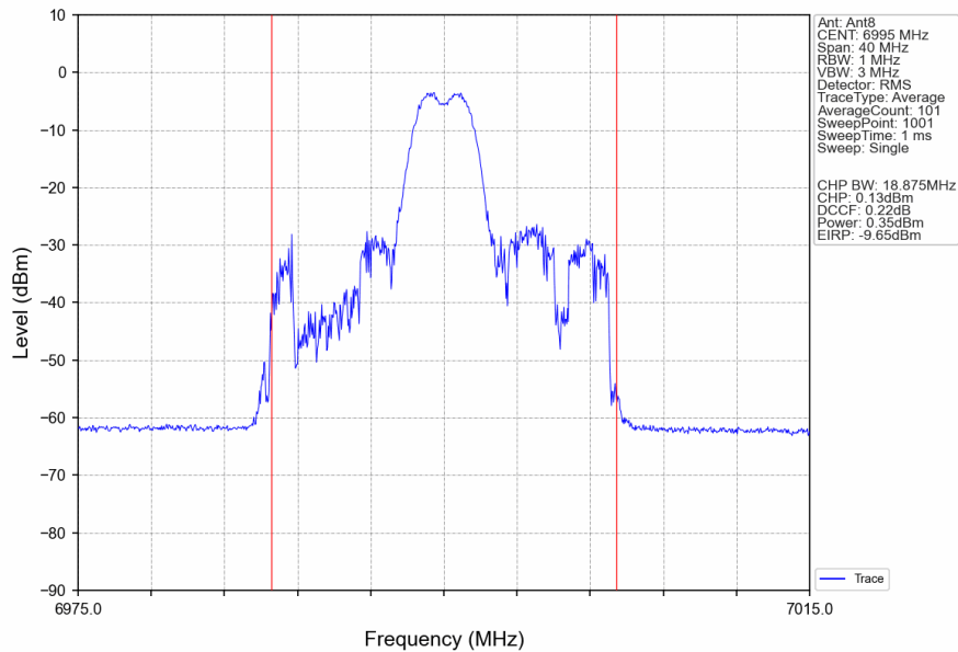
802.11ax(HEW20)_MCH_6995MHz_RU26_Mid_Ant8_NTNV
