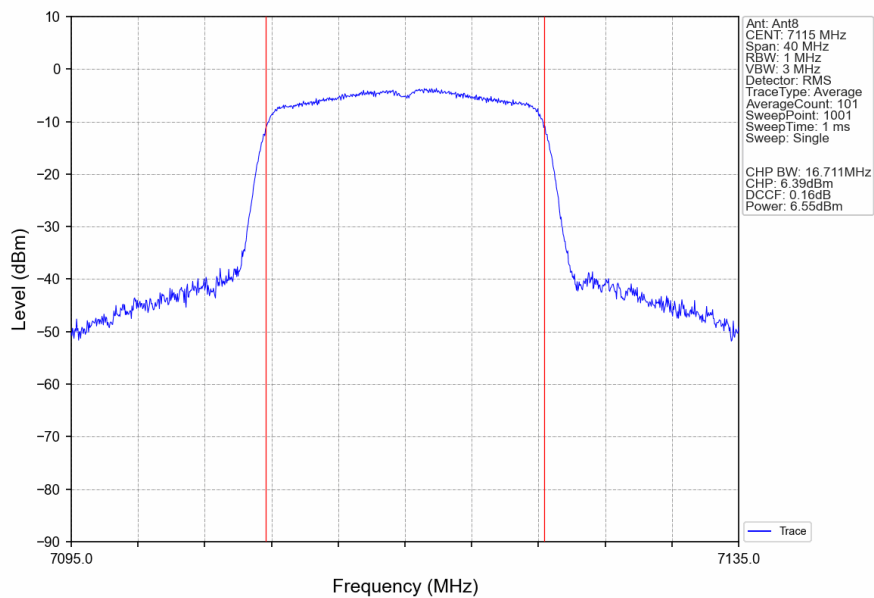
802.11a_HCH_7115MHz_Ant8_NTNV
