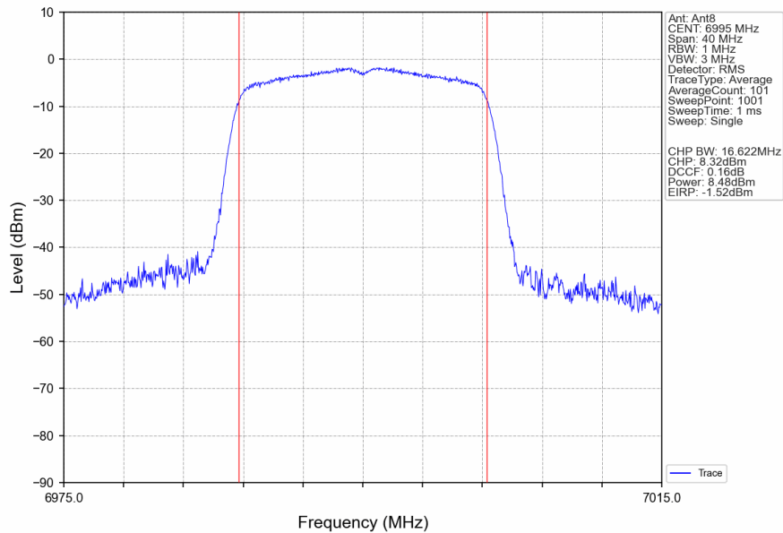
802.11a_MCH_6995MHz_Ant8_NTNV
