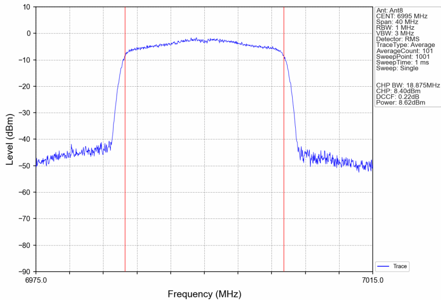
802.11ax(HEW20)_MCH_6995MHz_RU242_Left_Ant8_NTNV
