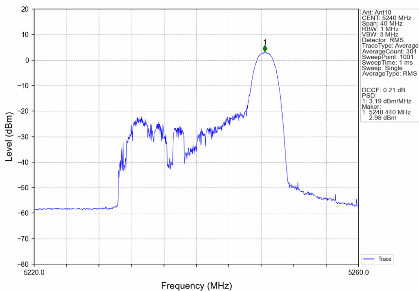
802.11ax(HEW20) HCH 5240MHz RU26 Right Ant10 NTN
