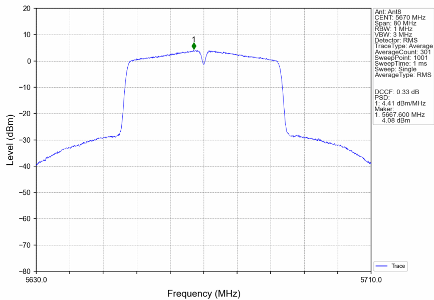
802.11n(HT40) HCH 5670MHz Ant8 NTN
