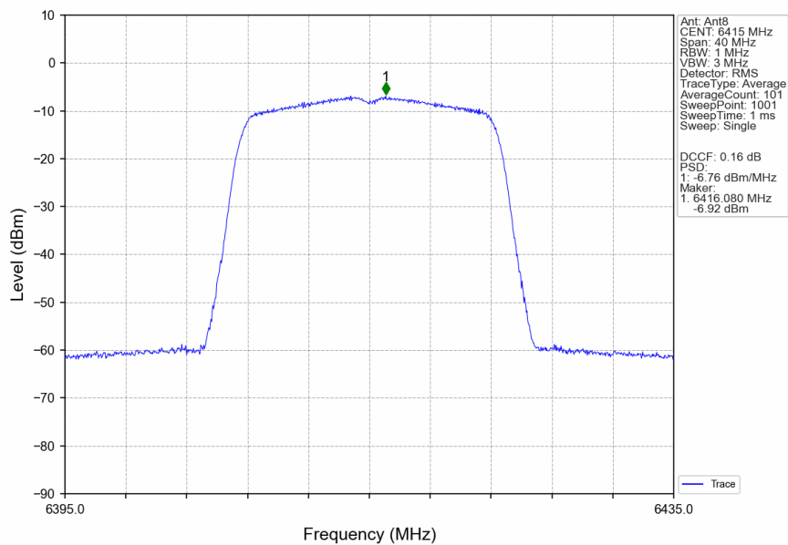
802.11a_HCH_6415MHz_Ant8_NTNV
