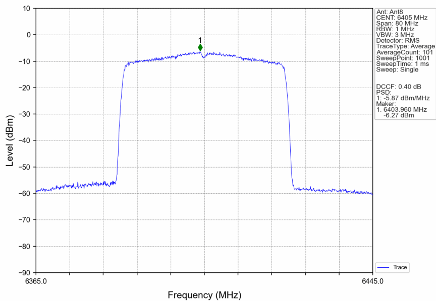
802.11ax(HEW40)_HCH_6405MHz_RU484_Left_Ant8_NTNV
