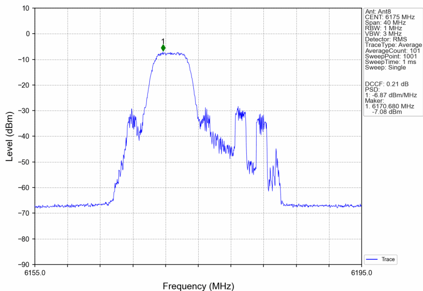
802.11ax(HEW20)_MCH_6175MHz_RU52_Mid_Ant8_NTNV
