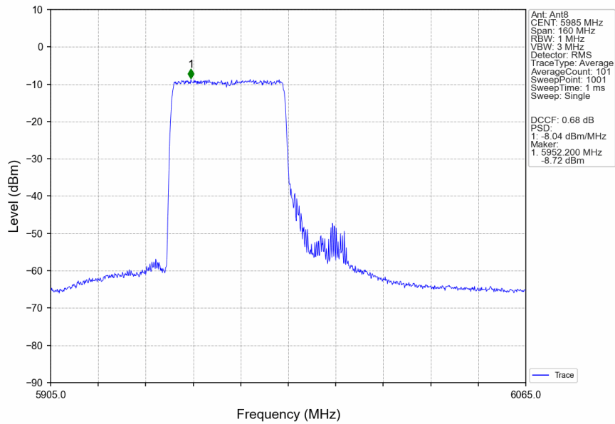
802.11ax(HEW80)_LCH_5985MHz_RU484_Left_MIMO_NTNV
