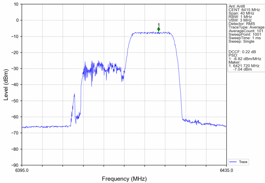
802.11ax(HEW20)_HCH_6415MHz_RU106_Right_MIMO_NTNV
