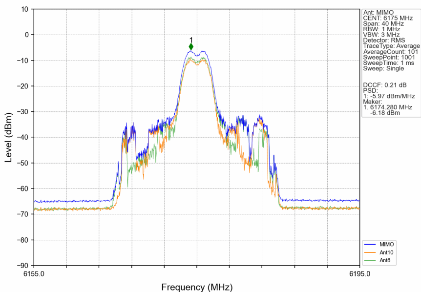
802.11ax(HEW20)_MCH_6175MHz_RU26_Mid_MIMO_NTNV
