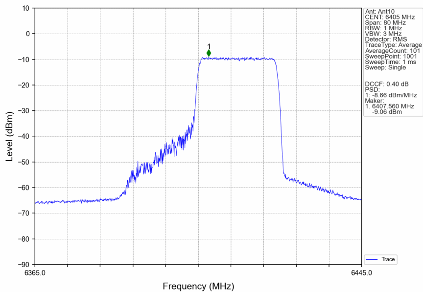
802.11ax(HEW40)_HCH_6405MHz_RU242_Right_Ant10_NTNV
