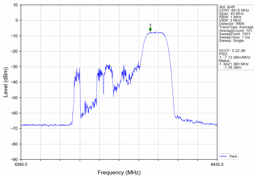
802.11ax(HEW20)_HCH_6415MHz_RU52_Right_Ant8_NTNV
