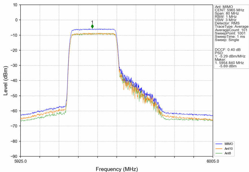
802.11ax(HEW40)_LCH_5965MHz_RU242_Left_MIMO_NTNV
