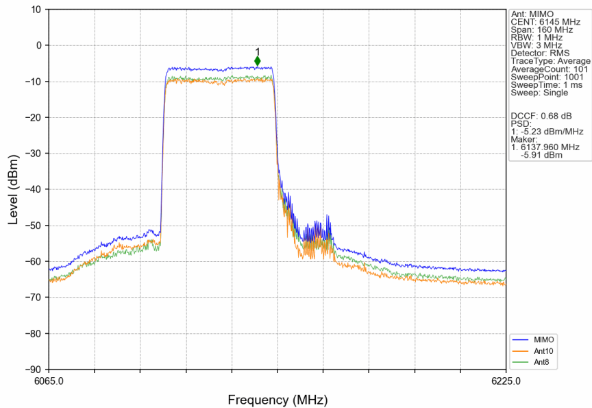
802.11ax(HEW80)_MCH_6145MHz_RU484_Left_MIMO_NTNV
