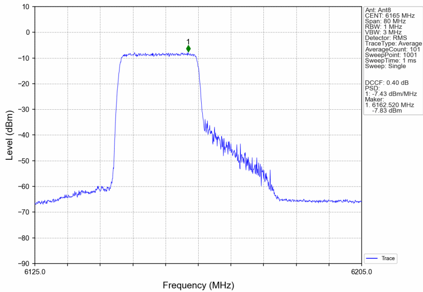
802.11ax(HEW40)_MCH_6165MHz_RU242_Left_MIMO_NTNV
