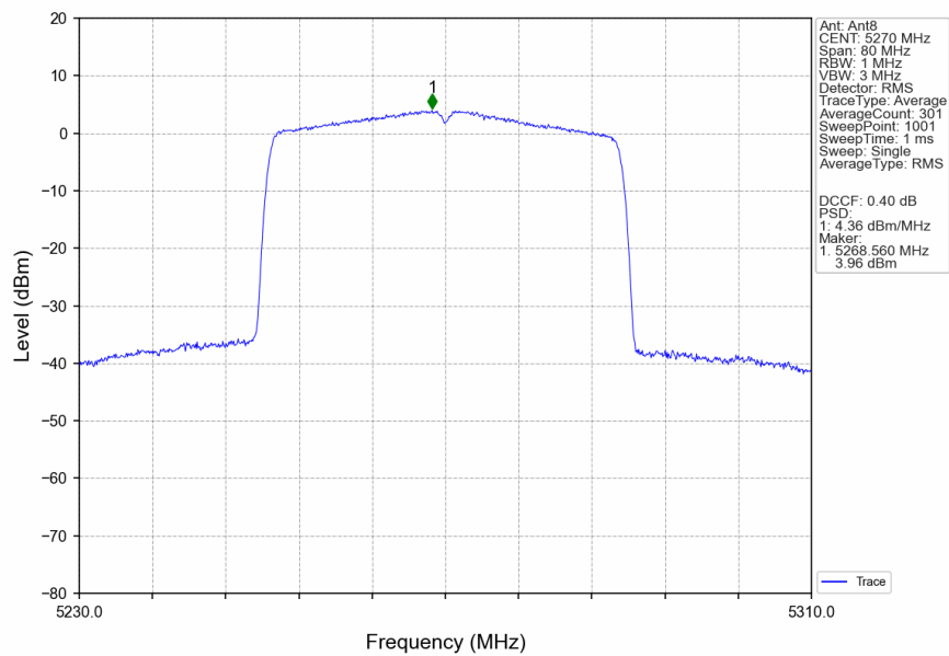
802.11ax(HEW40) LCH 5270MHz RU484 Left Ant8 NTN
