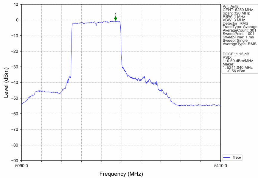
802.11ax(HEW160) MCH 5250MHz RU996 Left MIMO NTN
