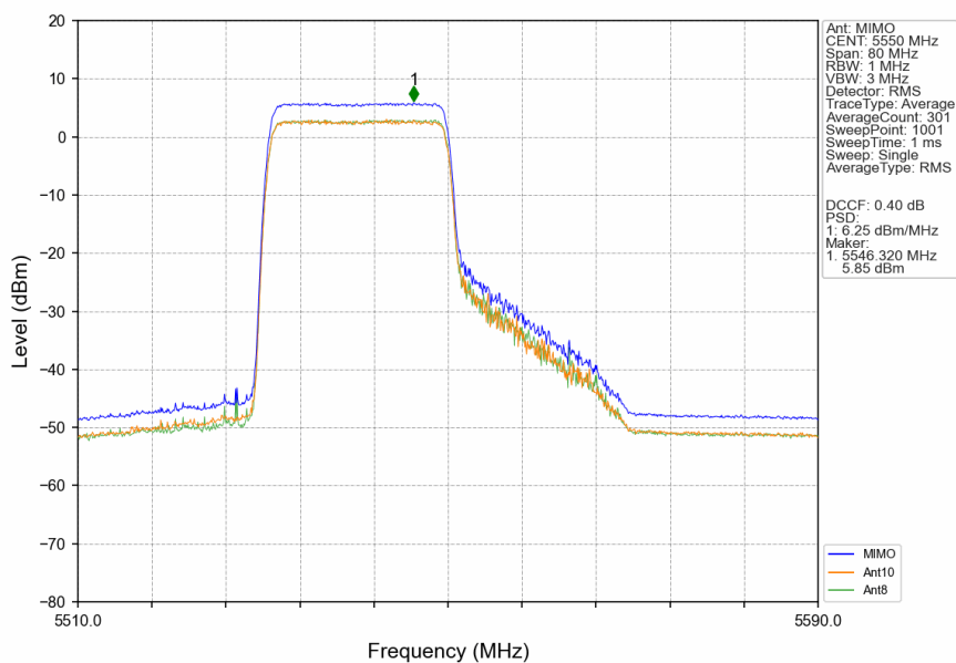
802.11ax(HEW40) MCH 5550MHz RU242 Left MIMO NTN
