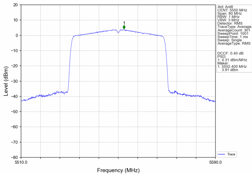
802.11ax(HEW40) MCH 5550MHz RU484 Left Ant8 NTN
