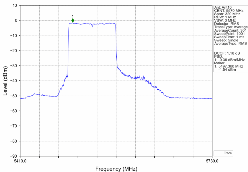
802.11ax(HEW160) MCH 5570MHz RU996 Left Ant10 NTN
