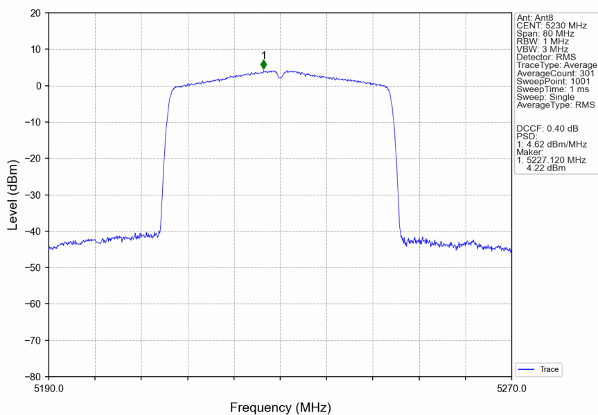
802.11ax(HEW40) HCH 5230MHz RU484 Left Ant8 NTN
