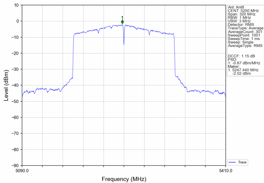
802.11ax(HEW160) MCH 5250MHz 2xRU996 Left Ant8 NTN
