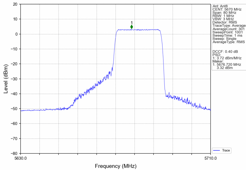
802.11ax(HEW40) HCH 5670MHz RU242 Right MIMO NTN
