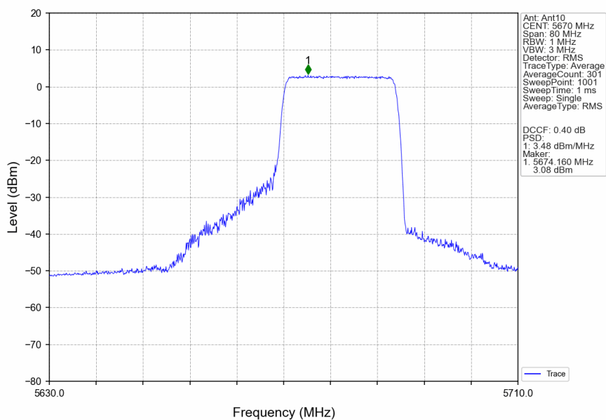
802.11ax(HEW40) HCH 5670MHz RU242 Right Ant10 NTN
