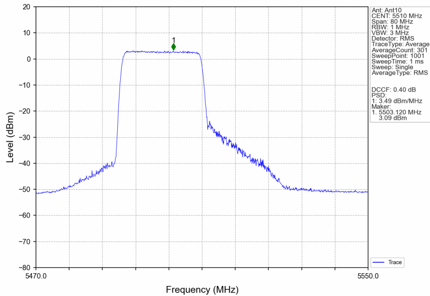
802.11ax(HEW40) LCH 5510MHz RU242 Left Ant10 NTN
