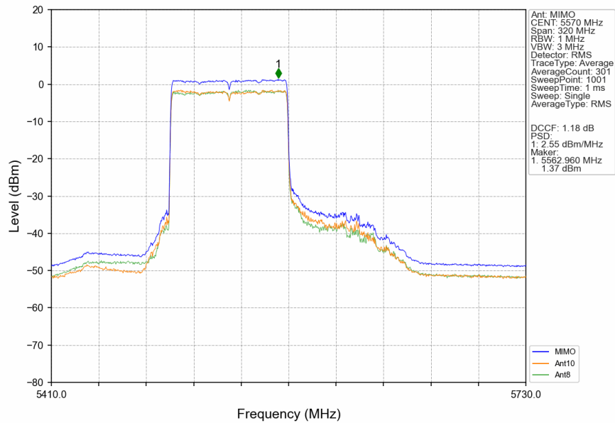
802.11ax(HEW160) MCH 5570MHz RU996 Left MIMO NTN
