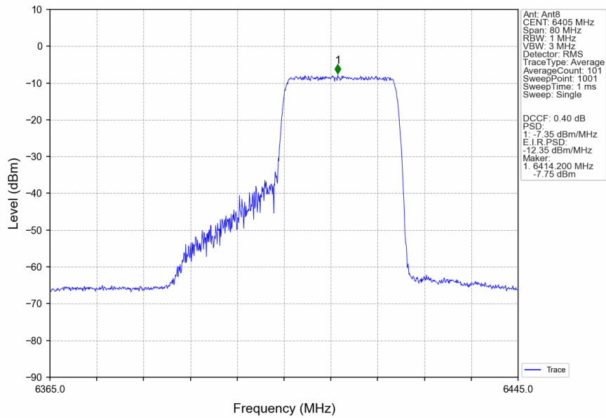
802.11ax(HEW40)_HCH_6405MHz_RU242_Right_MIMO_NTNV
