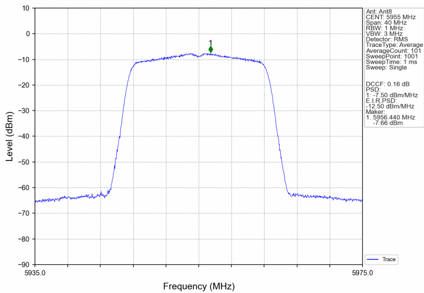
802.11a_LCH_5955MHz_Ant8_NTNV
