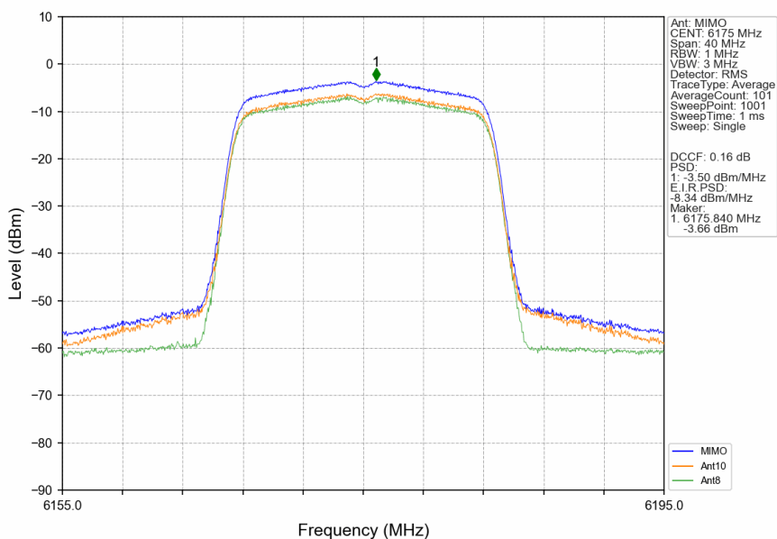
802.11a_MCH_6175MHz_MIMO_NTNV
