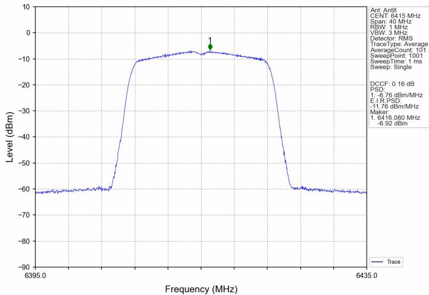
802.11a_HCH_6415MHz_Ant8_NTNV
