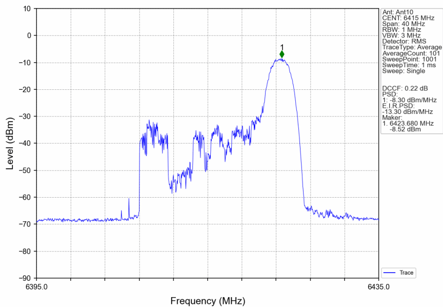
802.11ax(HEW20)_HCH_6415MHz_RU26_Right_Ant10_NTNV
