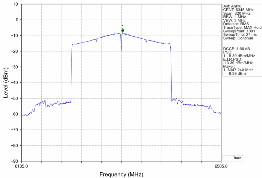
802.11ax(HEW160)_HCH_6345MHz_RU996_Right_Ant10_NTNV
