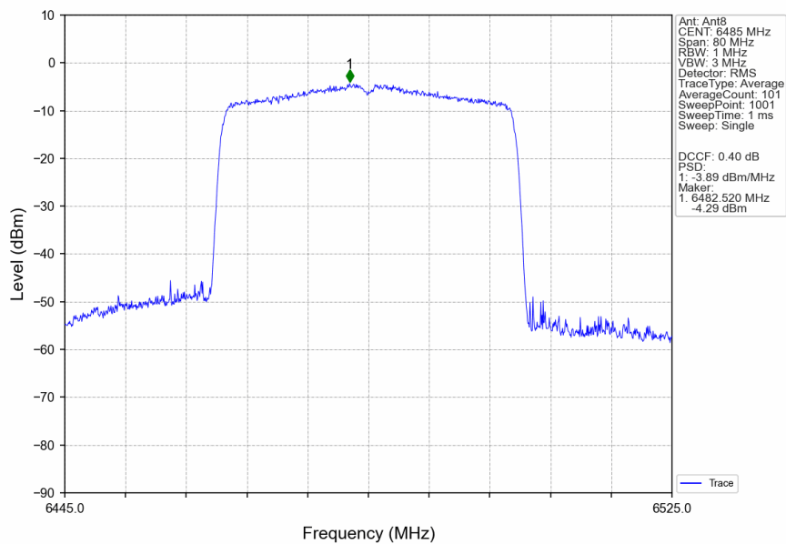
802.11ax(HEW40)_MCH_6485MHz_RU484_Left_Ant8_NTNV
