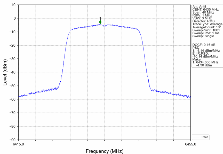
802.11a_LCH_6435MHz_Ant8_NTNV
