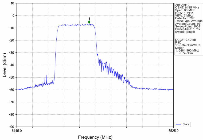
802.11ax(HEW40)_MCH_6485MHz_RU242_Left_Ant10_NTNV
