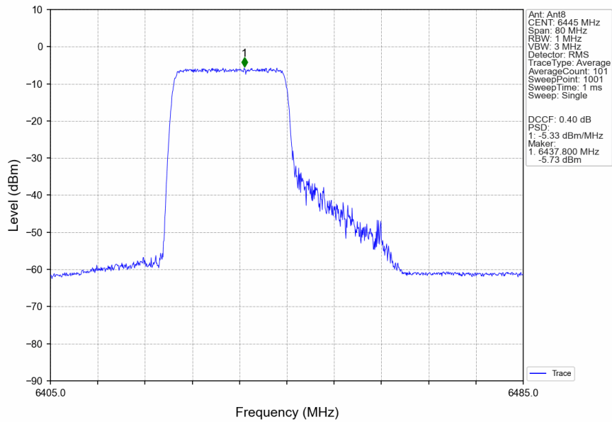
802.11ax(HEW40)_LCH_6445MHz_RU242_Left_MIMO_NTNV
