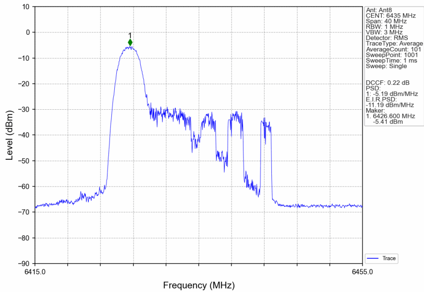
802.11ax(HEW20)_LCH_6435MHz_RU26_Left_MIMO_NTNV
