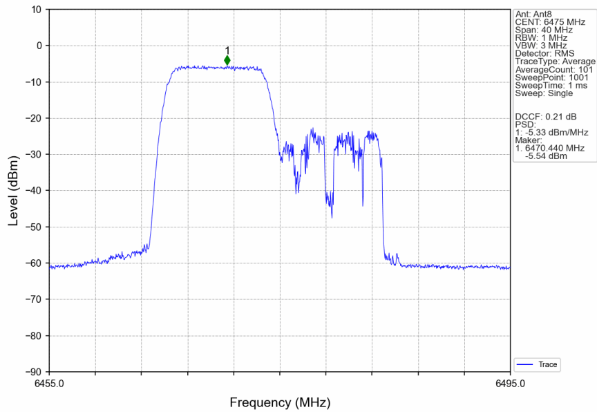
802.11ax(HEW20)_MCH_6475MHz_RU106_Left_MIMO_NTNV
