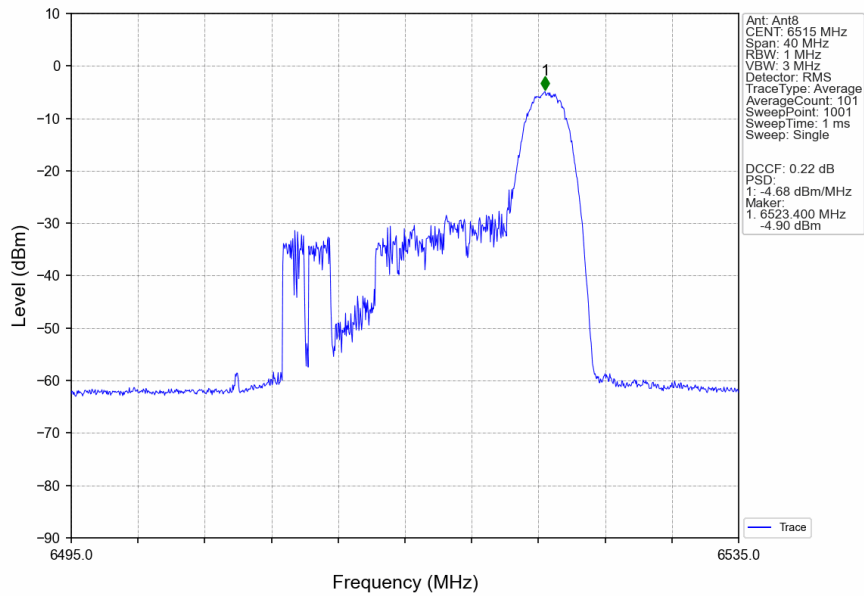
802.11ax(HEW20)_HCH_6515MHz_RU26_Right_MIMO_NTNV
