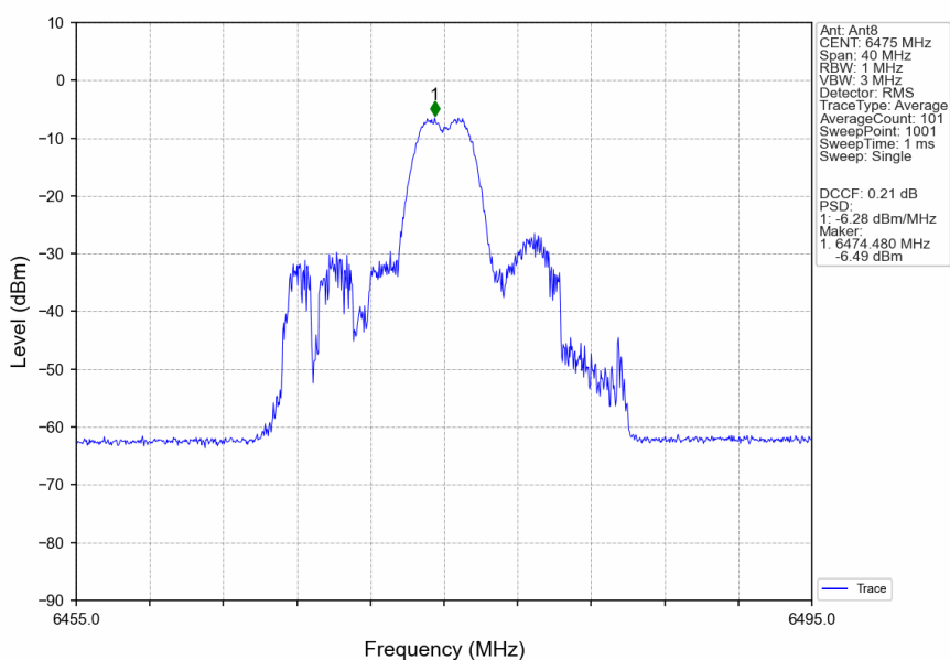
802.11ax(HEW20)_MCH_6475MHz_RU26_Mid_MIMO_NTNV
