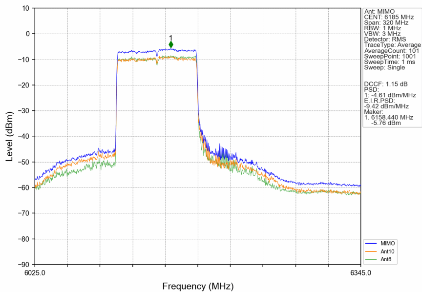
802.11ax(HEW160)_MCH_6185MHz_RU996_Left_MIMO_NTNV
