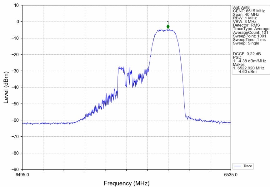
802.11ax(HEW20)_HCH_6515MHz_RU52_Right_Ant8_NTNV
