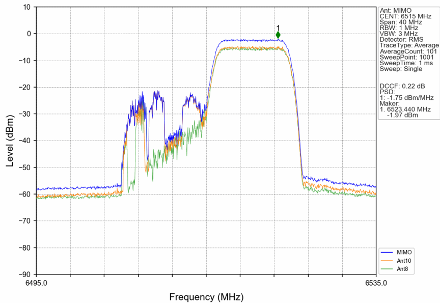
802.11ax(HEW20)_HCH_6515MHz_RU106_Right_MIMO_NTNV
