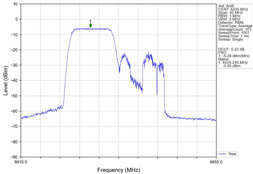
802.11ax(HEW20)_LCH_6435MHz_RU106_Left_MIMO_NTNV
