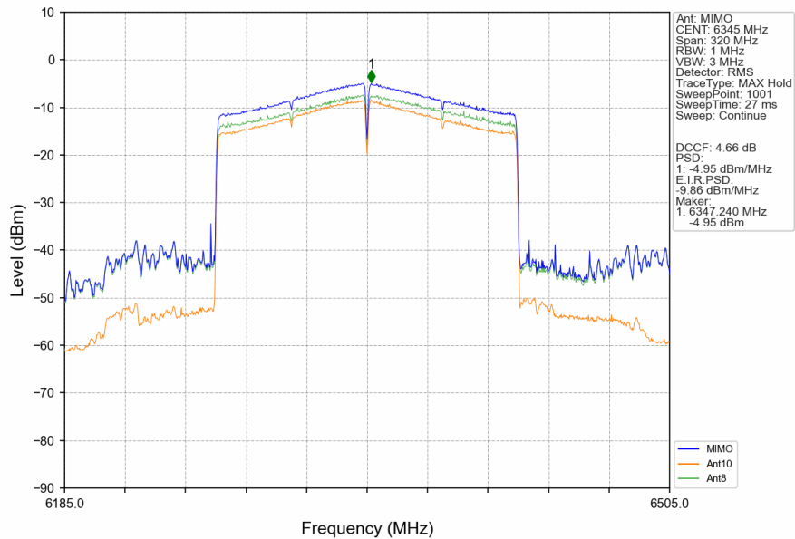
802.11ax(HEW160)_HCH_6345MHz_RU996_Right_MIMO_NTNV
