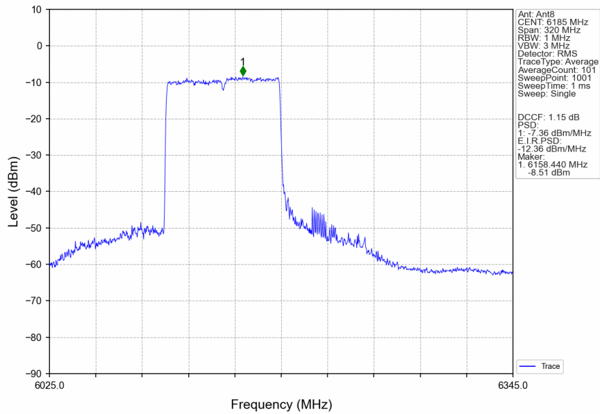
802.11ax(HEW160)_MCH_6185MHz_RU996_Left_MIMO_NTNV
