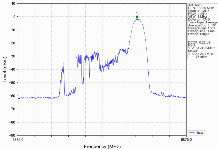
802.11ax(HEW20)_HCH_6855MHz_RU26_Right_MIMO_NTNV
