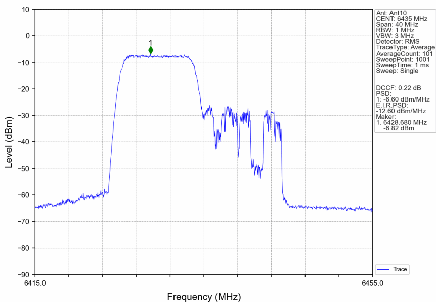
802.11ax(HEW20)_LCH_6435MHz_RU106_Left_Ant10_NTNV
