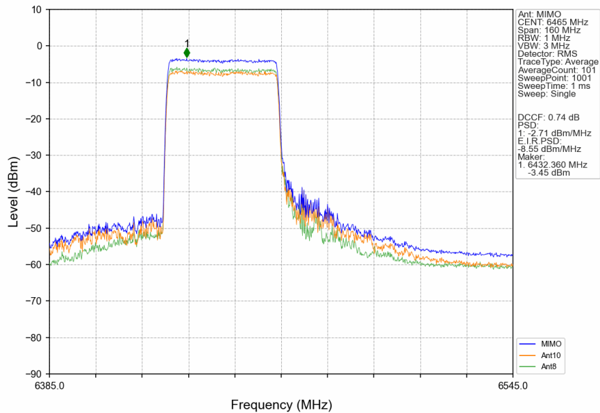
802.11ax(HEW80)_LCH_6465MHz_RU484_Left_MIMO_NTNV
