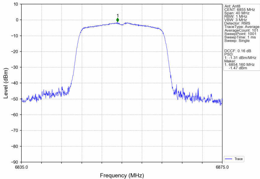
802.11a_HCH_6855MHz_Ant8_NTNV
