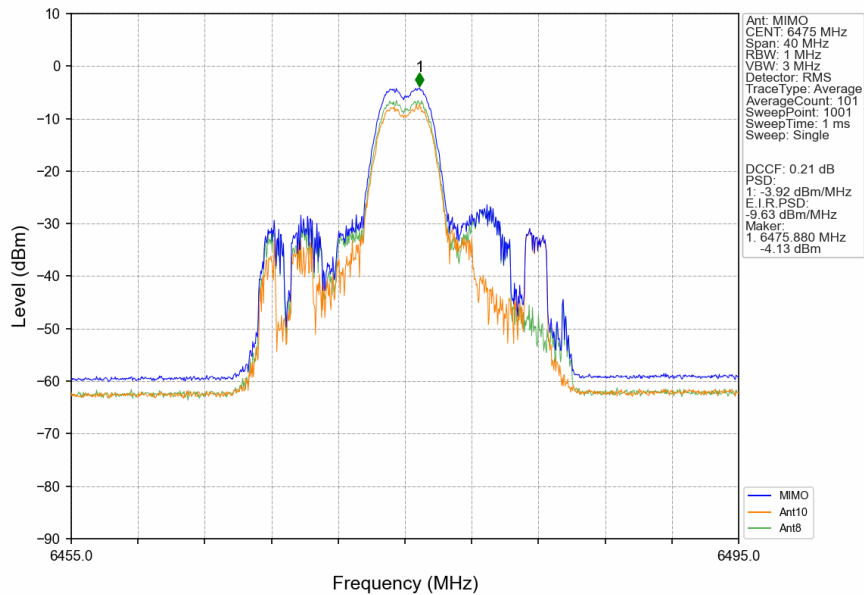
802.11ax(HEW20)_MCH_6475MHz_RU26_Mid_MIMO_NTNV
