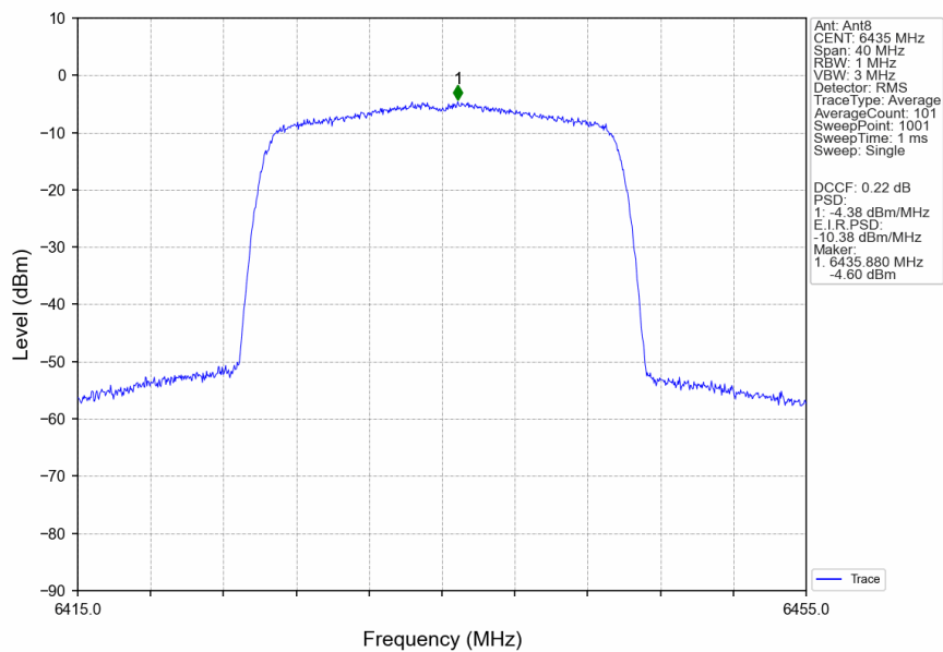
802.11ax(HEW20)_LCH_6435MHz_RU242_Left_Ant8_NTNV
