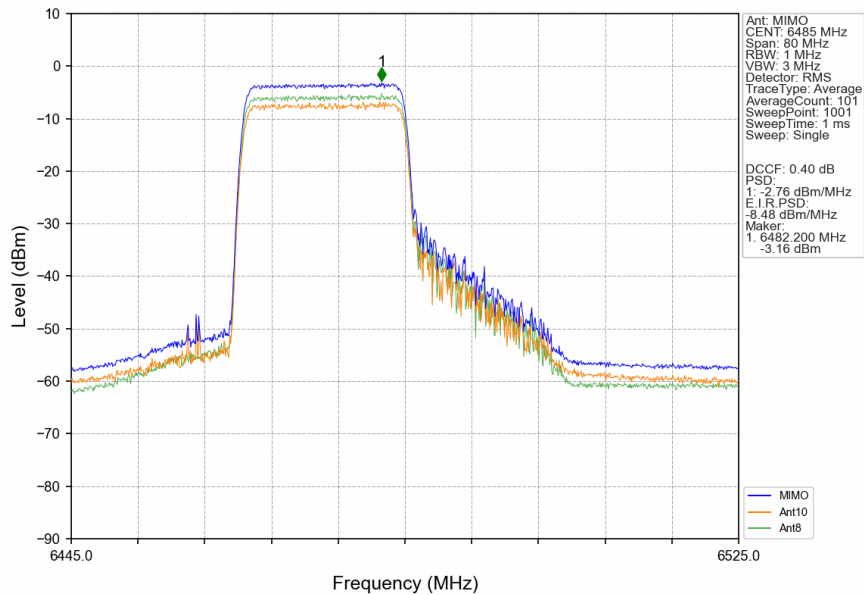
802.11ax(HEW40)_MCH_6485MHz_RU242_Left_MIMO_NTNV
