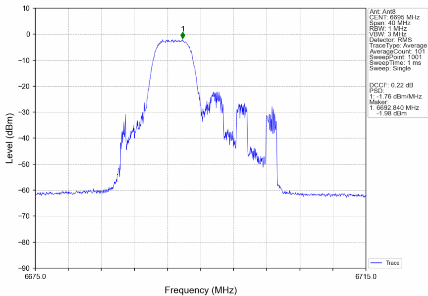
802.11ax(HEW20)_MCH_6695MHz_RU52_Mid_Ant8_NTNV
