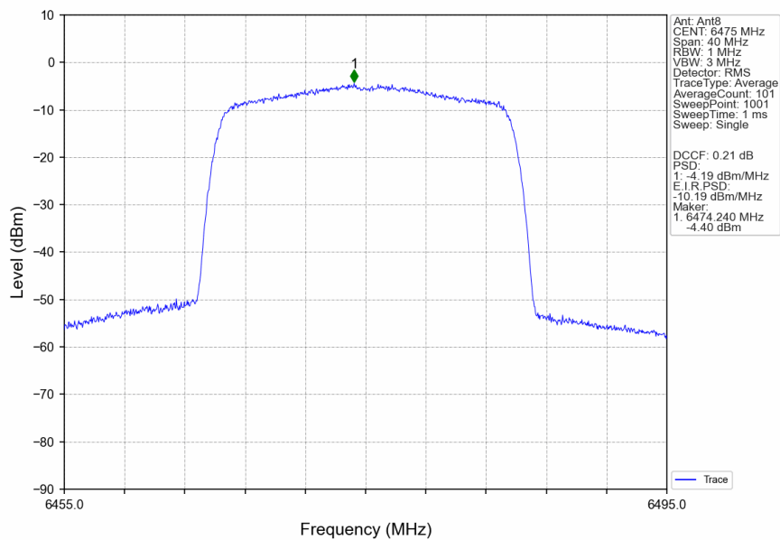
802.11ax(HEW20)_MCH_6475MHz_RU242_Left_Ant8_NTNV
