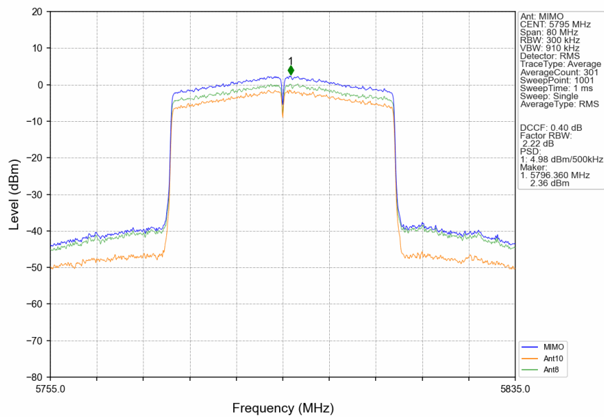
802.11ax(HEW40) HCH 5795MHz RU484 Left MIMO NTN
