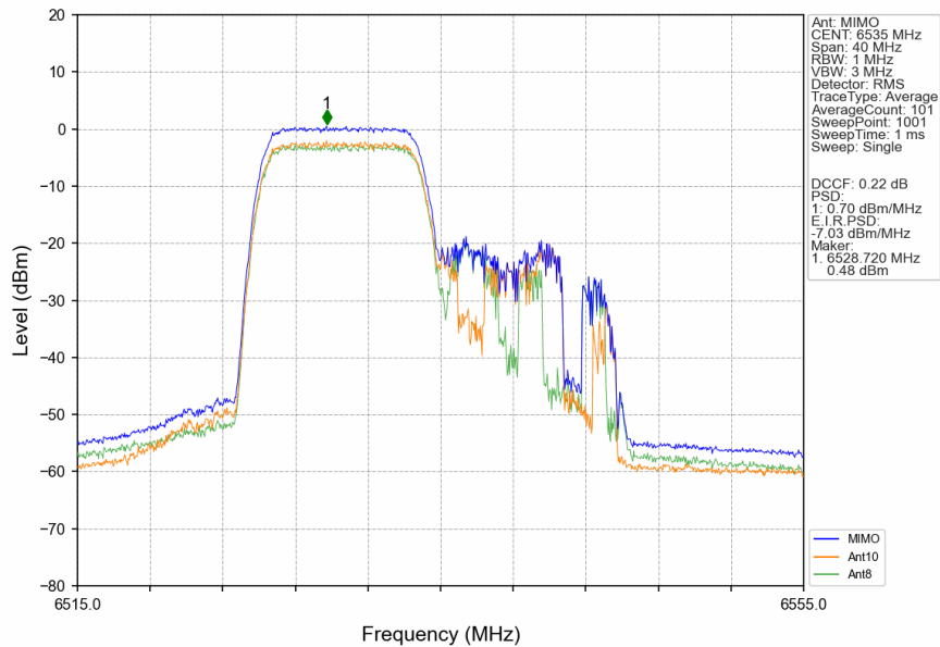
802.11ax(HEW20)_LCH_6535MHz_RU106_Left_MIMO_NTNV
