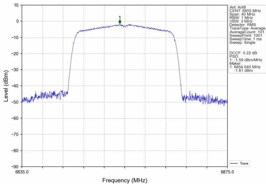
802.11ax(HEW20)_HCH_6855MHz_RU242_Left_Ant8_NTNV
