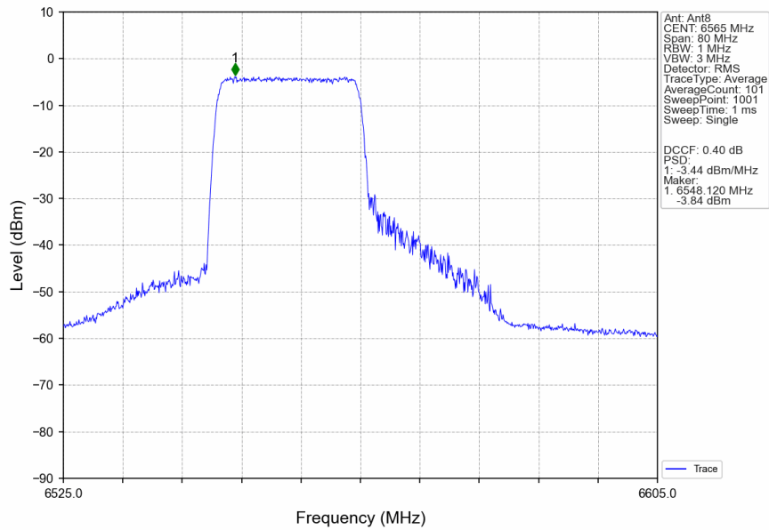
802.11ax(HEW40)_LCH_6565MHz_RU242_Left_MIMO_NTNV
