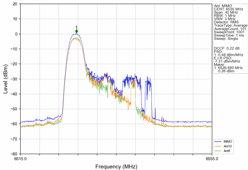
802.11ax(HEW20)_LCH_6535MHz_RU26_Left_MIMO_NTNV
