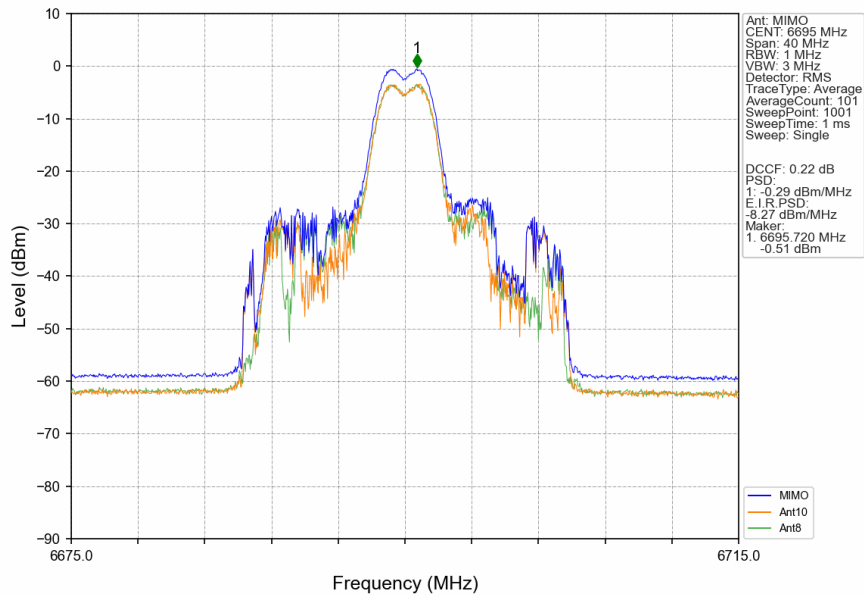
802.11ax(HEW20)_MCH_6695MHz_RU26_Mid_MIMO_NTNV
