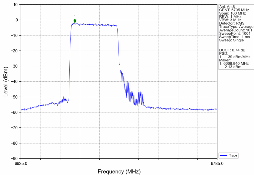
802.11ax(HEW80)_MCH_6705MHz_RU484_Left_MIMO_NTNV
