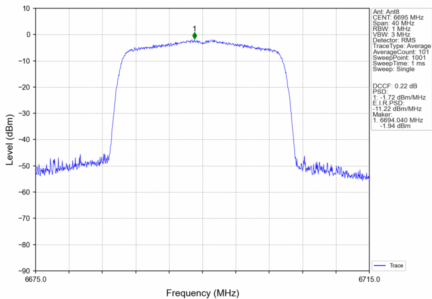
802.11ax(HEW20)_MCH_6695MHz_RU242_Left_Ant8_NTNV
