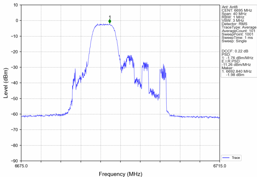
802.11ax(HEW20)_MCH_6695MHz_RU52_Mid_Ant8_NTNV
