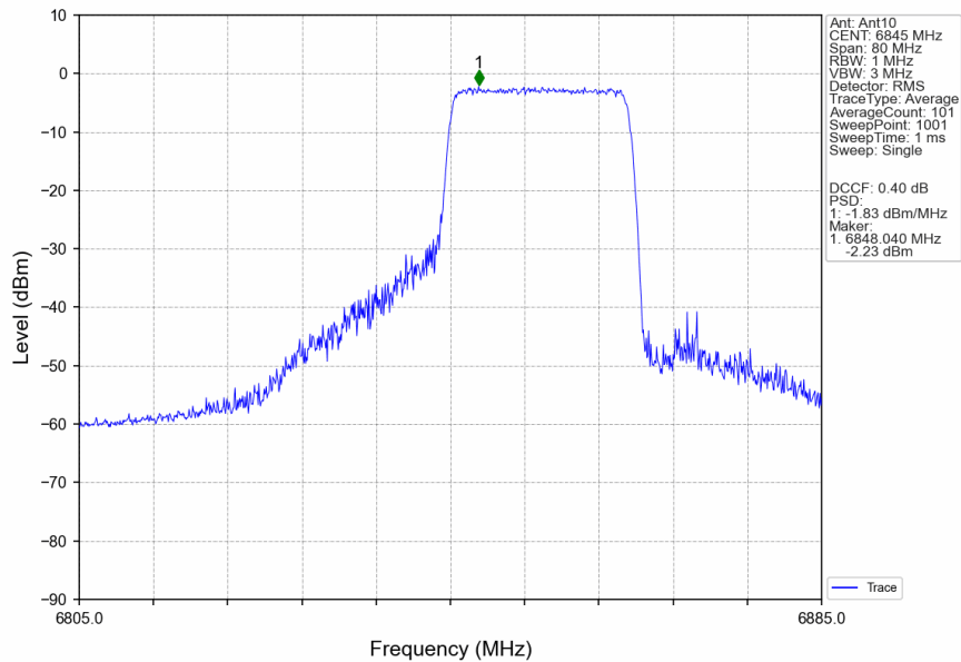
802.11ax(HEW40)_HCH_6845MHz_RU242_Right_Ant10_NTNV
