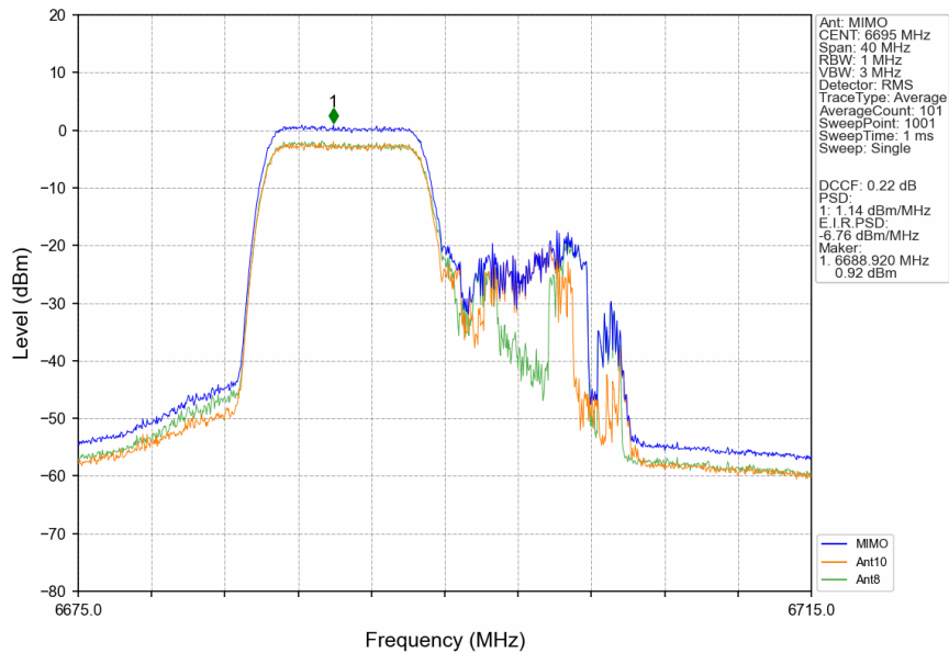
802.11ax(HEW20)_MCH_6695MHz_RU106_Left_MIMO_NTNV
