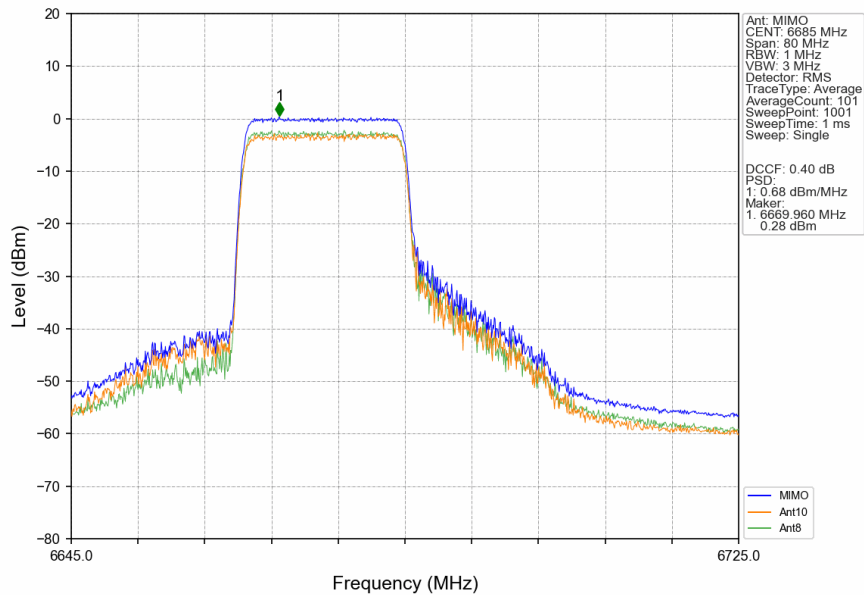
802.11ax(HEW40)_MCH_6685MHz_RU242_Left_MIMO_NTNV
