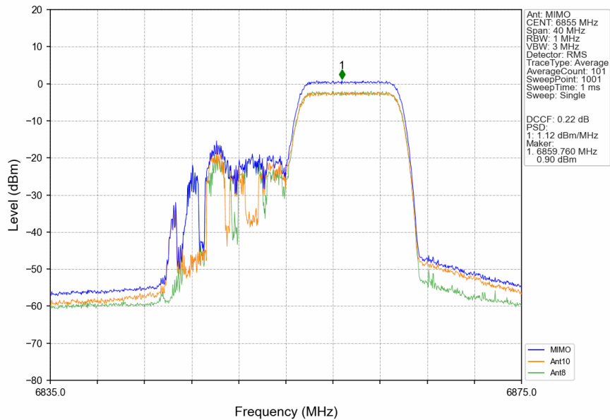
802.11ax(HEW20)_HCH_6855MHz_RU106_Right_MIMO_NTNV
