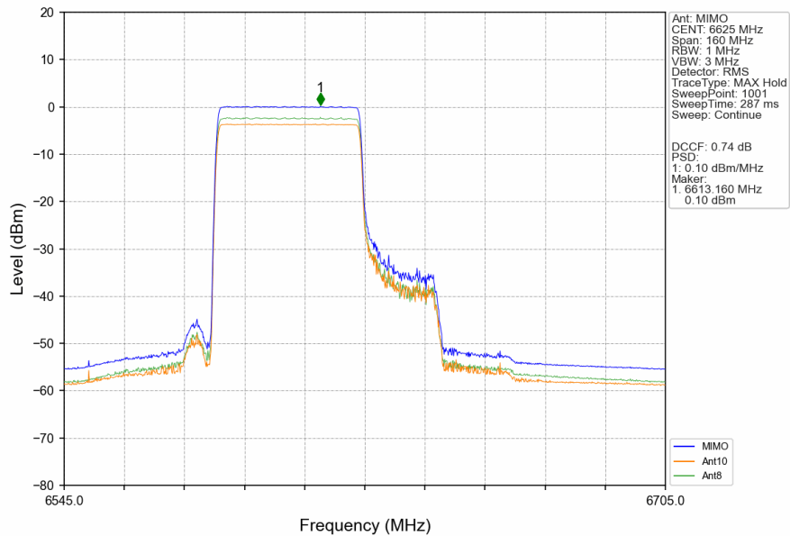
802.11ax(HEW80)_LCH_6625MHz_RU484_Left_MIMO_NTNV
