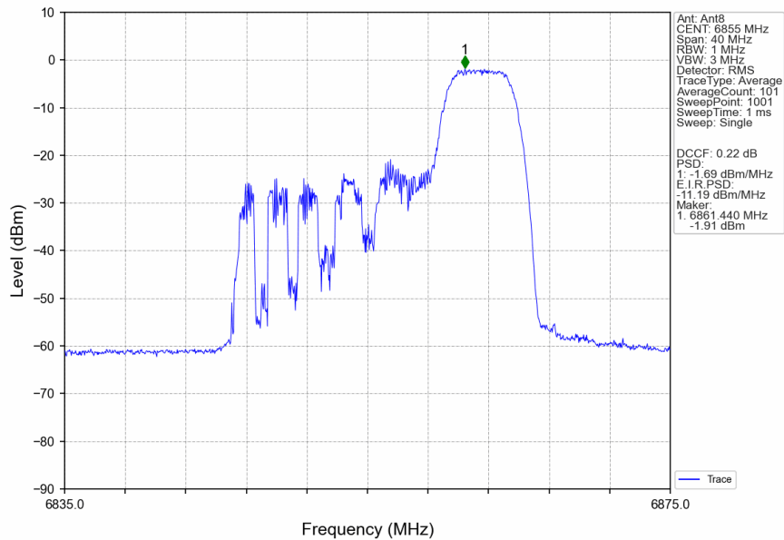
802.11ax(HEW20)_HCH_6855MHz_RU52_Right_Ant8_NTNV
