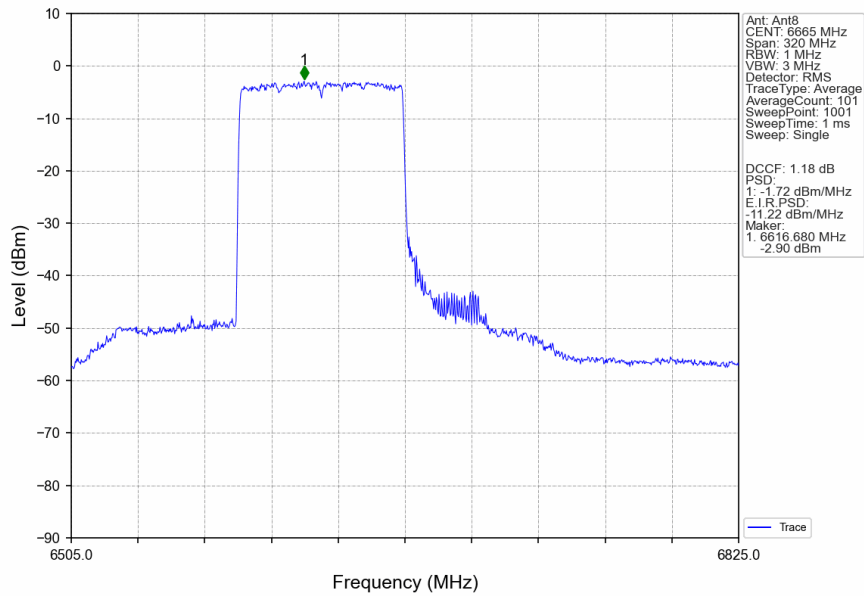
802.11ax(HEW160)_MCH_6665MHz_RU996_Left_MIMO_NTNV
