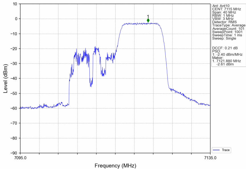
802.11ax(HEW20)_HCH_7115MHz_RU106_Right_Ant10_NTNV
