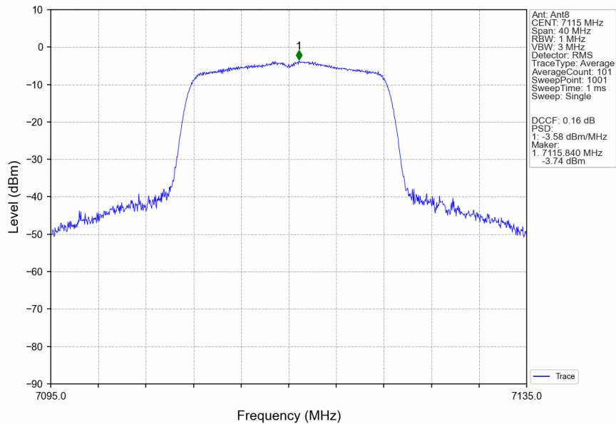
802.11a_HCH_7115MHz_Ant8_NTNV
