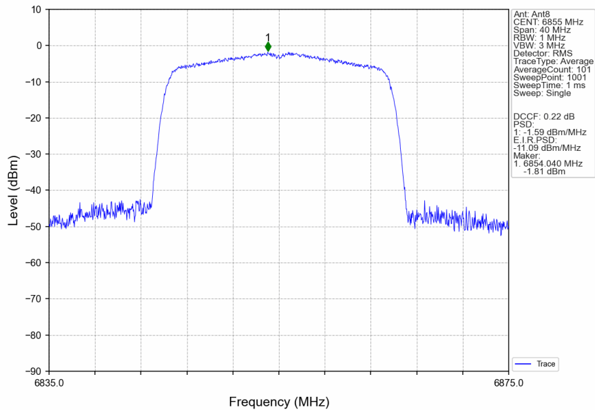
802.11ax(HEW20)_HCH_6855MHz_RU242_Left_Ant8_NTNV
