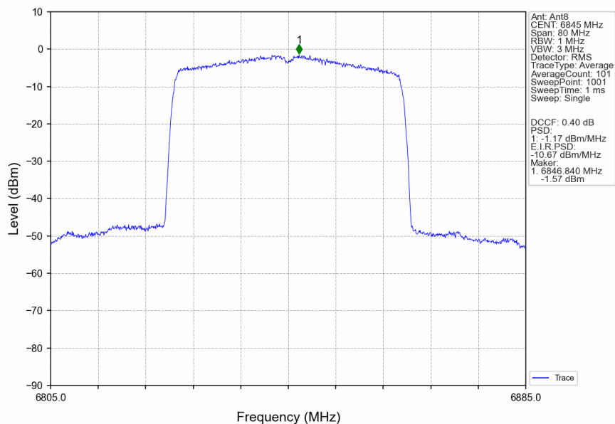
802.11ax(HEW40)_HCH_6845MHz_RU484_Left_Ant8_NTNV
