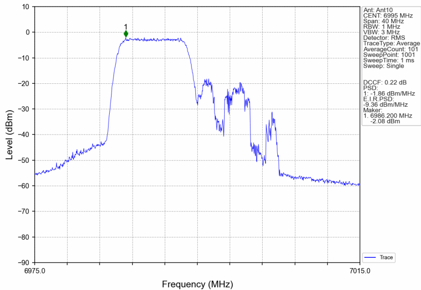
802.11ax(HEW20)_MCH_6995MHz_RU106_Left_Ant10_NTNV
