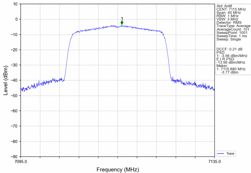
802.11ax(HEW20)_HCH_7115MHz_RU242_Left_Ant8_NTNV
