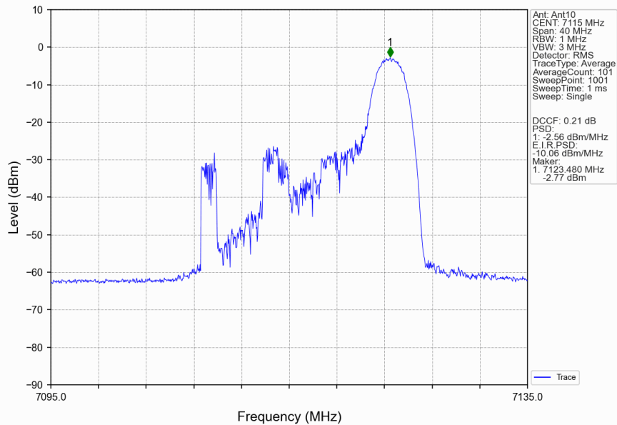
802.11ax(HEW20)_HCH_7115MHz_RU26_Right_Ant10_NTNV
