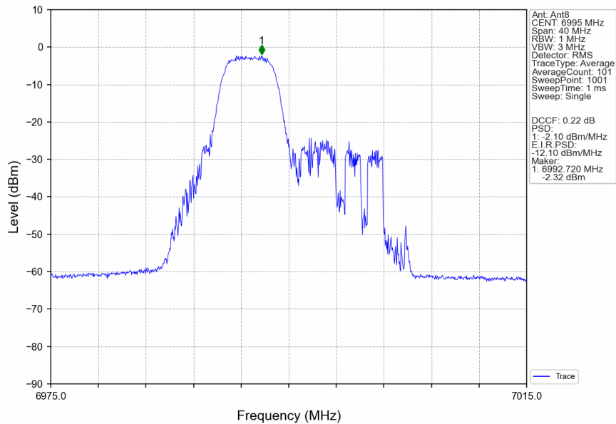
802.11ax(HEW20)_MCH_6995MHz_RU52_Mid_Ant8_NTNV
