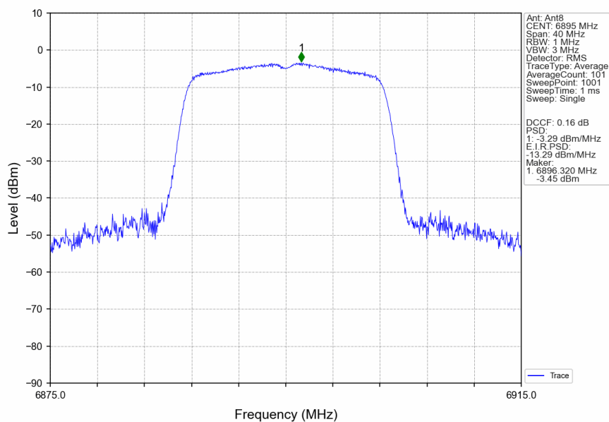
802.11a_LCH_6895MHz_Ant8_NTNV
