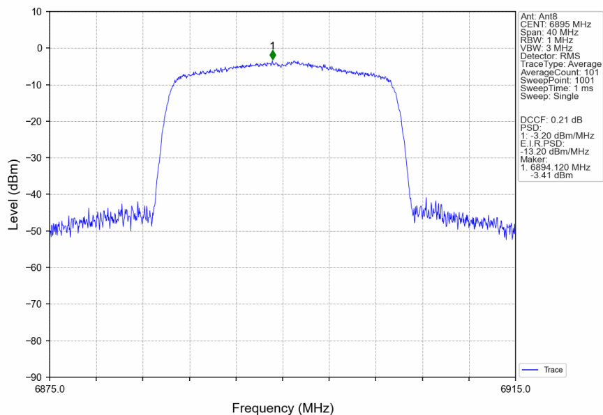
802.11ax(HEW20)_LCH_6895MHz_RU242_Left_Ant8_NTNV
