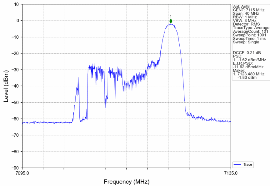
802.11ax(HEW20)_HCH_7115MHz_RU26_Right_MIMO_NTNV
