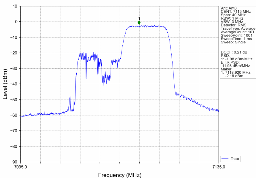
802.11ax(HEW20)_HCH_7115MHz_RU106_Right_MIMO_NTNV
