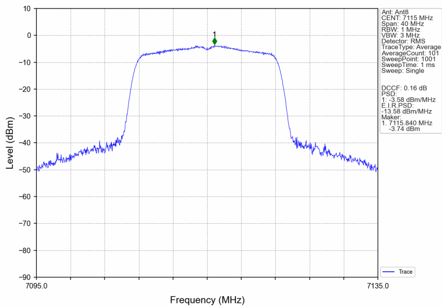
802.11a_HCH_7115MHz_Ant8_NTNV
