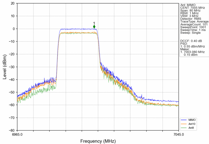
802.11ax(HEW40)_MCH_7005MHz_RU242_Left_MIMO_NTNV
