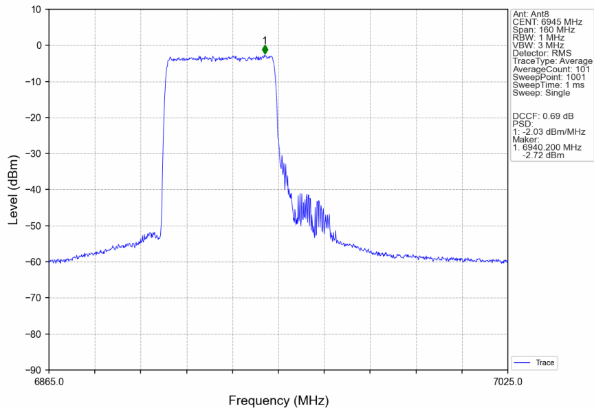
802.11ax(HEW80)_LCH_6945MHz_RU484_Left_MIMO_NTNV
