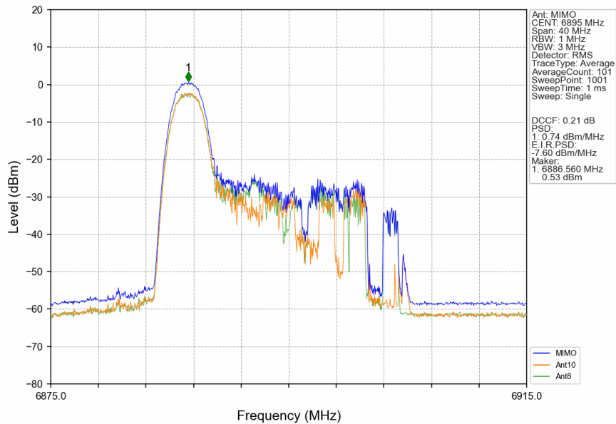
802.11ax(HEW20)_LCH_6895MHz_RU26_Left_MIMO_NTNV
