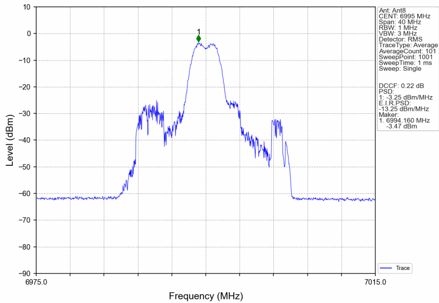
802.11ax(HEW20)_MCH_6995MHz_RU26_Mid_MIMO_NTNV
