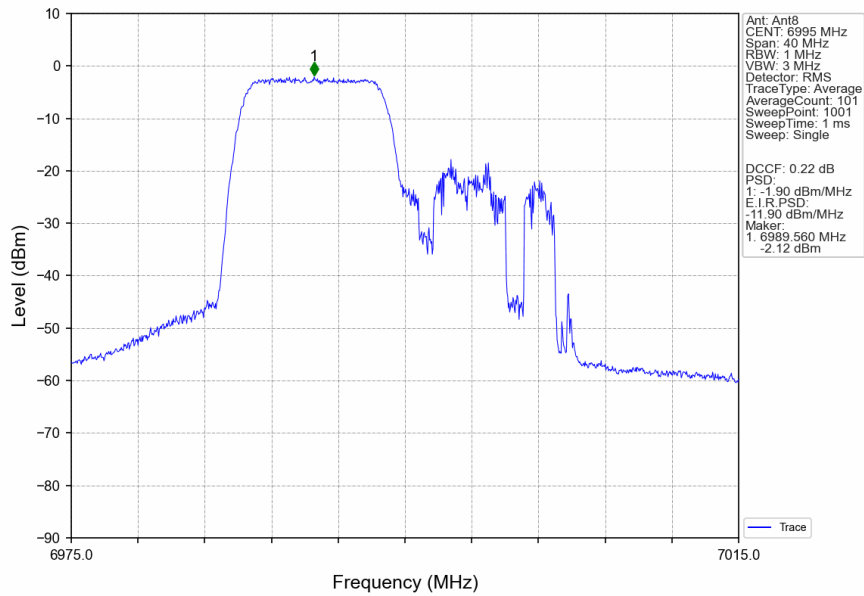
802.11ax(HEW20)_MCH_6995MHz_RU106_Left_MIMO_NTNV
