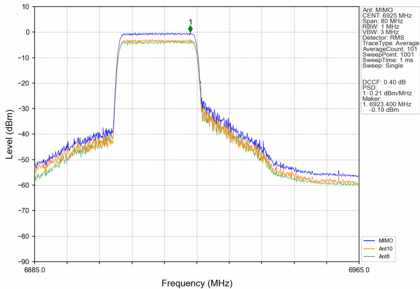
802.11ax(HEW40)_LCH_6925MHz_RU242_Left_MIMO_NTNV
