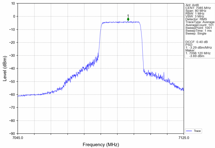
802.11ax(HEW40)_HCH_7085MHz_RU242_Right_MIMO_NTNV
