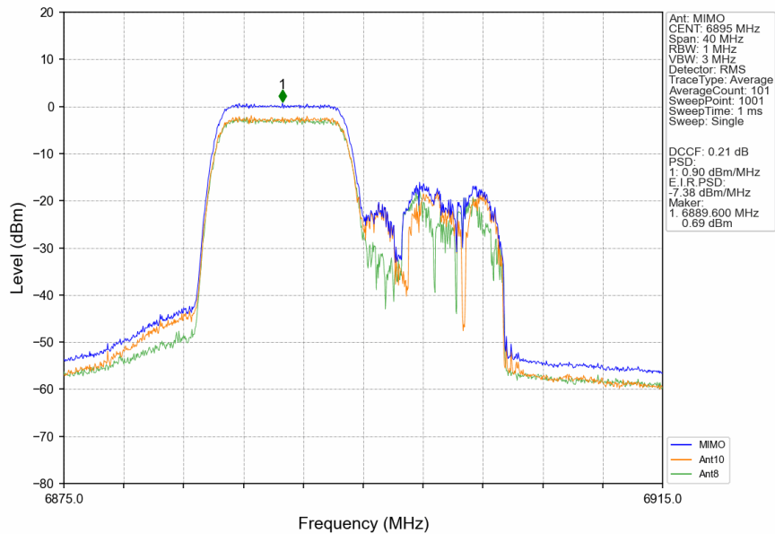
802.11ax(HEW20)_LCH_6895MHz_RU106_Left_MIMO_NTNV
