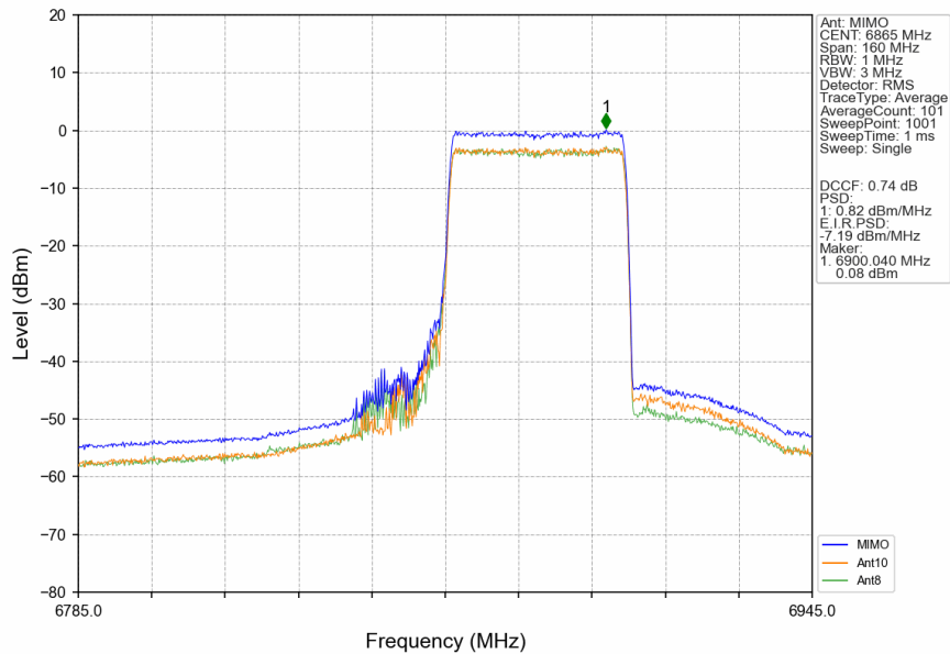
802.11ax(HEW80)_HCH_6865MHz_RU484_Right_MIMO_NTNV
