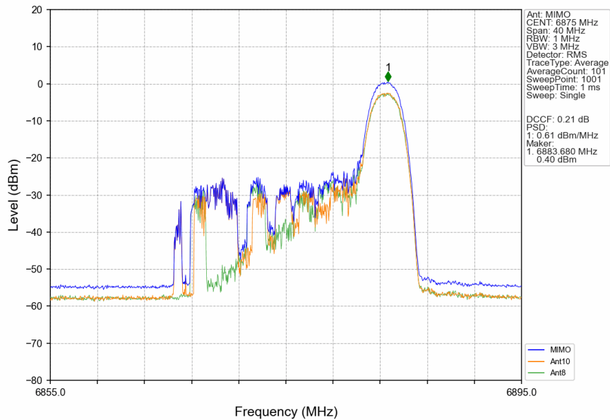
802.11ax(HEW20)_HCH_6875MHz_RU26_Right_MIMO_NTNV
