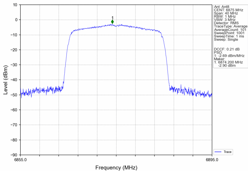
802.11ax(HEW20)_HCH_6875MHz_RU242_Left_Ant8_NTNV
