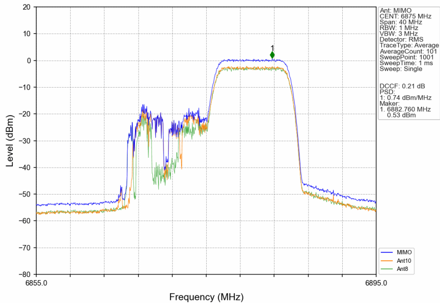
802.11ax(HEW20)_HCH_6875MHz_RU106_Right_MIMO_NTNV
