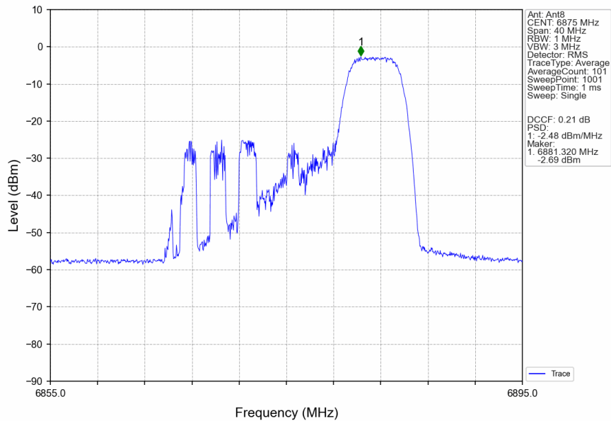
802.11ax(HEW20)_HCH_6875MHz_RU52_Right_Ant8_NTNV
