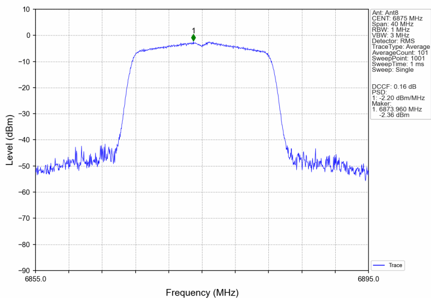
802.11a_HCH_6875MHz_Ant8_NTNV
