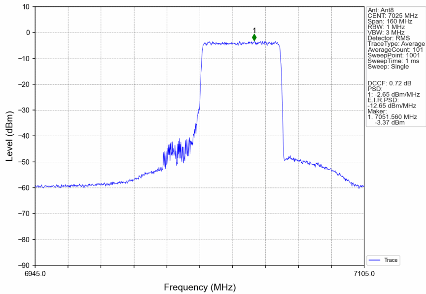
802.11ax(HEW80)_HCH_7025MHz_RU484_Right_MIMO_NTNV
