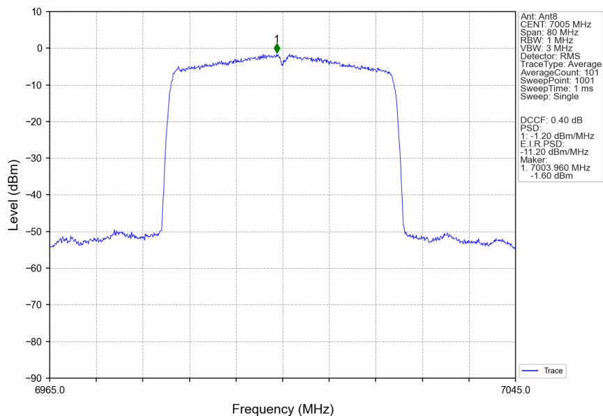
802.11ax(HEW40)_MCH_7005MHz_RU484_Left_Ant8_NTNV
