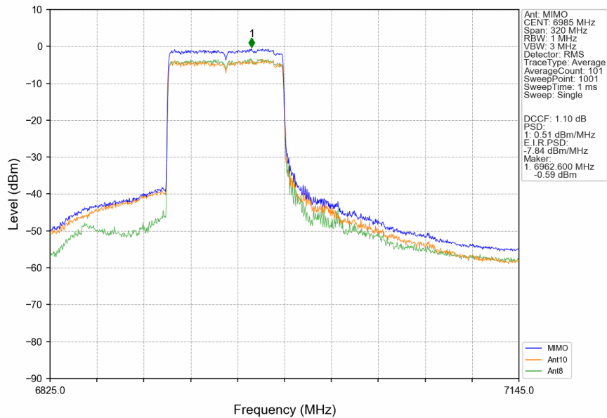
802.11ax(HEW160)_MCH_6985MHz_RU996_Left_MIMO_NTNV
