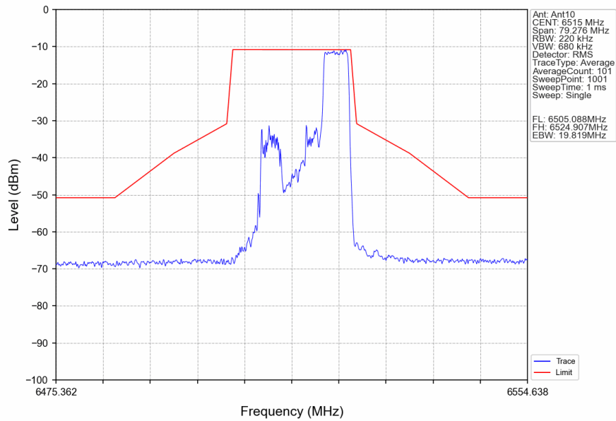
802.11ax(HEW20)_HCH_6515MHz_RU106_Right_Ant10_NTNV
