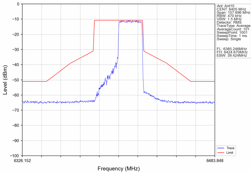
802.11ax(HEW40)_HCH_6405MHz_RU242_Right_Ant10_NTNV
