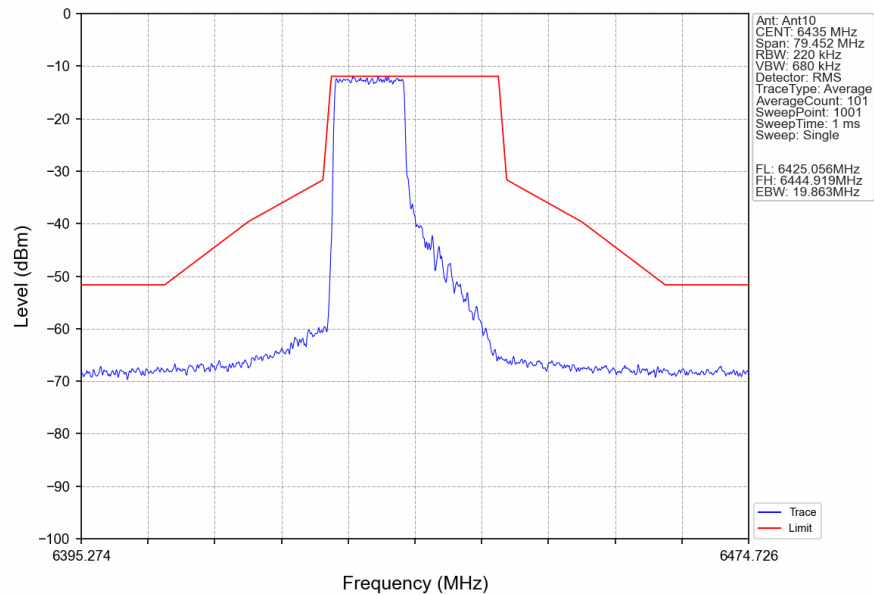
802.11ax(HEW20)_LCH_6435MHz_RU106_Left_Ant10_NTNV
