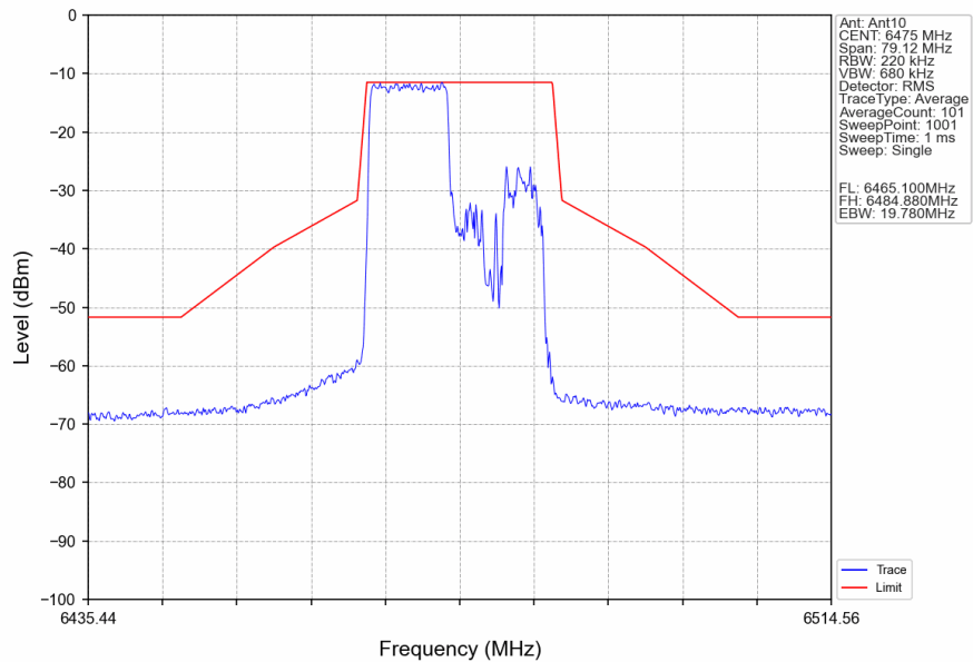
802.11ax(HEW20)_MCH_6475MHz_RU106_Left_Ant10_NTNV
