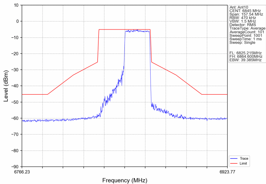
802.11ax(HEW40)_HCH_6845MHz_RU242_Right_Ant10_NTNV
