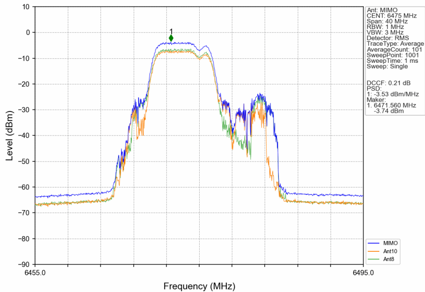
802.11be(EHT20)_MCH_6475MHz_26+52_/_MIMO_NTNV
