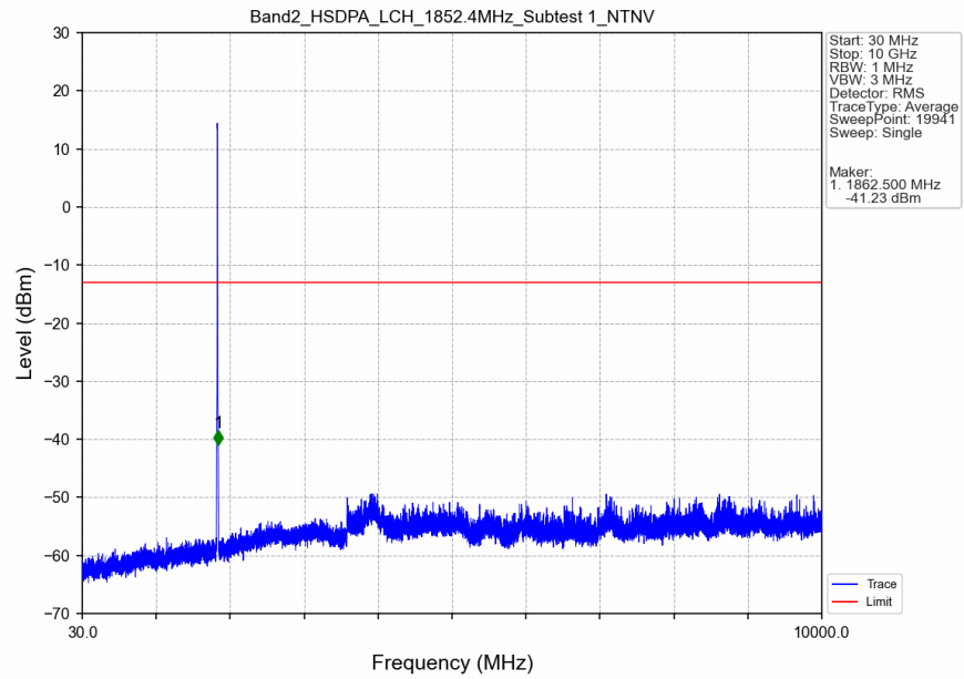
Band2_HSDPA_LCH_1852.4MHz_Subtest 1_NTNV
