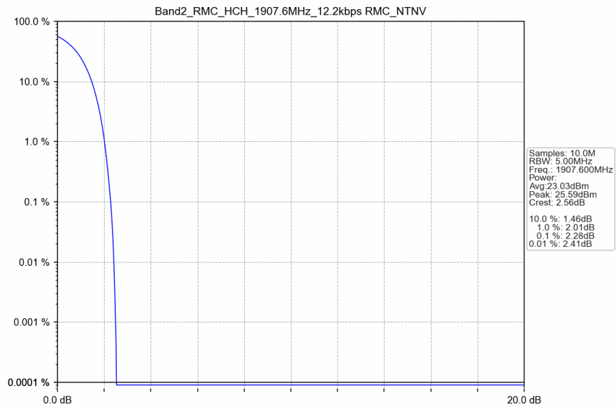
Band2_RMC_HCH_1907.6MHz_12.2kbps RMC_NTNV
