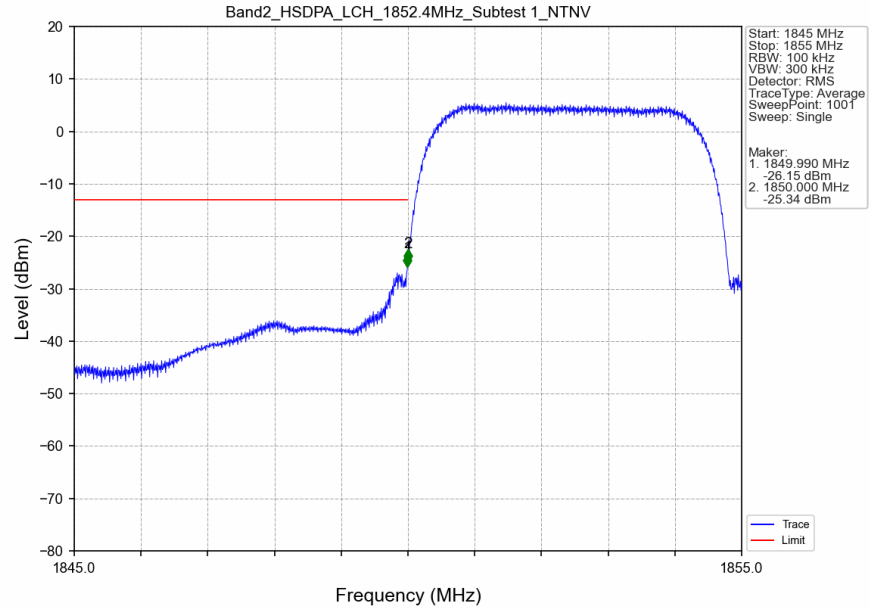
Band2_HSDPA_LCH_1852.4MHz_Subtest 1_NTNV
