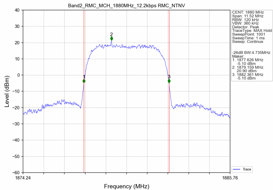
Band2_RMC_MCH_1880MHz_12.2kbps RMC_NTNV
