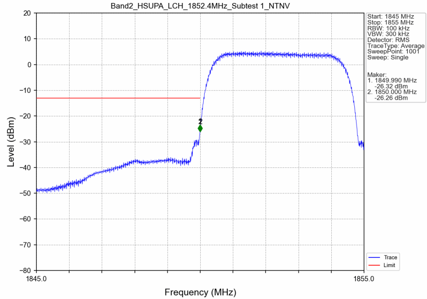
Band2_HSUPA_LCH_1852.4MHz_Subtest 1_NTNV
