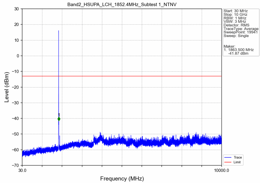
Band2_HSUPA_LCH_1852.4MHz_Subtest 1_NTNV
