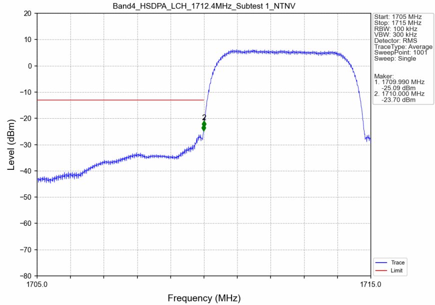
Band4_HSDPA_LCH_1712.4MHz_Subtest 1_NTNV
