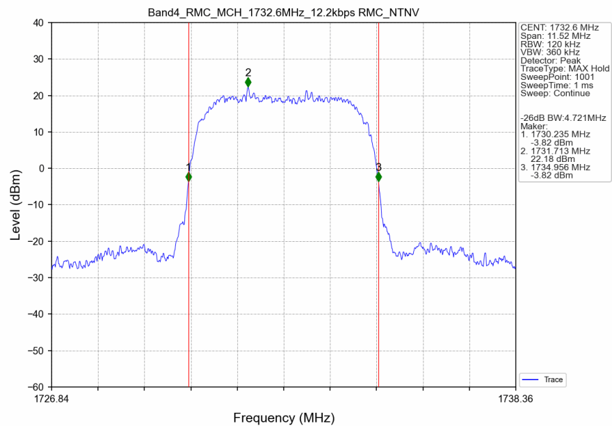
Band4_RMC_MCH_1732.6MHz_12.2kbps RMC_NTNV
