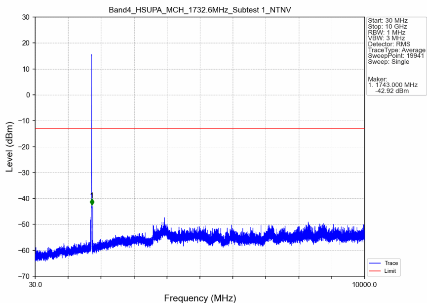
Band4_HSUPA_MCH_1732.6MHz_Subtest 1_NTNV
