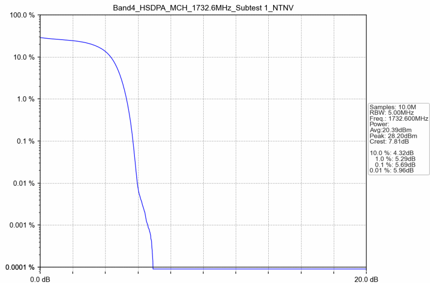
Band4_HSDPA_MCH_1732.6MHz_Subtest 1_NTNV
