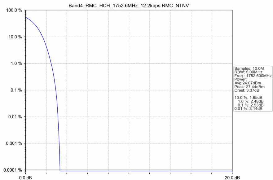
Band4_RMC_HCH_1752.6MHz_12.2kbps RMC_NTNV
