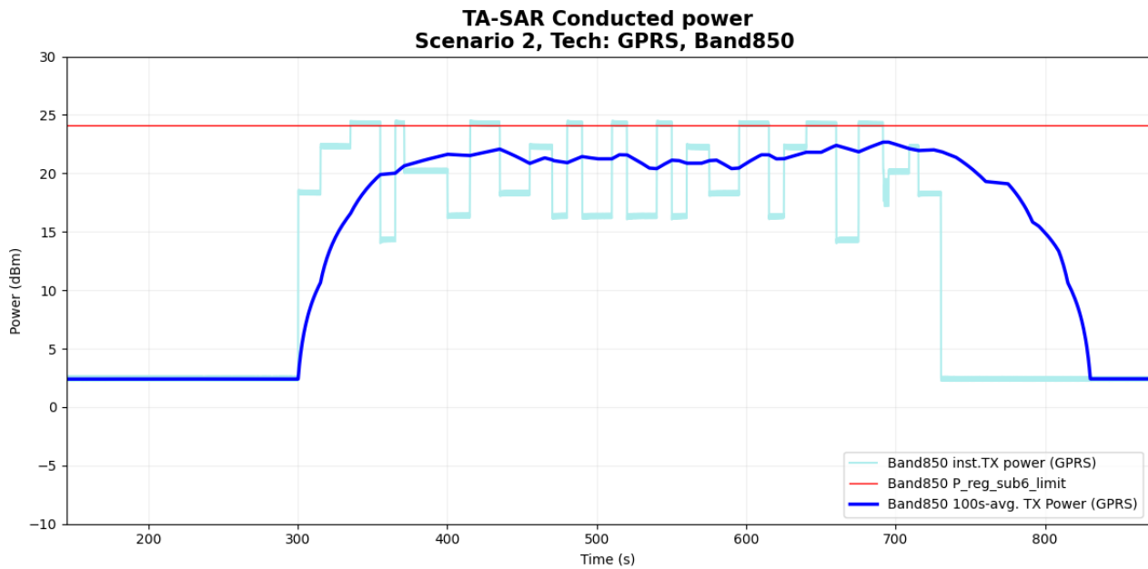
Figure 6- 9 Time-averaged conducted TX power over time
