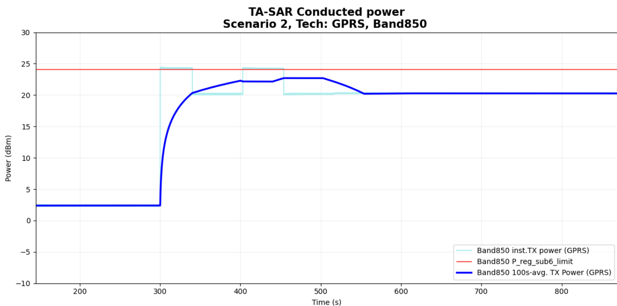
Figure 6- 7 Time-averaged conducted TX power over time
