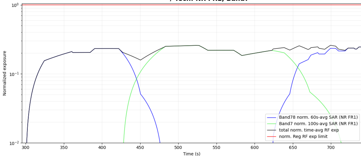
Figure 6- 46 Normalized time-averaged SAR
