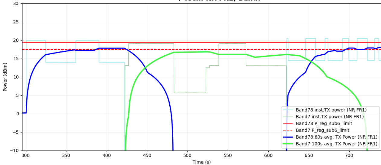
Figure 6- 45 Time-averaged conducted TX power over time
