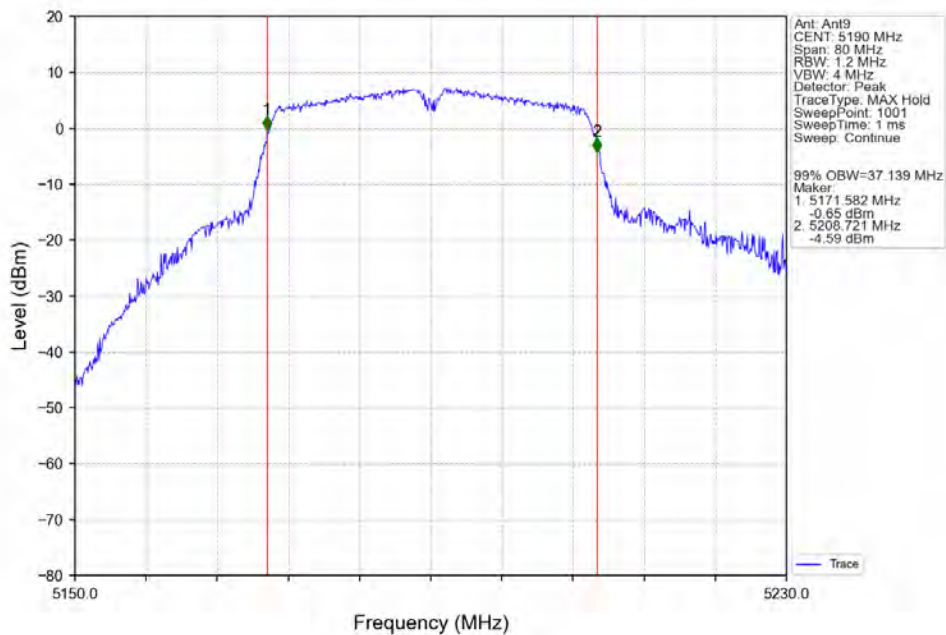
802.11ac(VHT40)_LCH_5190MHz_Ant9_NTNV
