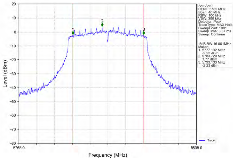
802.11ac(VHT20)_MCH_5785MHz_Ant9_NTNV
