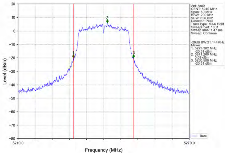
802.11ac(VHT20)_HCH_5240MHz_Ant9_NTNV
