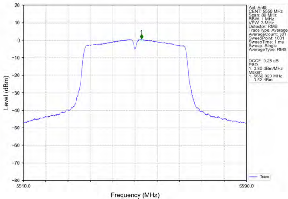
802.11ac(VHT40)_MCH_5550MHz_Ant9_NTNV
