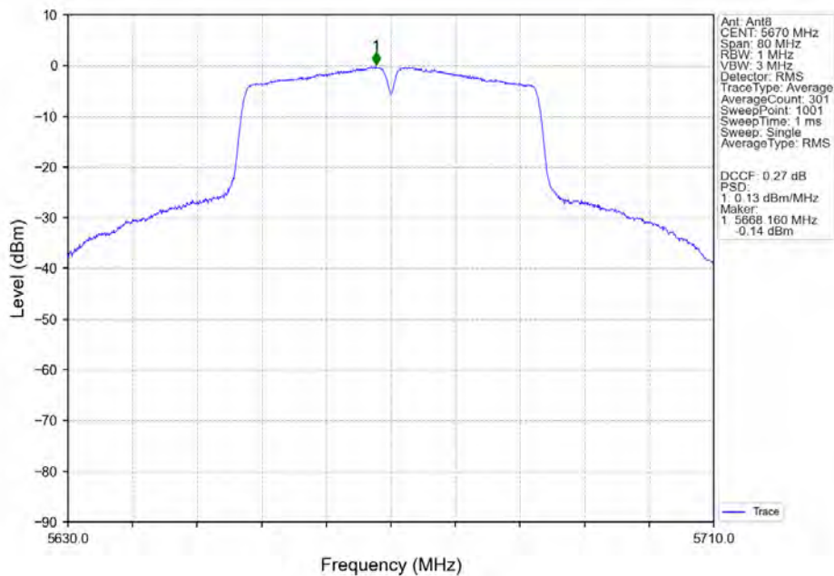
802.11ac(VHT40)_HCH_5670MHz_Ant8_NTNV
