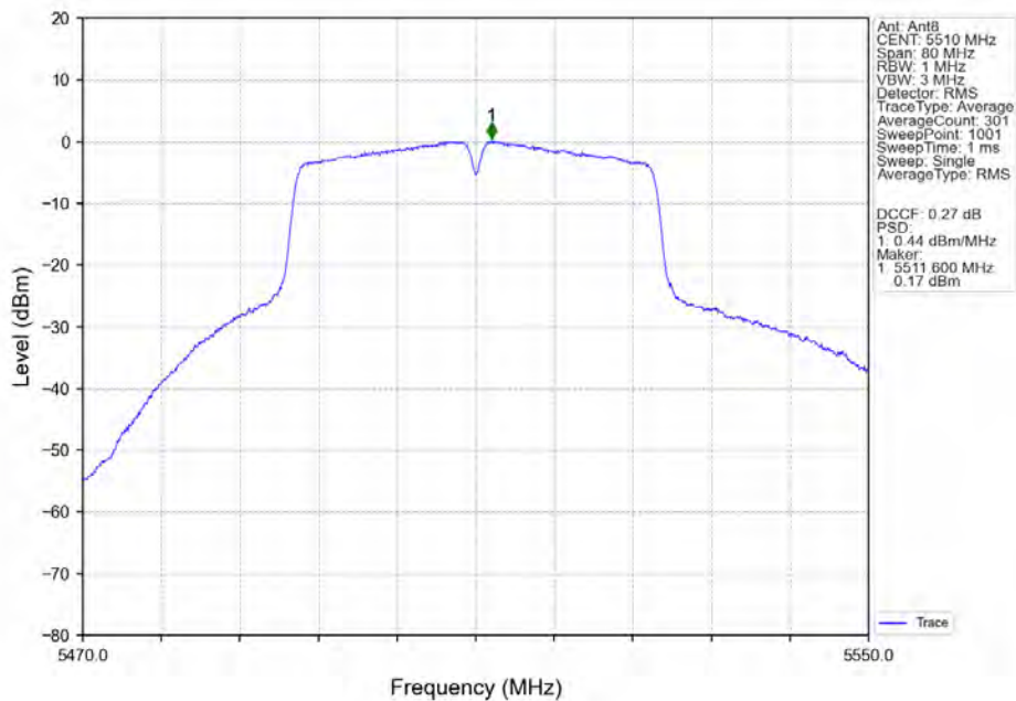
802.11ac(VHT40)_LCH_5510MHz_Ant8_NTNV
