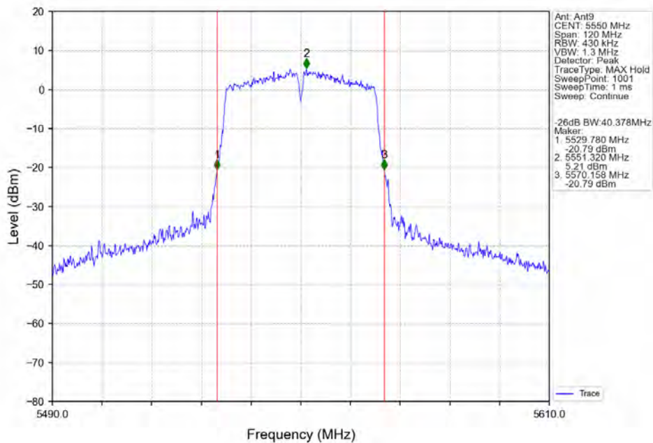
802.11ac(VHT40)_MCH_5550MHz_Ant9_NTNV
