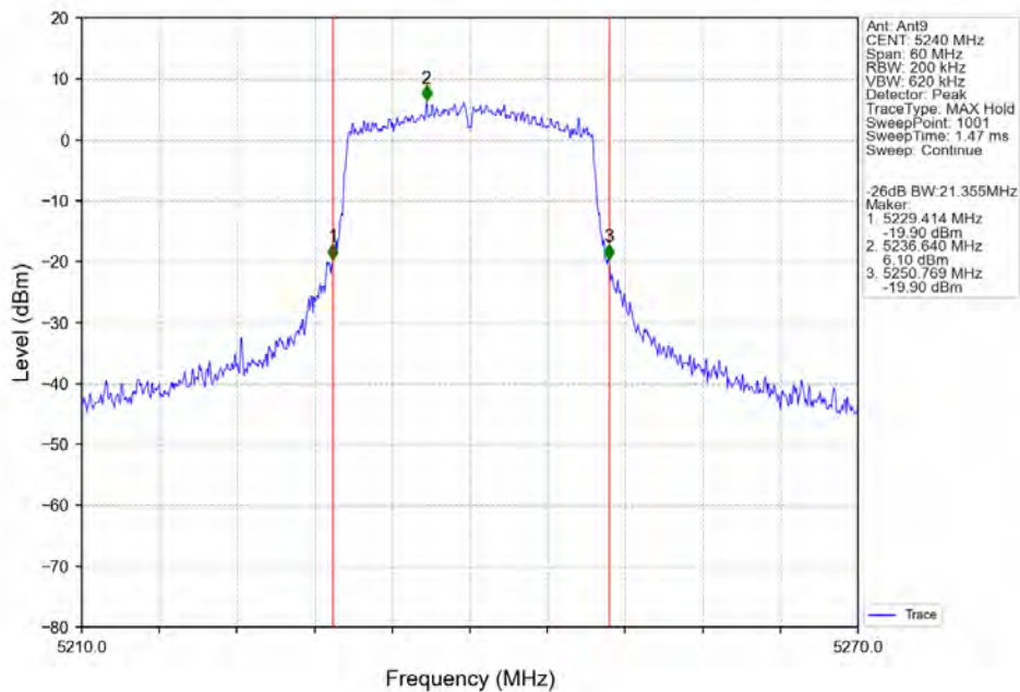
802.11ax(HEW20)_HCH_5240MHz_RU242_Left_Ant9_NTNV
