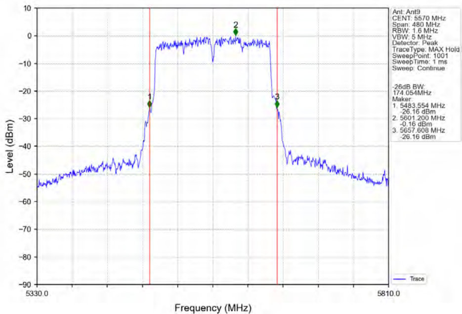
802.11ac(VHT160)_MCH_5570MHz_Ant9_NTNV
