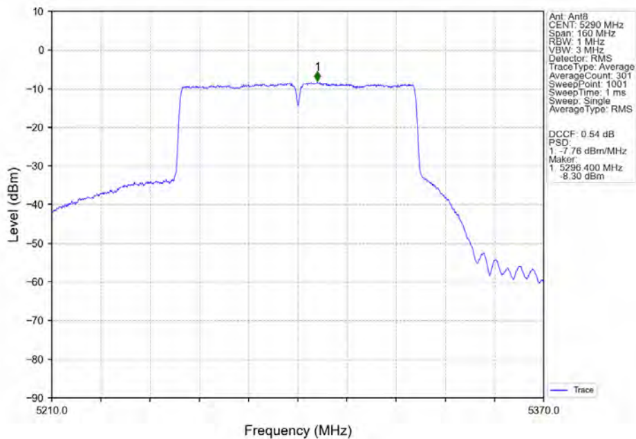
802.11ac(VHT80)_MCH_5290MHz_Ant8_NTNV
