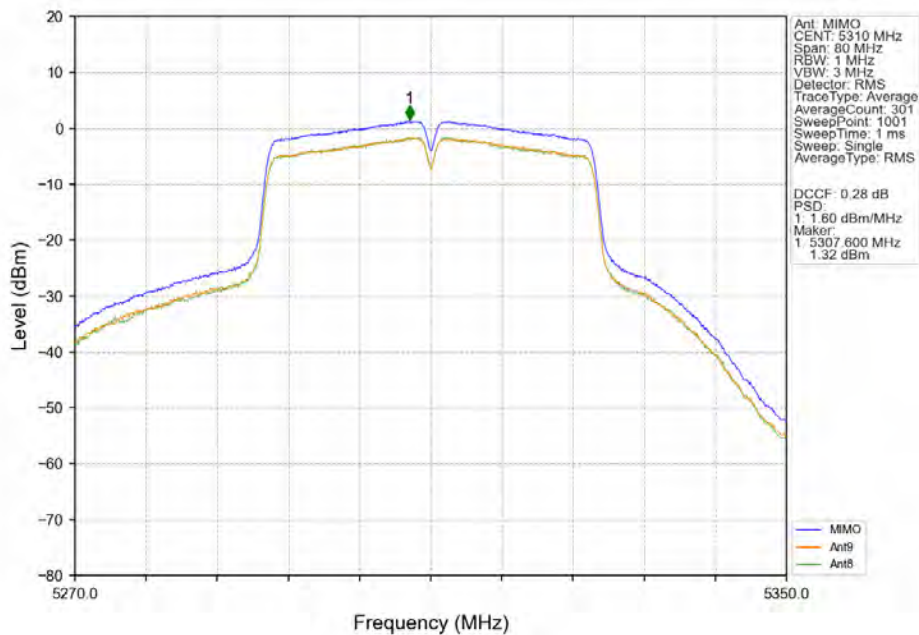
802.11ac(VHT40)_HCH_5310MHz_MIMO_NTNV
