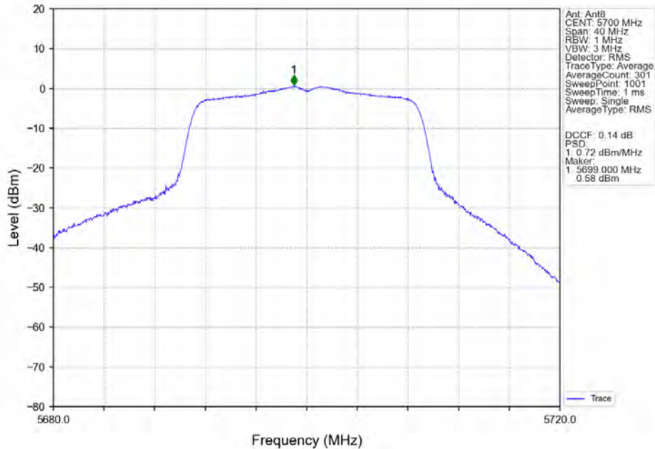
802.11n(HT20)_HCH_5700MHz_MIMO_NTNV
