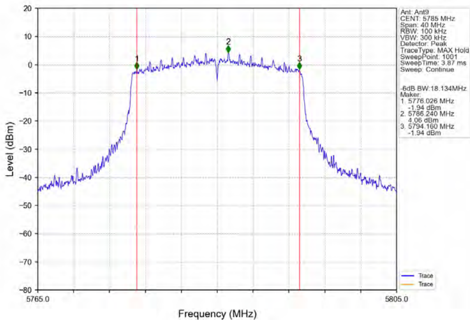
802.11ax(HEW20)_MCH_5785MHz_RU242_Left_Ant9_NTNV
