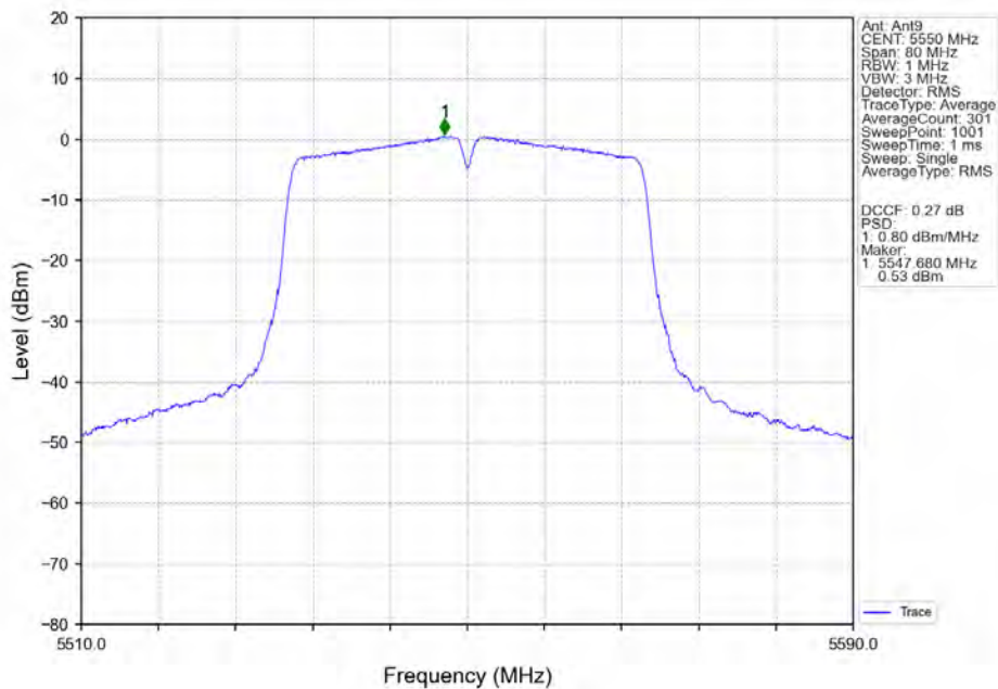
802.11n(HT40)_MCH_5550MHz_Ant9_NTNV
