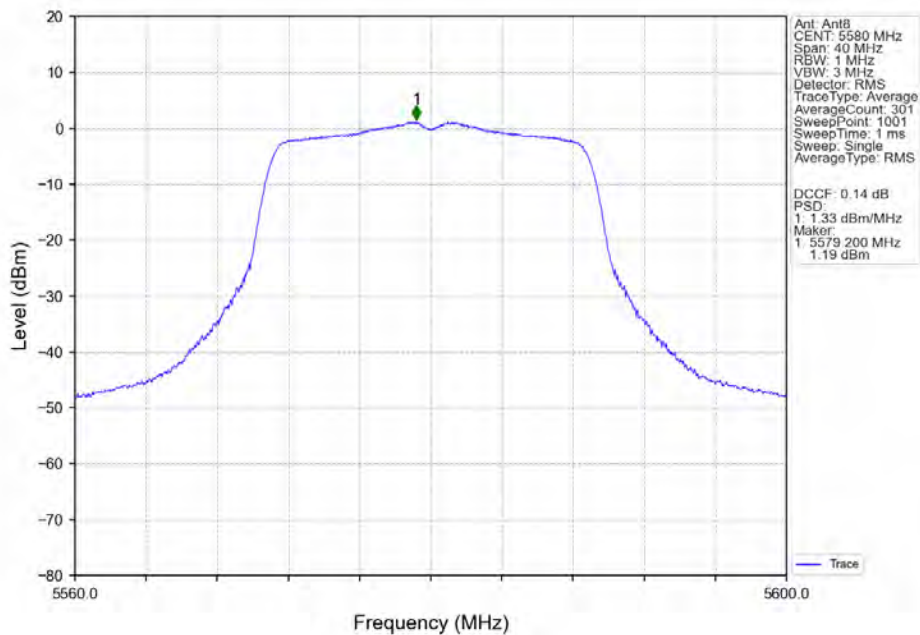
802.11ac(VHT20)_MCH_5580MHz_Ant8_NTNV
