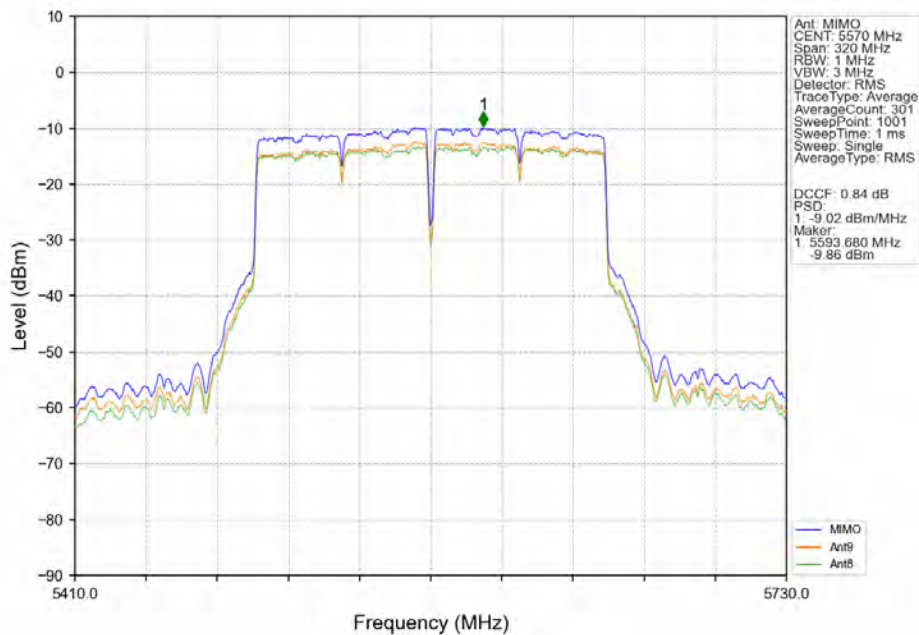
802.11ac(VHT160)_MCH_5570MHz_MIMO_NTNV
