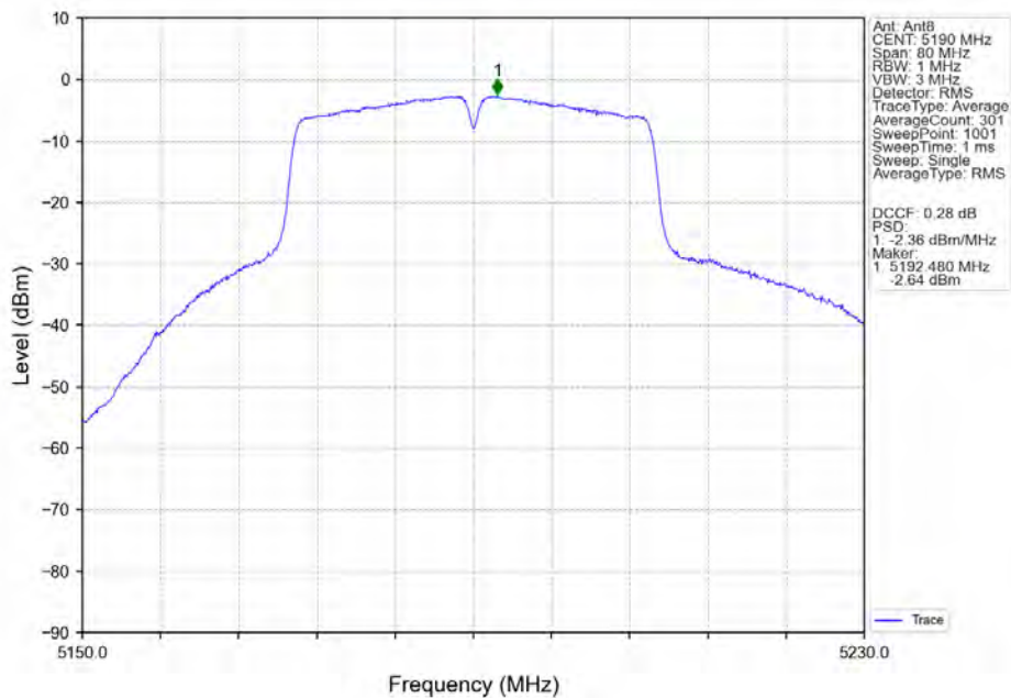
802.11ac(VHT40)_LCH_5190MHz_Ant8_NTNV
