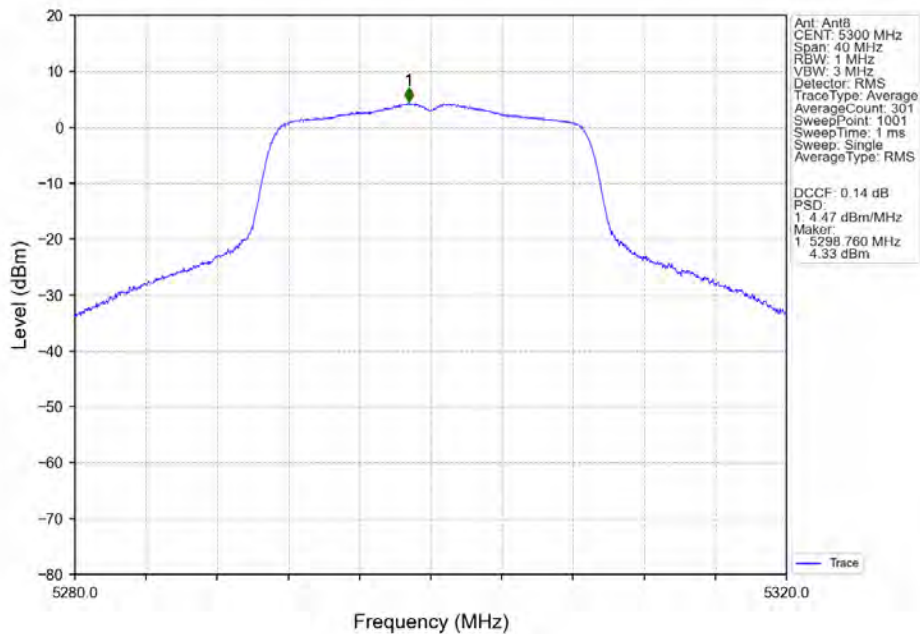
802.11ac(VHT20)_MCH_5300MHz_MIMO_NTNV
