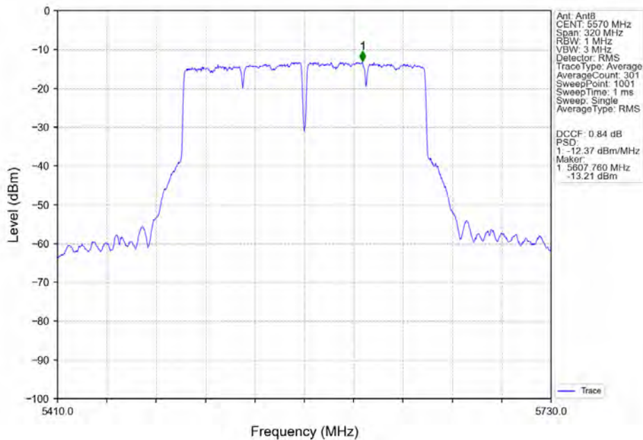
802.11ac(VHT160)_MCH_5570MHz_MIMO_NTNV
