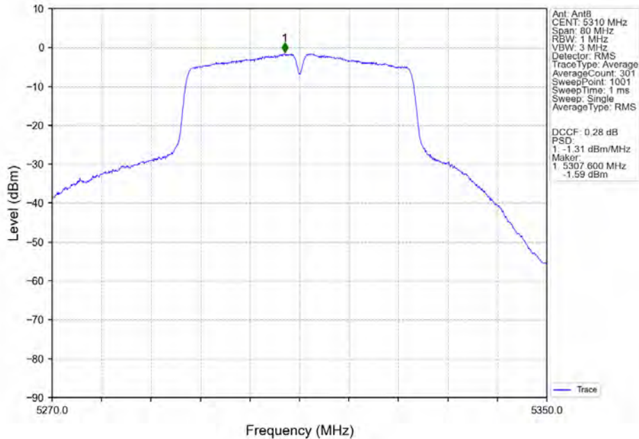
802.11ac(VHT40)_HCH_5310MHz_MIMO_NTNV
