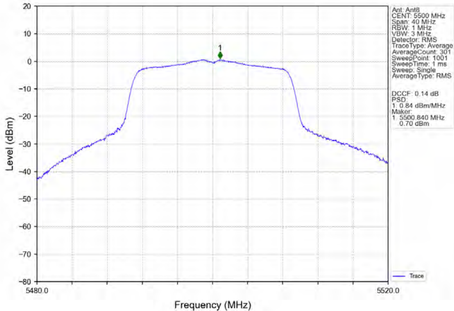
802.11ac(VHT20)_LCH_5500MHz_MIMO_NTNV
