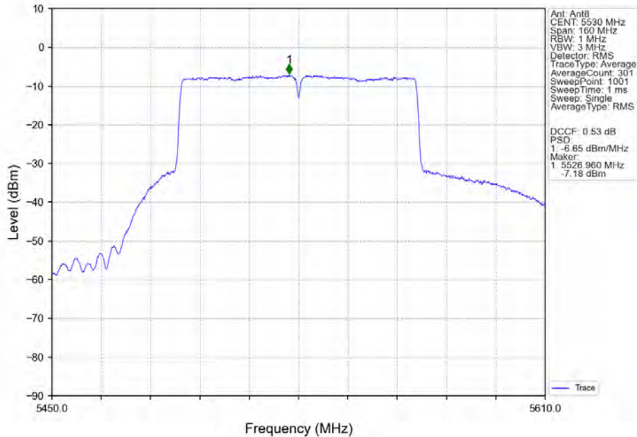
802.11ac(VHT80)_LCH_5530MHz_MIMO_NTNV
