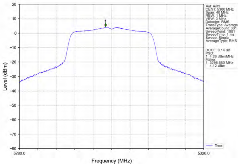
802.11ac(VHT20)_MCH_5300MHz_Ant9_NTNV
