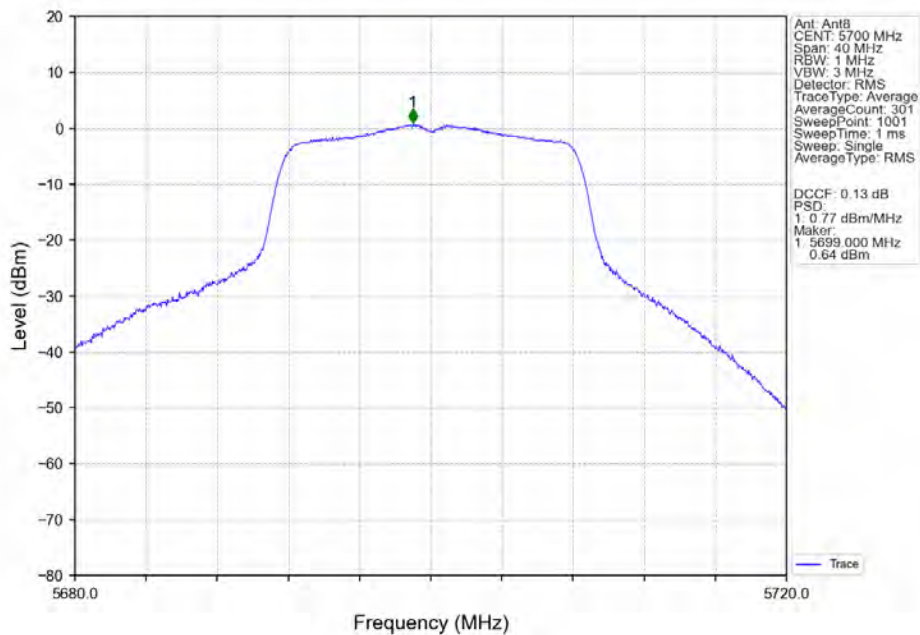
802.11a_HCH_5700MHz_Ant8_NTNV
