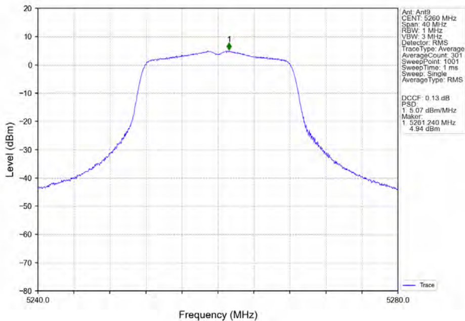
802.11a_LCH_5260MHz_Ant9_NTNV
