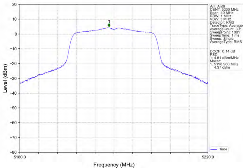
802.11ac(VHT20)_MCH_5200MHz_Ant8_NTNV
