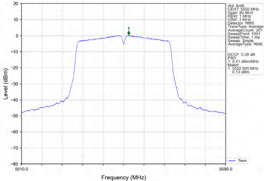
802.11ac(VHT40)_MCH_5550MHz_MIMO_NTNV
