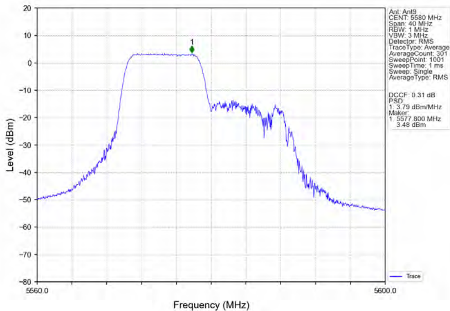
802.11ax(HEW20)_MCH_5580MHz_RU106_Left_Ant9_NTNV
