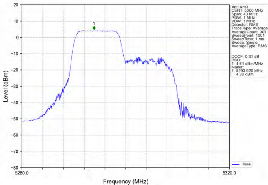
802.11ax(HEW20)_MCH_5300MHz_RU106_Left_Ant9_NTNV
