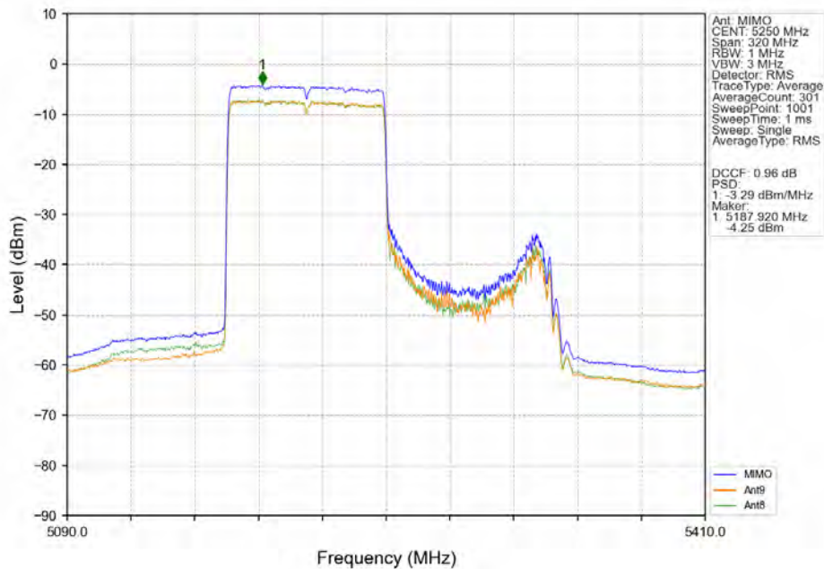
802.11ax(HEW160)_MCH_5250MHz_RU996_Right_Ant9_NTNV
