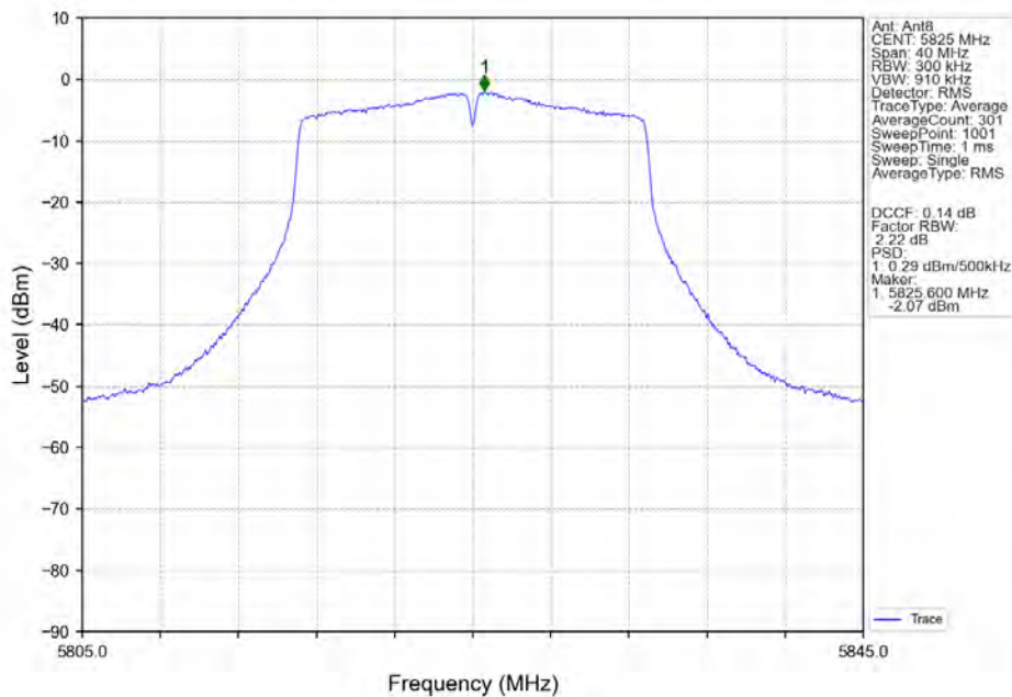
802.11ac(VHT20)_HCH_5825MHz_Ant8_NTNV
