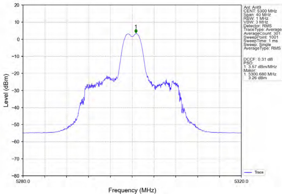
802.11ax(HEW20)_MCH_5300MHz_RU26_Mid_Ant9_NTNV
