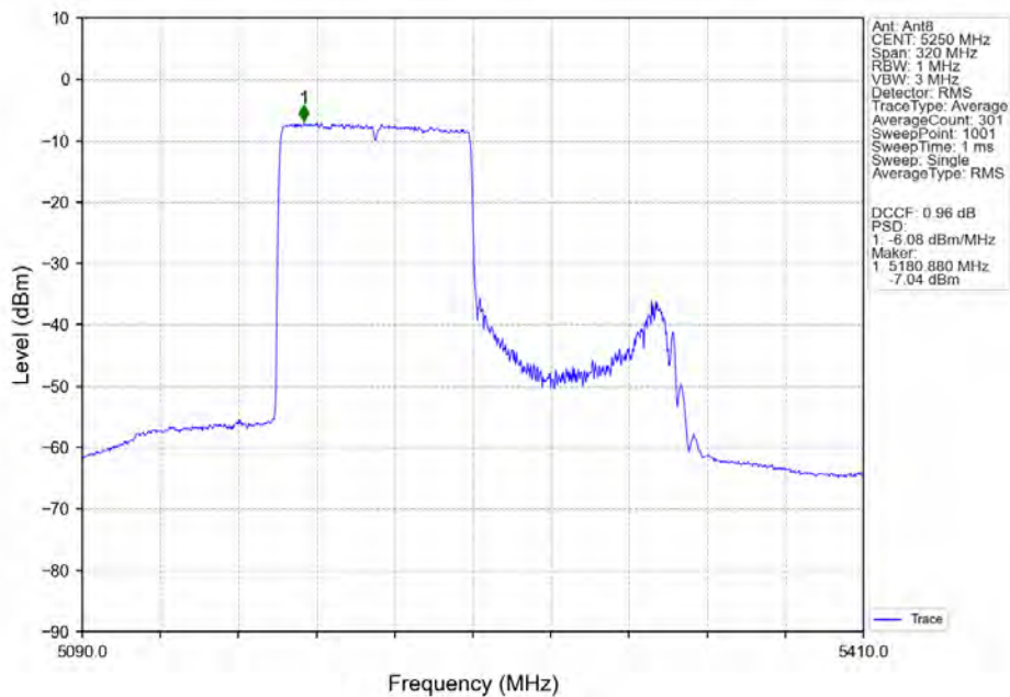
802.11ax(HEW160)_MCH_5250MHz_RU996_Left_Ant8_NTNV
