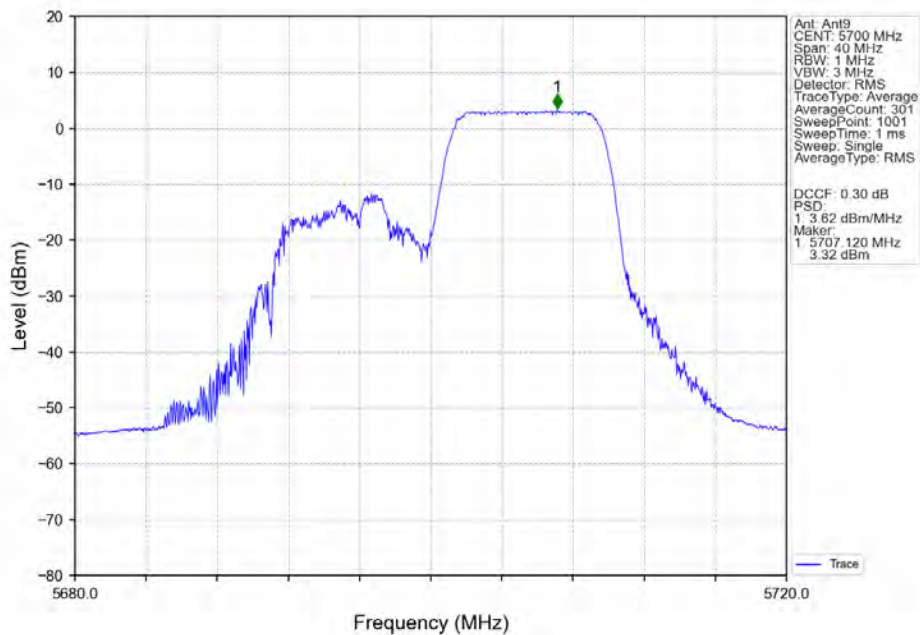
802.11ax(HEW20)_HCH_5700MHz_RU106_Right_Ant9_NTNV
