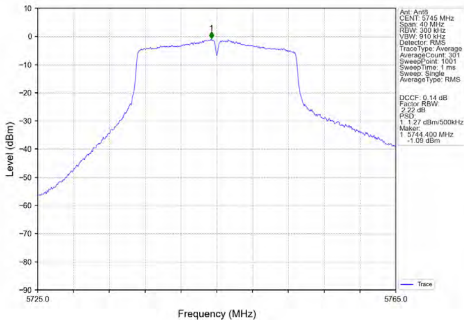
802.11ac(VHT20)_LCH_5745MHz_Ant8_NTNV
