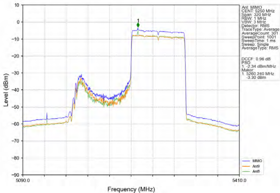
802.11ax(HEW160)_MCH_5250MHz_RU996_Right_MIMO_NTNV
