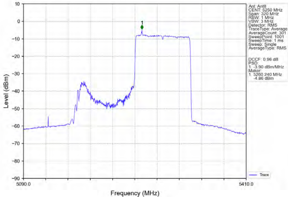
802.11ax(HEW160)_MCH_5250MHz_RU996_Right_MIMO_NTNV
