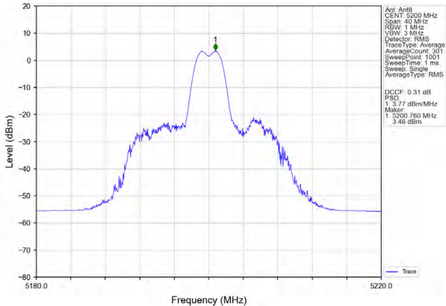
802.11ax(HEW20)_MCH_5200MHz_RU26_Mid_MIMO_NTNV
