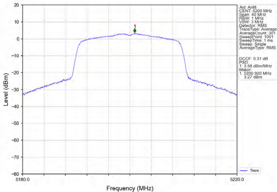
802.11ax(HEW20)_MCH_5200MHz_RU242_Left_Ant8_NTNV
