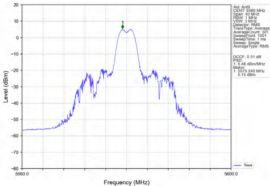
802.11ax(HEW20)_MCH_5580MHz_RU26_Mid_Ant9_NTNV
