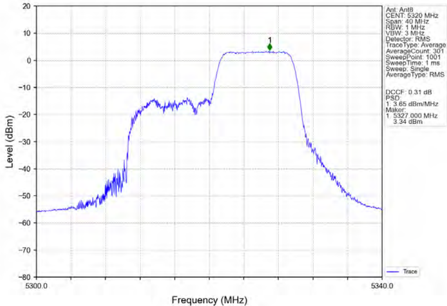
802.11ax(HEW20)_HCH_5320MHz_RU106_Right_MIMO_NTNV
