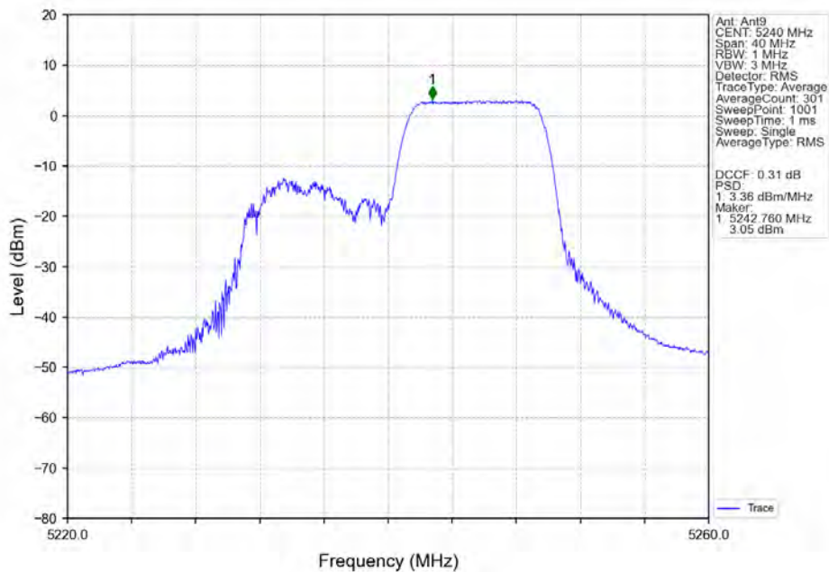
802.11ax(HEW20)_HCH_5240MHz_RU106_Right_Ant9_NTNV
