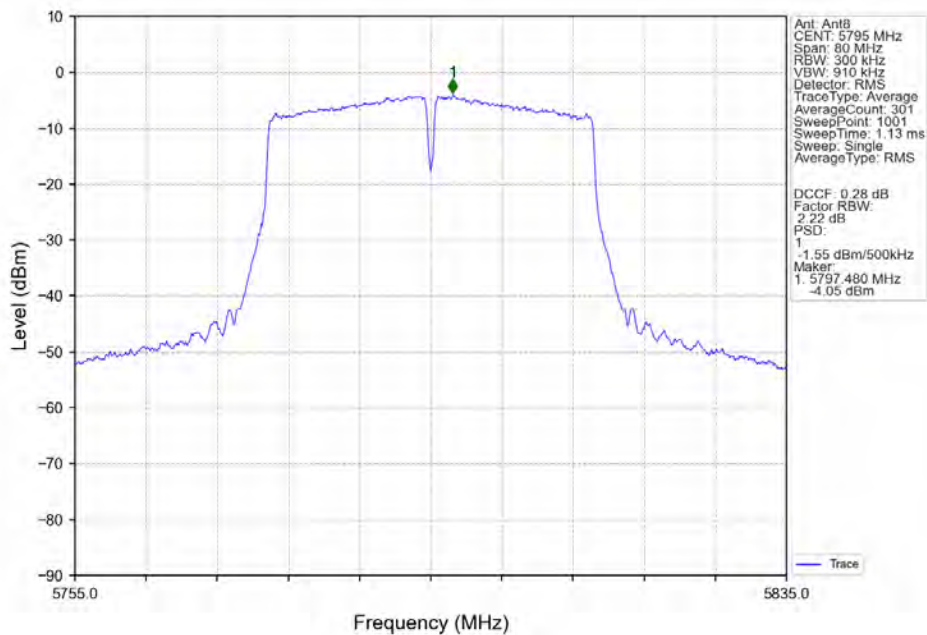
802.11ac(VHT40)_HCH_5795MHz_Ant8_NTNV
