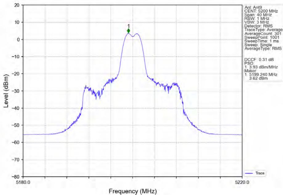
802.11ax(HEW20)_MCH_5200MHz_RU26_Mid_Ant9_NTNV
