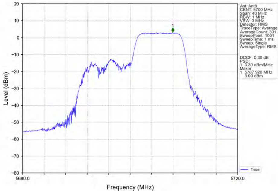
802.11ax(HEW20)_HCH_5700MHz_RU106_Right_MIMO_NTNV
