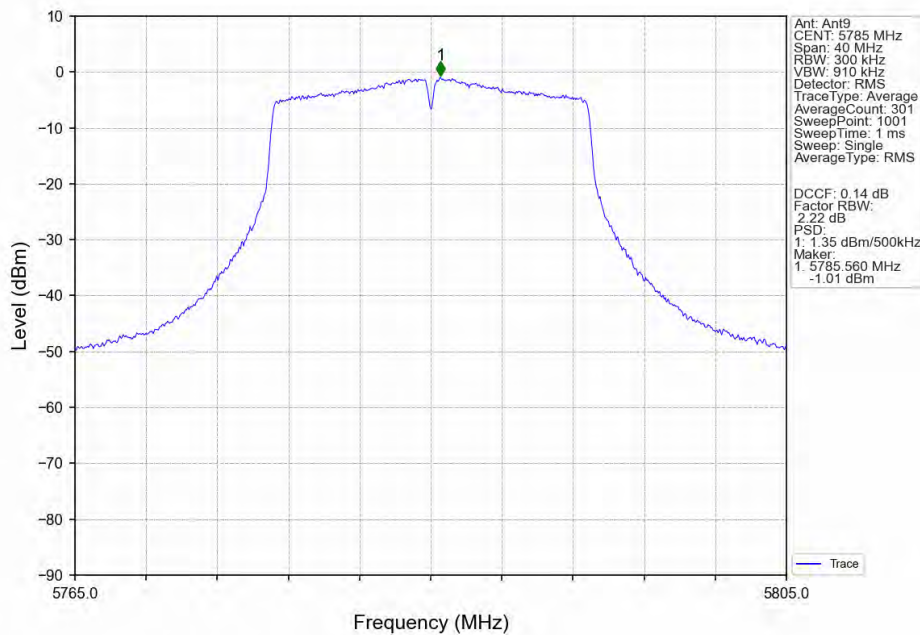
802.11ac(VHT20)_MCH_5785MHz_Ant9_NTNV
