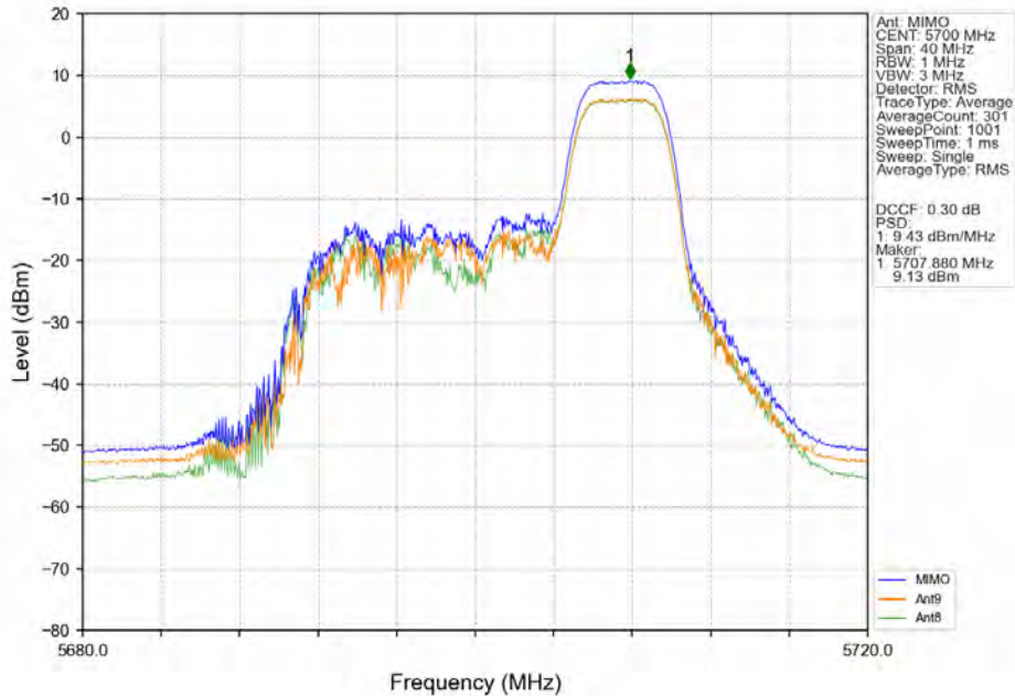
802.11ax(HEW20)_HCH_5700MHz_RU106_Right_Ant9_NTNV
