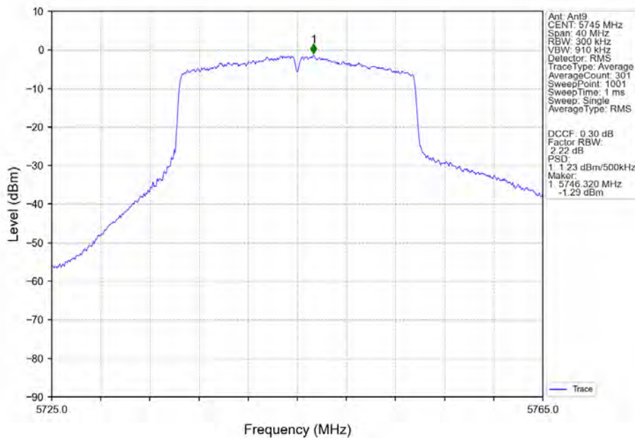
802.11ax(HEW20)_LCH_5745MHz_RU242_Left_Ant9_NTNV
