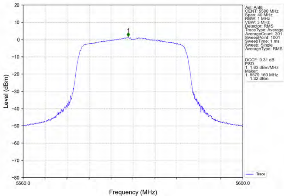
802.11ax(HEW20)_MCH_5580MHz_RU242_Left_Ant8_NTNV
