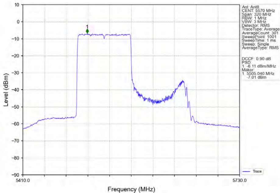
802.11ax(HEW160)_MCH_5570MHz_RU996_Left_MIMO_NTNV
