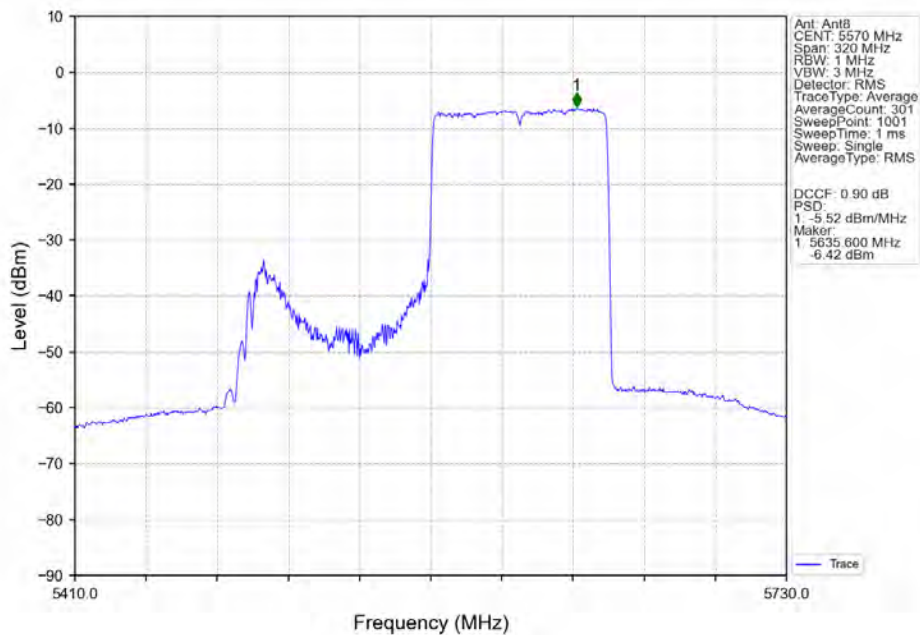
802.11ax(HEW160)_MCH_5570MHz_RU996_Right_Ant8_NTNV
