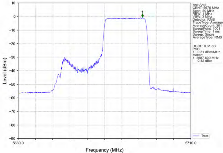
802.11ax(HEW40)_HCH_5670MHz_RU242_Right_MIMO_NTNV
