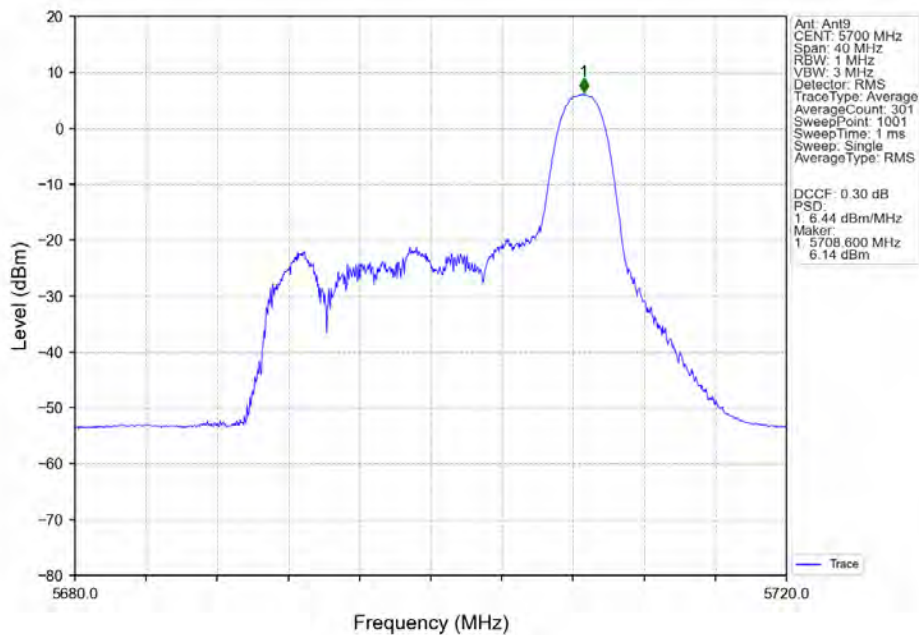
802.11ax(HEW20)_HCH_5700MHz_RU26_Right_Ant9_NTNV
