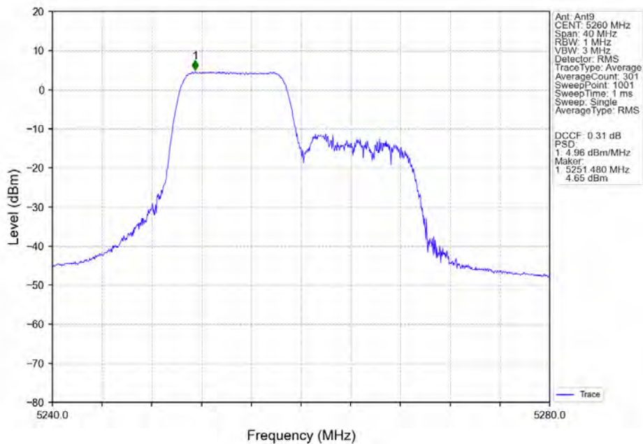
802.11ax(HEW20)_LCH_5260MHz_RU106_Left_Ant9_NTNV
