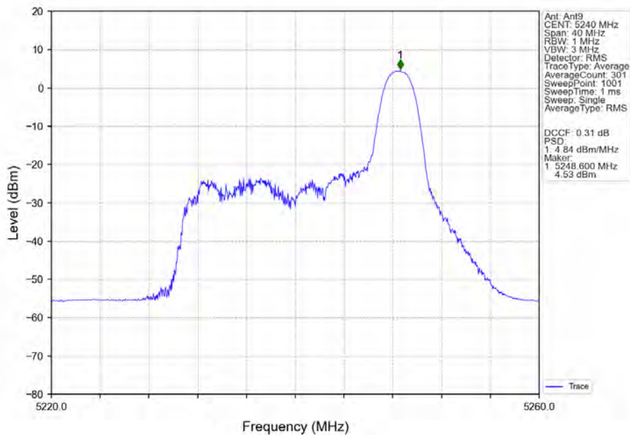
802.11ax(HEW20)_HCH_5240MHz_RU26_Right_Ant9_NTNV
