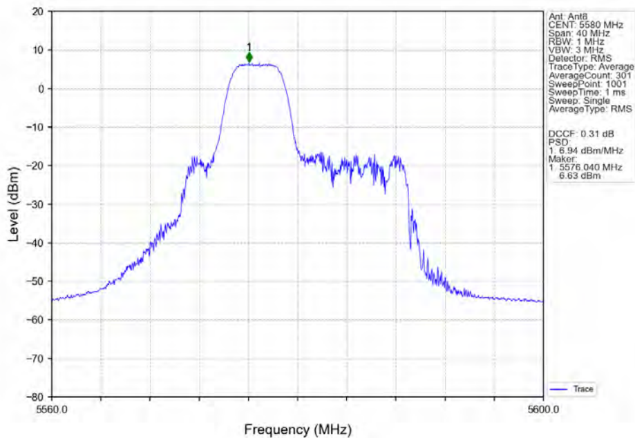
802.11ax(HEW20)_MCH_5580MHz_RU52_Mid_Ant8_NTNV
