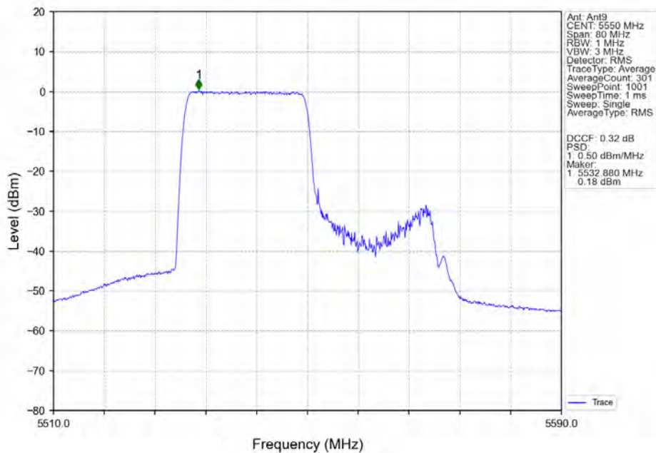
802.11ax(HEW40)_MCH_5550MHz_RU242_Left_Ant9_NTNV
