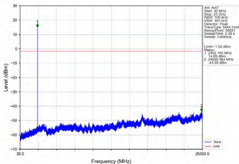
GFSK_DH5_LCH_2402MHz_Ant7_NTNV
