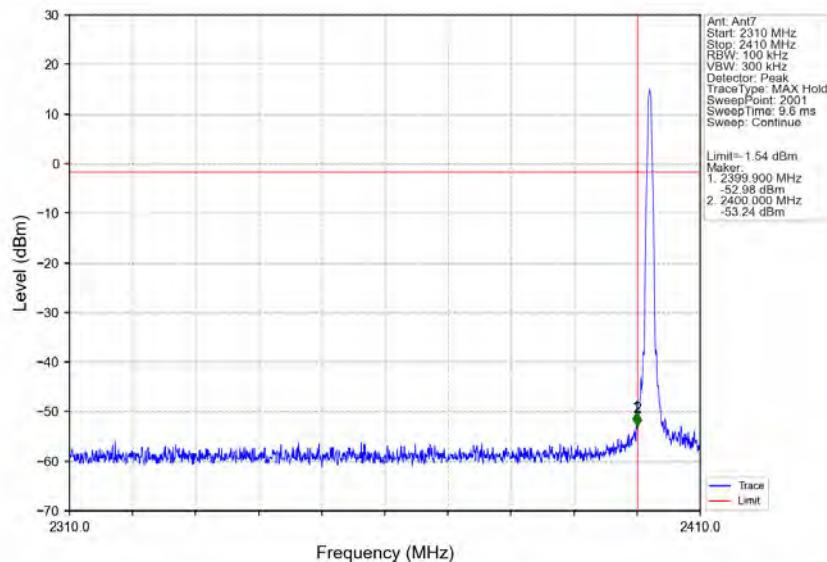
GFSK_DH5_LCH_2402MHz_Ant7_NTNV
