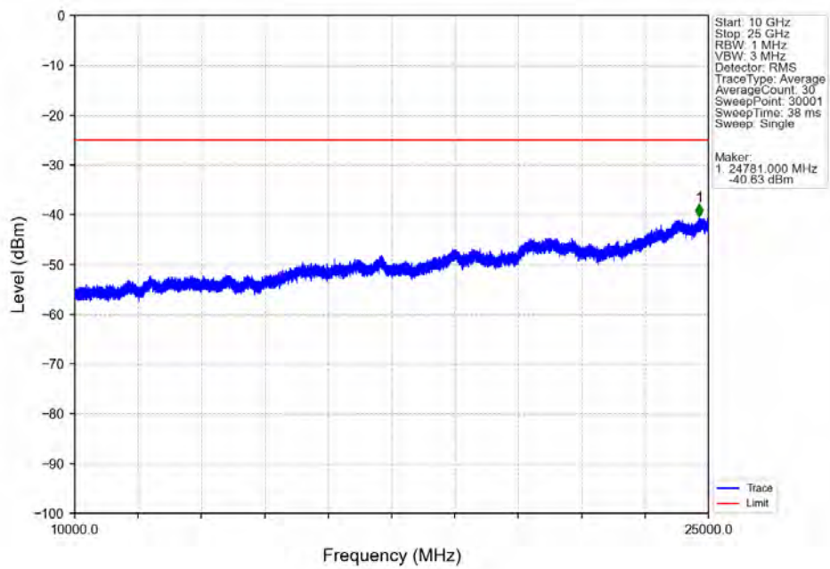
Band7_15MHz_256QAM_MCH_2535MHz_RB_1_0_NTNV
