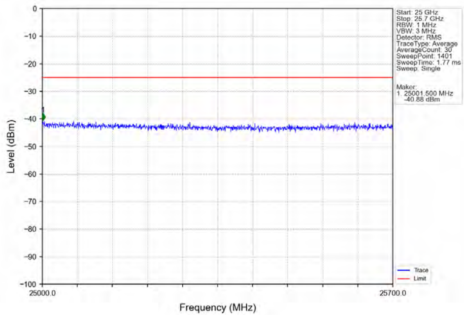
Band7 15MHz 64QAM LCH 2507.5MHz RB 1 0 NTNV
