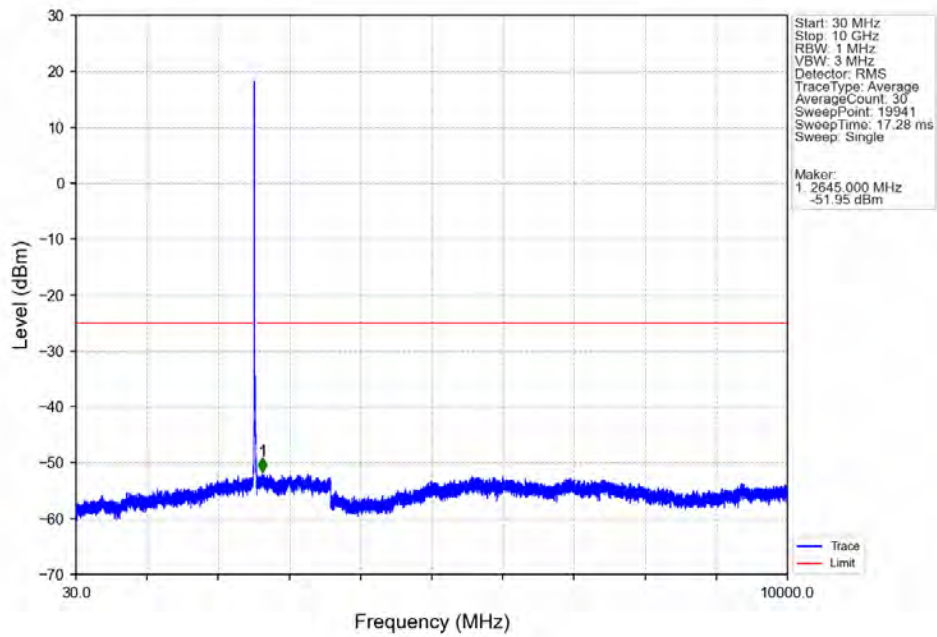
Band7_15MHz_256QAM_MCH_2535MHz_RB_1_0_NTNV
