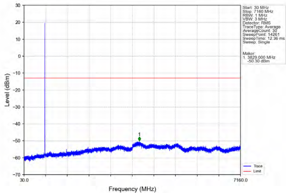
Band12 3MHz 256QAM HCH 714.5MHz RB 1 0 NTNV
