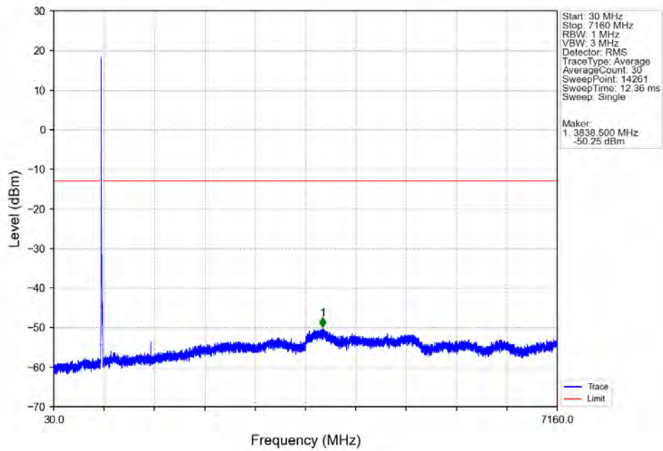
Band12_10MHz_256QAM_HCH_711MHz_RB_1_0_NTNV
