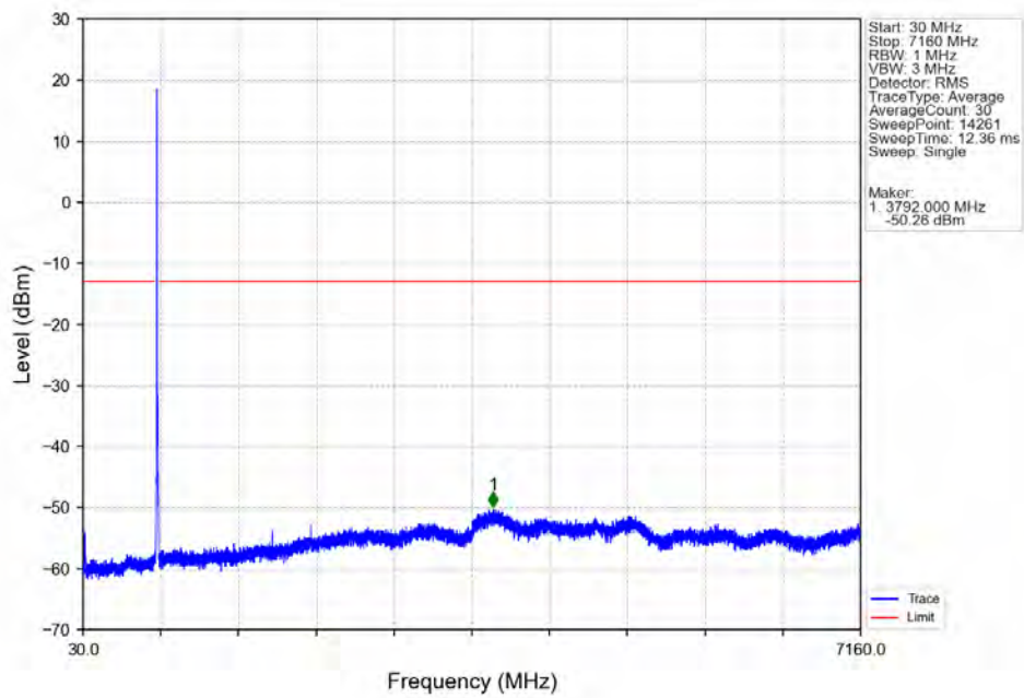
Band12_10MHz_256QAM_HCH_711MHz_RB_1_0_NTNV
