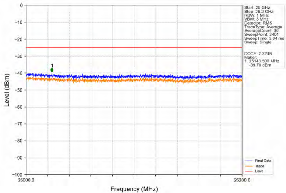
Band38_5MHz_QPSK_LCH_2572.5MHz_RB_1_0_NTV
