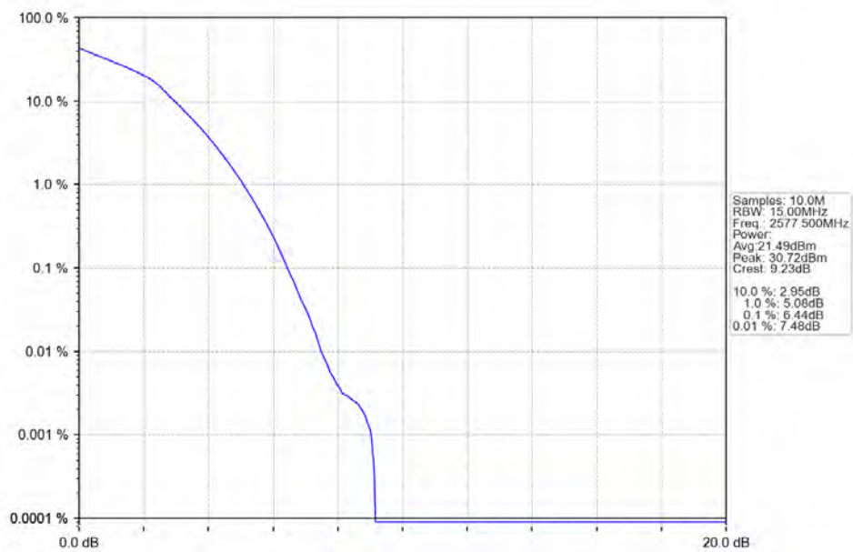
Band38_15MHz_16QAM_LCH_2577.5MHz_RB_75_0_NTN
