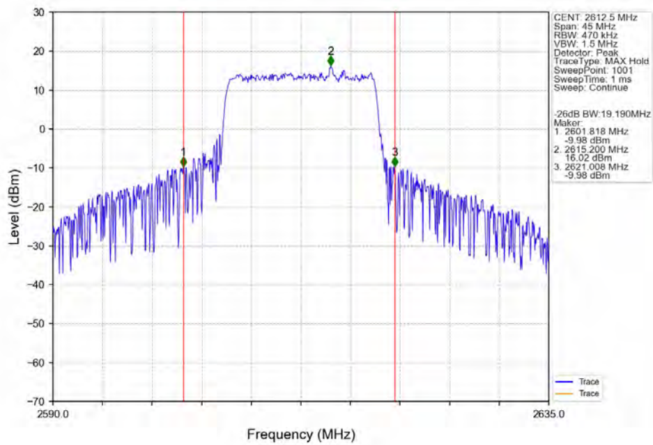
Band38_15MHz_256QAM_HCH_2612.5MHz_RB_75_0_NTNV
