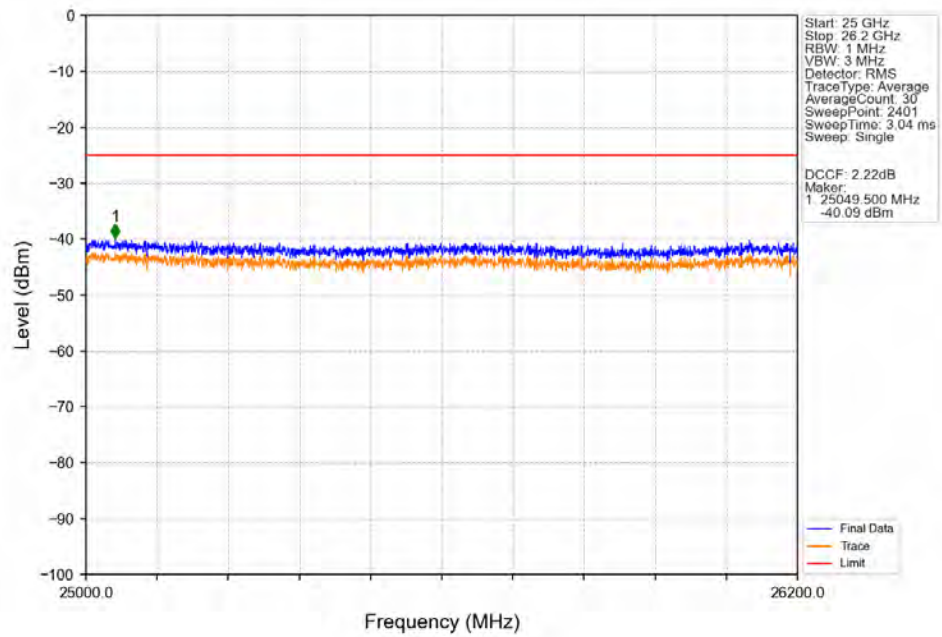
Band38_15MHz_256QAM_HCH_2612.5MHz_RB_1_0_NTNV
