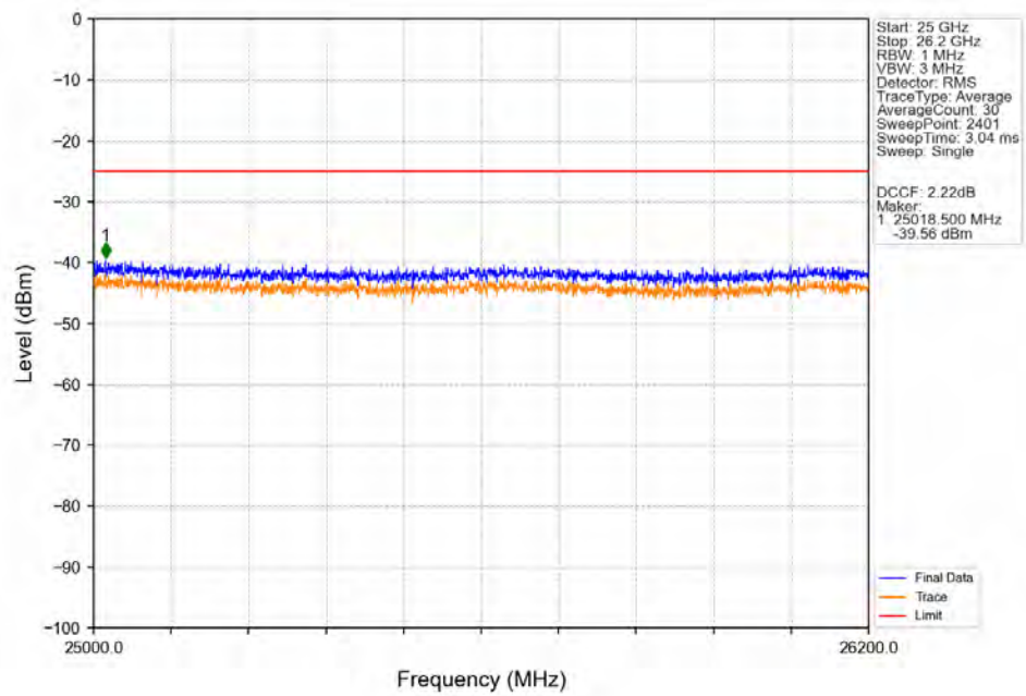
Band38_5MHz_256QAM_HCH_2617.5MHz_RB_1_0_NTN
