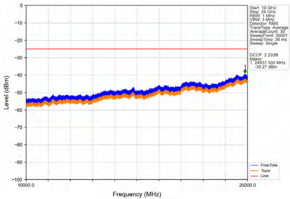
Band38_5MHz_256QAM_MCH_2595MHz_RB_1_0_NTNV
