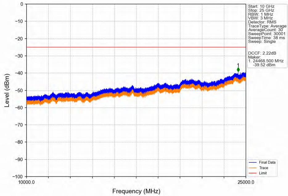
Band38_15MHz_256QAM_HCH_2612.5MHz_RB_1_0_NTNV
