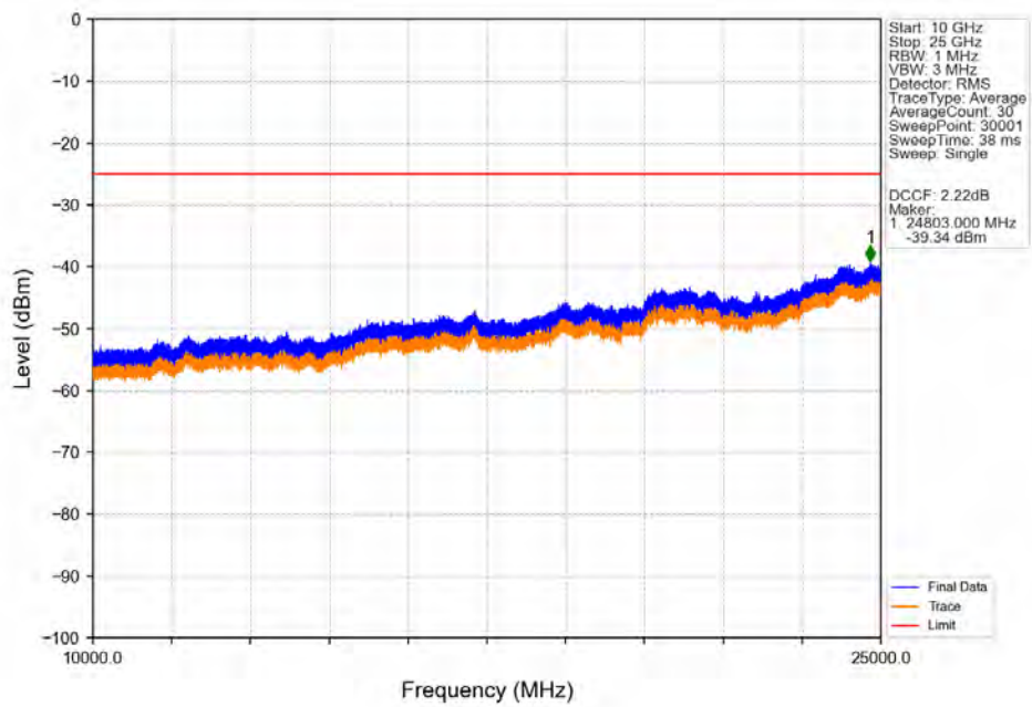
Band38_15MHz_256QAM_LCH_2577.5MHz_RB_1_0_NTNV
