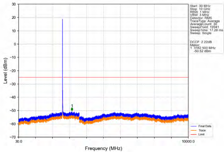
Band38_15MHz_256QAM_HCH_2612.5MHz_RB_1_0 NTN
