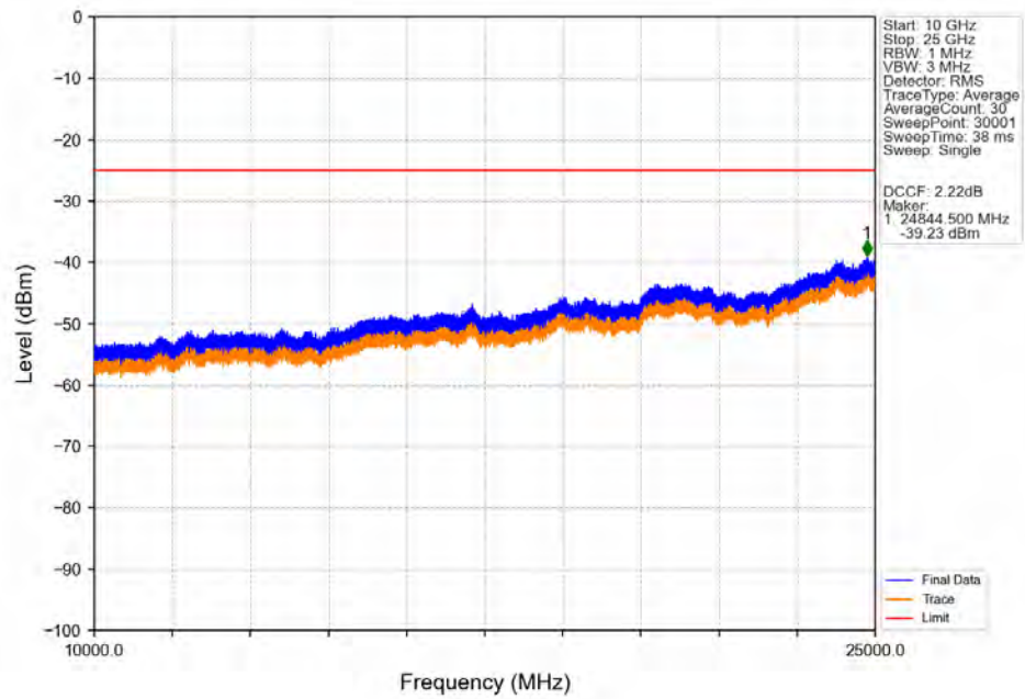
Band38_5MHz_256QAM_HCH_2617.5MHz_RB_1_0_NTN
