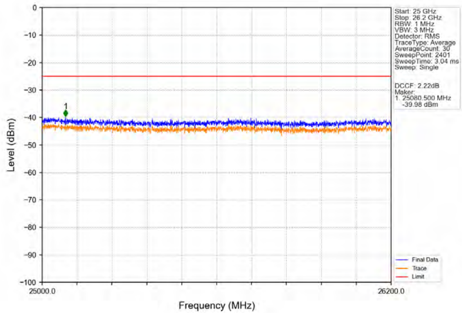
Band38_5MHz_64QAM_MCH_2595MHz_RB_1_0_NTNV
