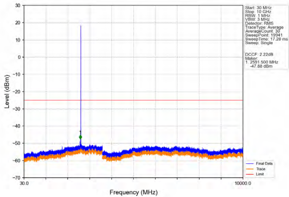
Band38_5MHz_256QAM_HCH_2617.5MHz_RB_1_0_NTNV
