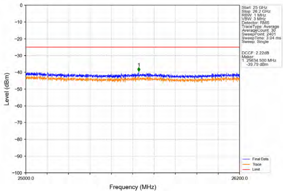
Band38_15MHz_64QAM_MCH_2595MHz_RB_1_0_NTNV
