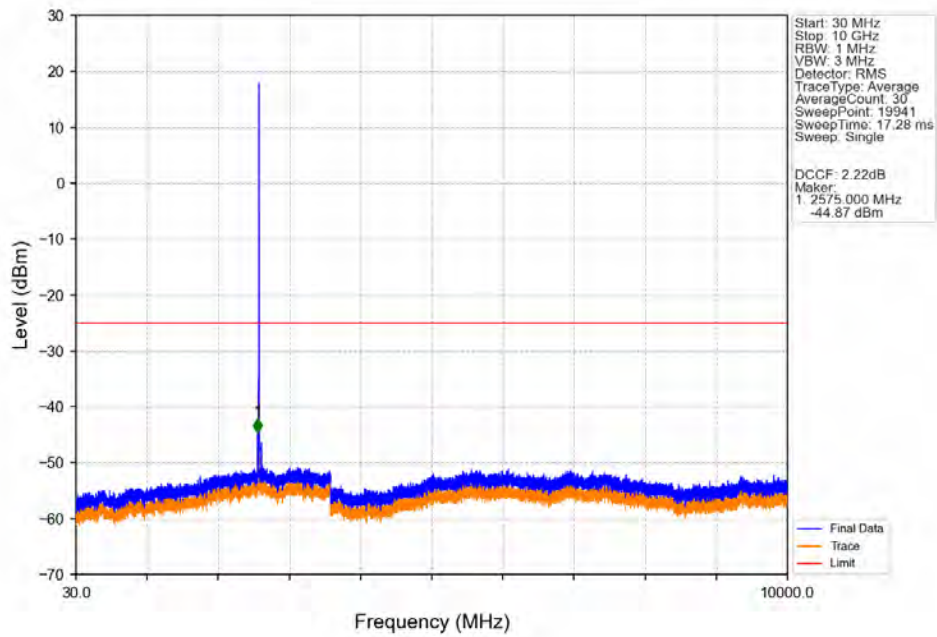
Band38_5MHz_256QAM_MCH_2595MHz_RB_1_0_NTNV
