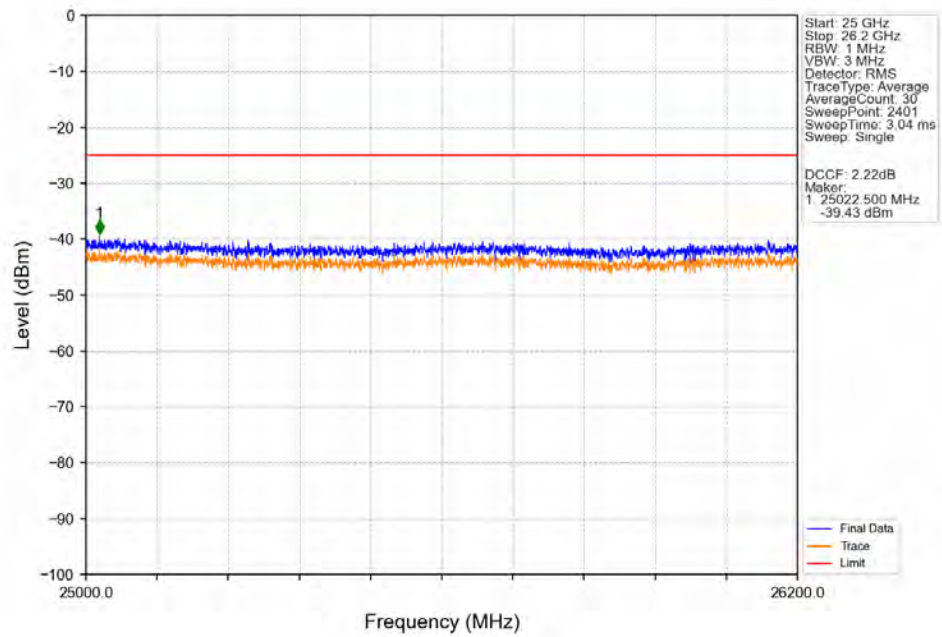
Band38_15MHz_256QAM_HCH_2612.5MHz_RB_1_0 NTN
