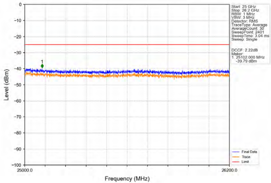
Band38_20MHz_64QAM_MCH_2595MHz_RB_1_0_NTNV
