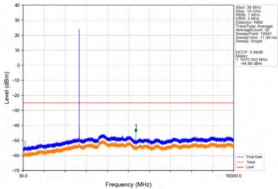
Band41_5MHz_16QAM_HCH_2687.5MHz_RB_1_0_NTV
