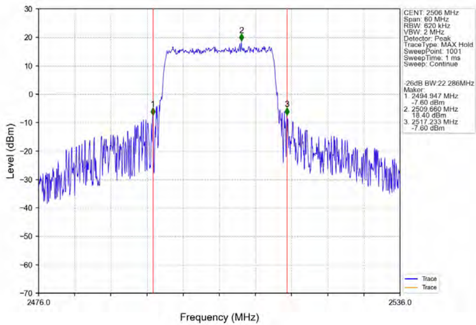
Band41_20MHz_256QAM_LCH_2506MHz_RB_100_0_NTNV
