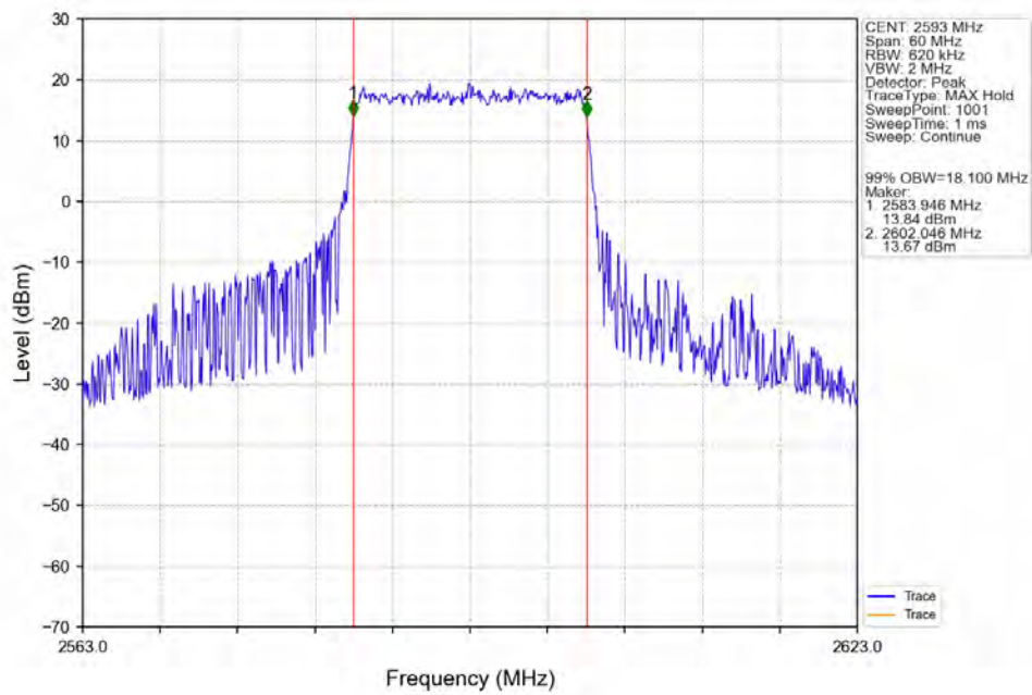
Band41_20MHz_64QAM_MCH_2593MHz_RB_100_0_NTNV
