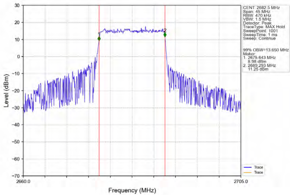
Band41_15MHz_256QAM_HCH_2682.5MHz_RB_75_0_NTNV
