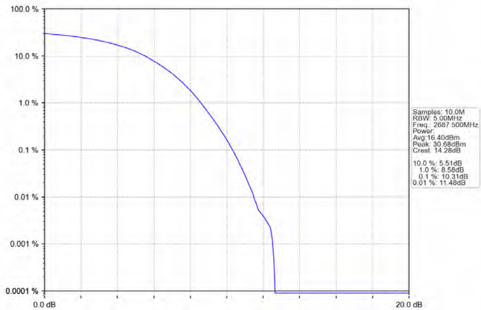
Band41_5MHz_256QAM_HCH_2687.5MHz_RB_25_0_NTNV
