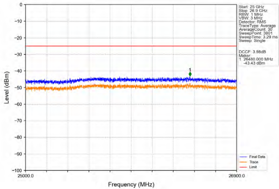
Band41_5MHz_16QAM_HCH_2687.5MHz_RB_1_0_NTV
