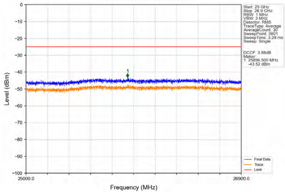
Band41_5MHz_64QAM_LCH_2498.5MHz_RB_1_0_NTNV
