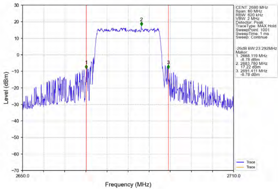
Band41_20MHz_256QAM_HCH_2680MHz_RB_100_0 NTN
