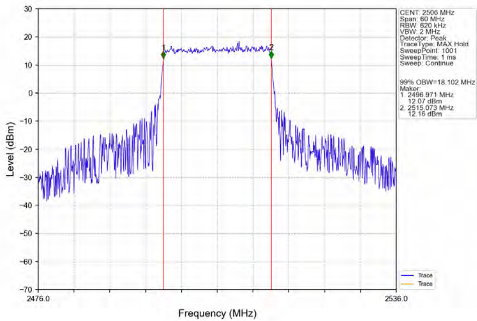
Band41_20MHz_256QAM_LCH_2506MHz_RB_100_0_NTNV
