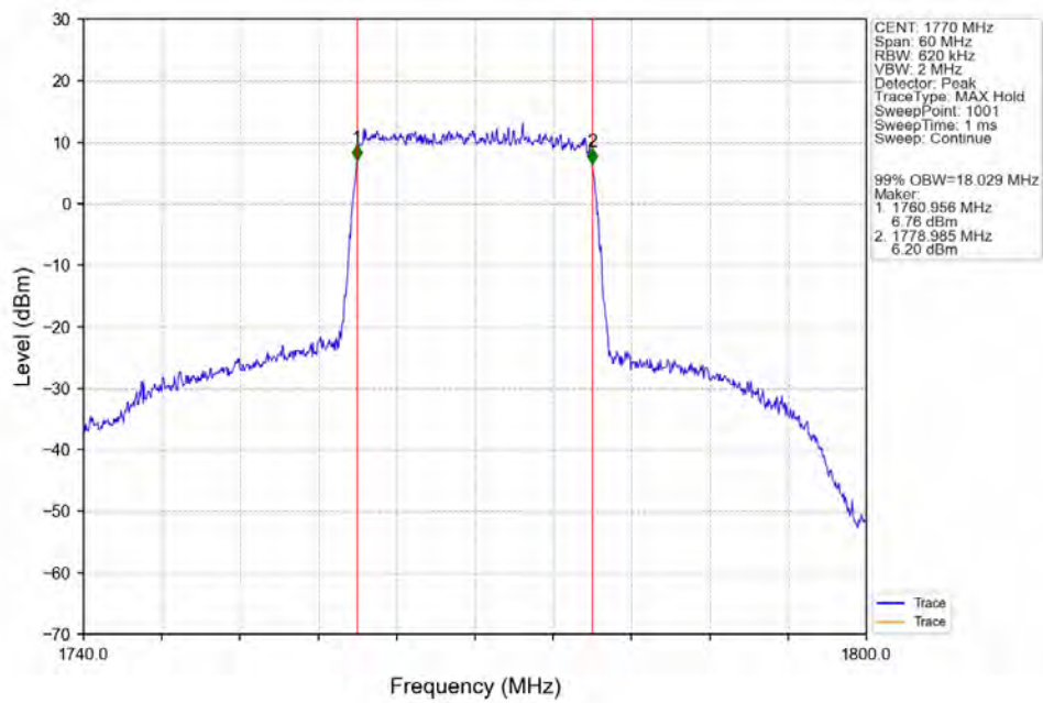
Band66_20MHz_256QAM_HCH_1770MHz_RB_100_0 NTN
