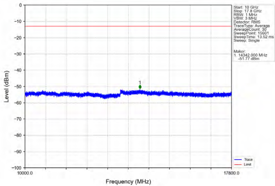
Band66_3MHz_256QAM_HCH_1778.5MHz_RB_1_0_NTNV
