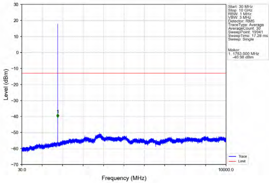
Band66_1.4MHz_64QAM_HCH_1779.3MHz_RB_1_0_NTNV
