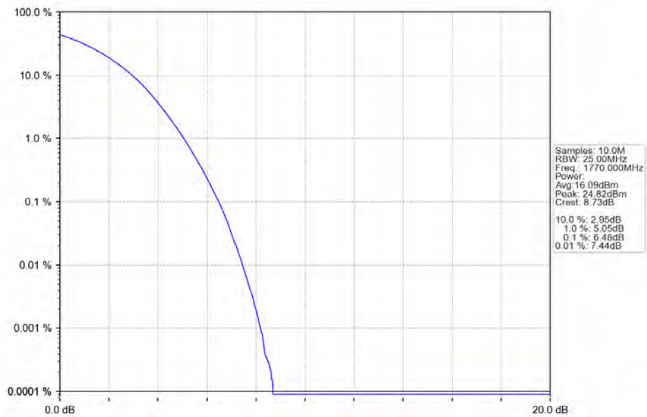
Band66_20MHz_256QAM_HCH_1770MHz_RB_100_0 NTN
