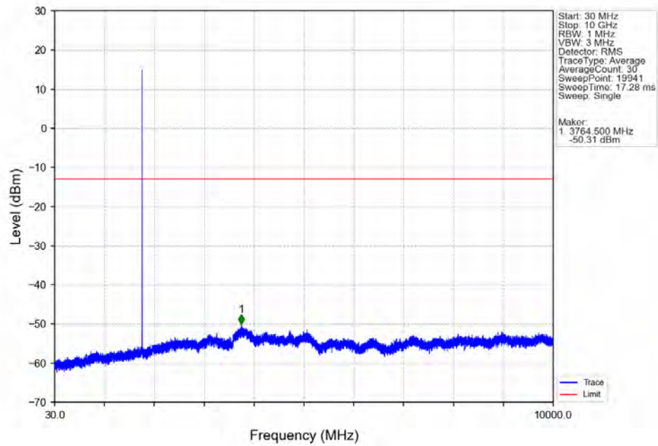
Band66_3MHz_256QAM_HCH_1778.5MHz_RB_1_0_NTNV
