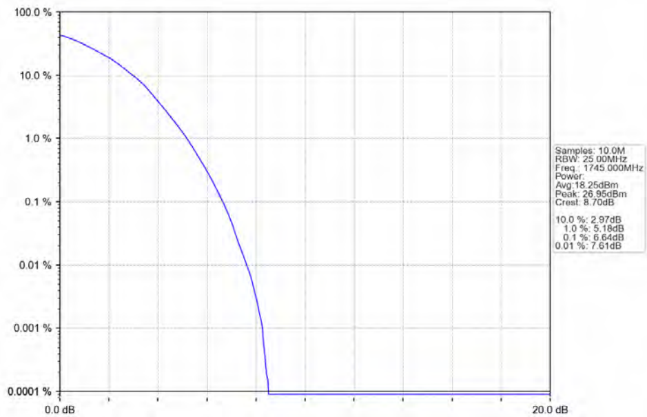
Band66_20MHz_64QAM_MCH_1745MHz_RB_100_0 NTN
