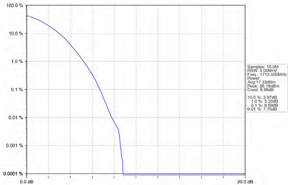
Band66_5MHz_256QAM_LCH_1712.5MHz_RB_25_0_NTN
