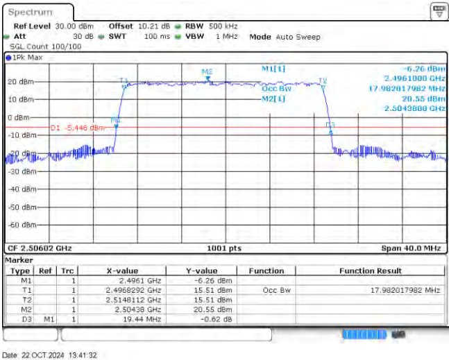
1-N41-PC2-30-20-L-2-DFT-PI2BPSK-Out_Full-50@0-Ant5-17.982-19.440-≤20-PASS
