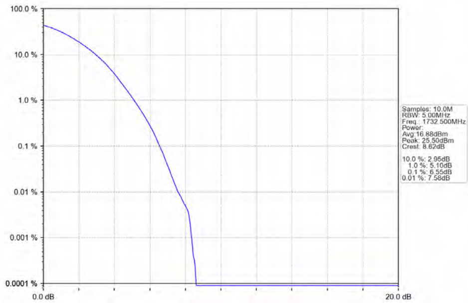
Band4 5MHz 256QAM MCH 1732.5MHz RB 25 0 NTNV
