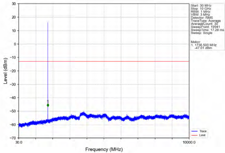
Band4 1.4MHz 256QAM MCH 1732.5MHz RB 1 0 NTNV
