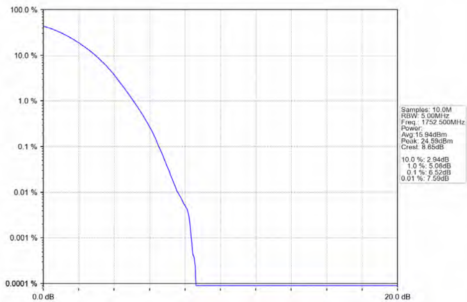
Band4 5MHz 256QAM HCH 1752.5MHz RB 25 0 NTNV
