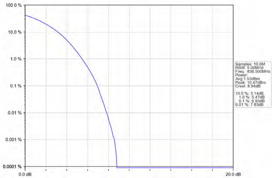
Band5_3MHz_256QAM_MCH_836.5MHz_RB_15_0_NTNV
