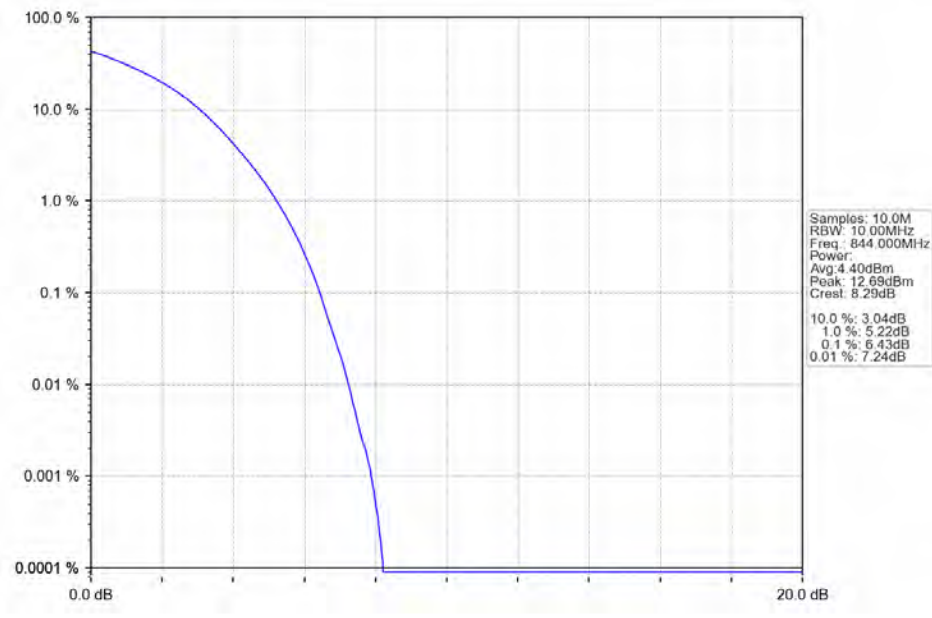
Band5_10MHz_16QAM_HCH_844MHz_RB_50_0_NTNV
