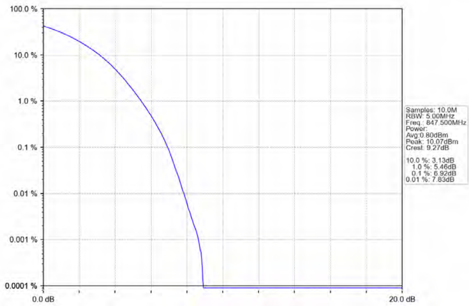
Band5_3MHz_256QAM_HCH_847.5MHz_RB_15_0_NTNV
