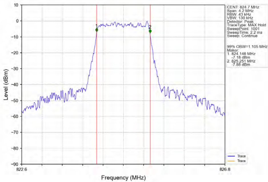
Band5_1.4MHz_256QAM_LCH_824.7MHz_RB_6_0_NTNV
