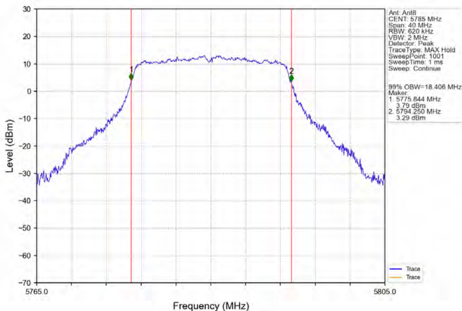
802.11ac(VHT20)_MCH_5785MHz_Ant8_NTNV
