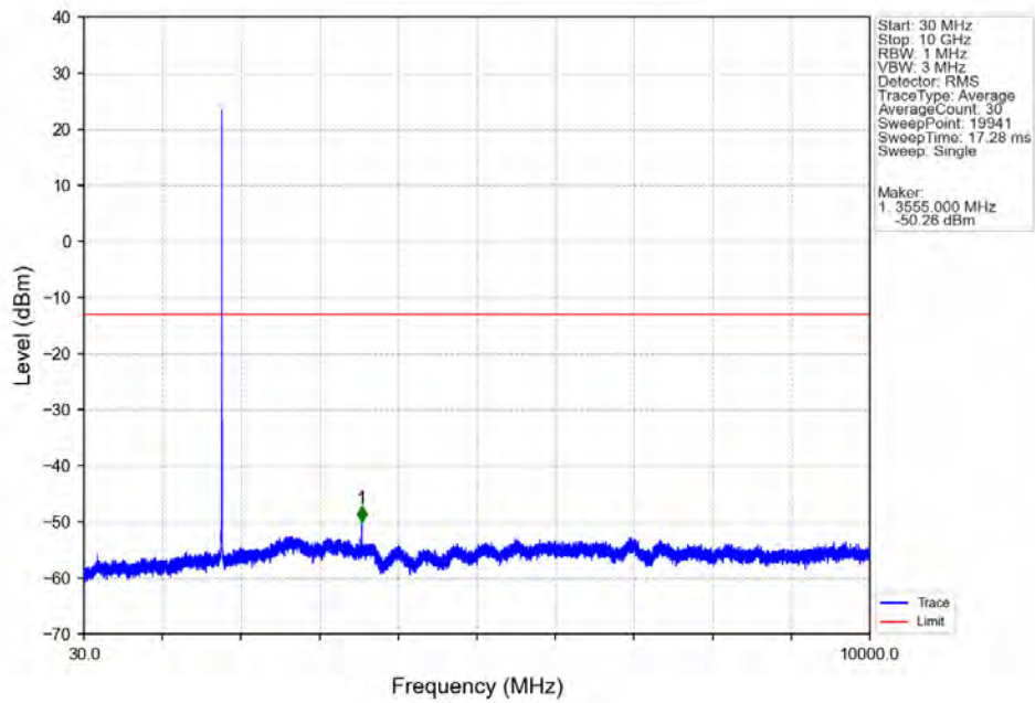
Band66_3MHz_16QAM_HCH_1778.5MHz_RB_1_0_NTV
