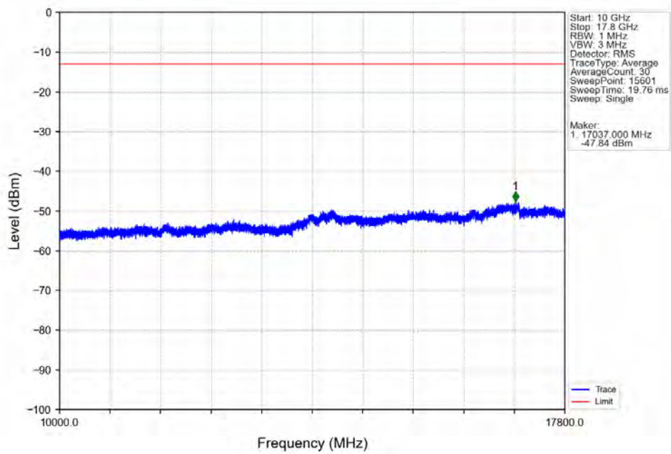
Band66_3MHz_16QAM_MCH_1745MHz_RB_1_0_NTV
