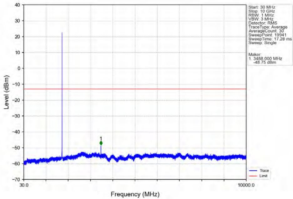
Band66_3MHz_16QAM_MCH_1745MHz_RB_1_0_NTV
