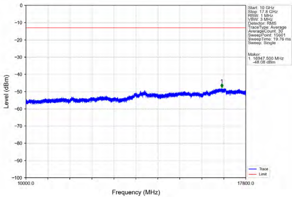
Band66_3MHz_16QAM_HCH_1778.5MHz_RB_1_0_NTV
