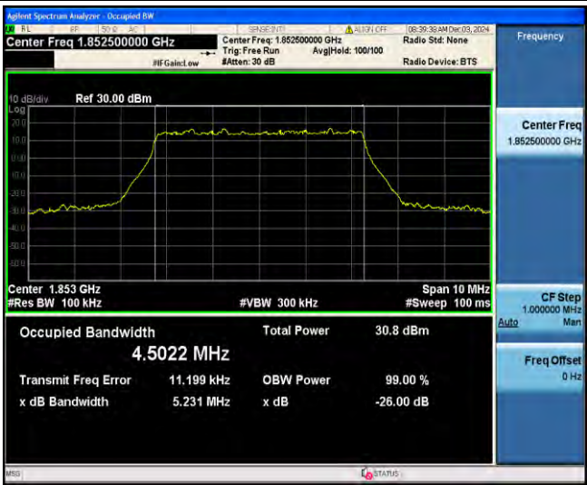
1-N2-PC3-15-5-L-1-DFT-QPSK-Outer_Full-25@0-Ant3-4.5022-5.231-≤5-PASS
