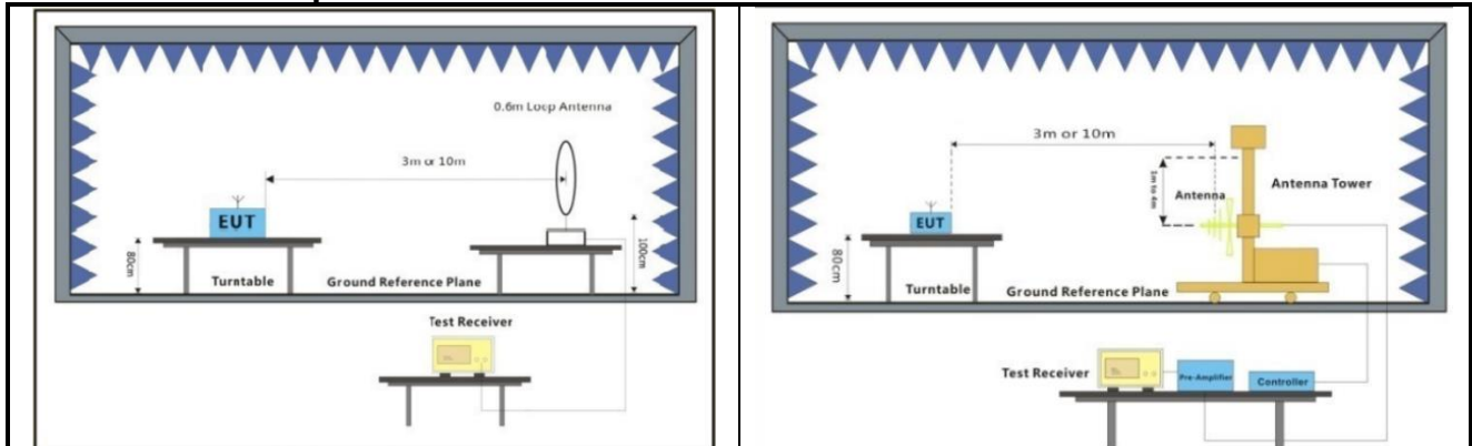
Figure 1. Below 30MHz
