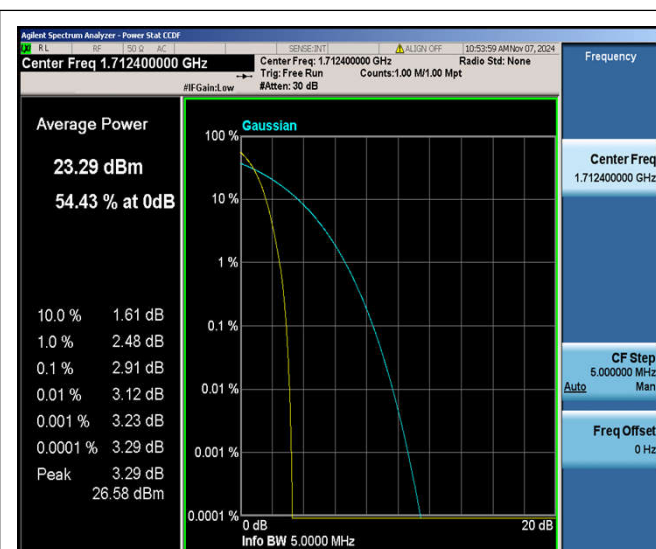
Band4-1312
