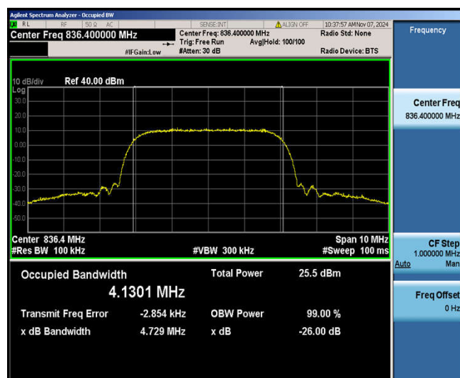
Band5-4182-4.729
