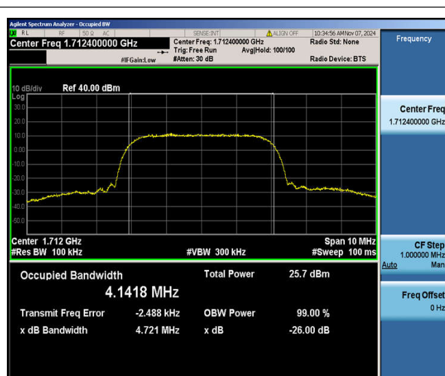
Band4-1312-4.721
