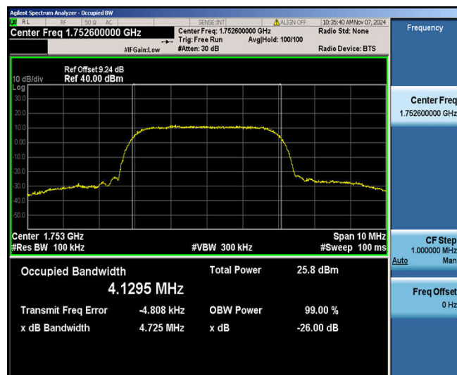
Band4-1513-4.725
