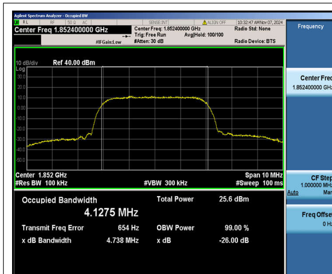
Band2-9262-4.738
