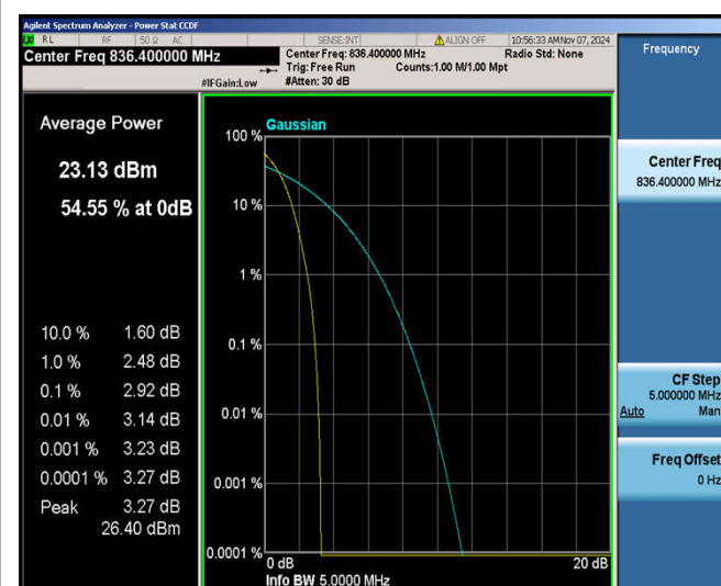
Band5-4182
