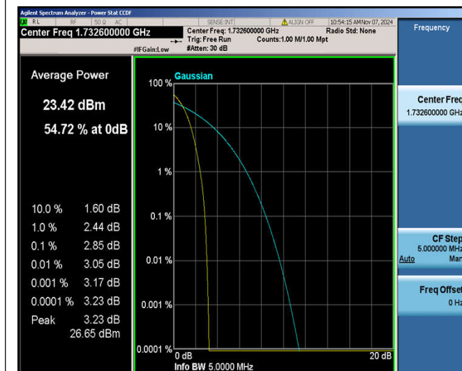
Band4-1413
