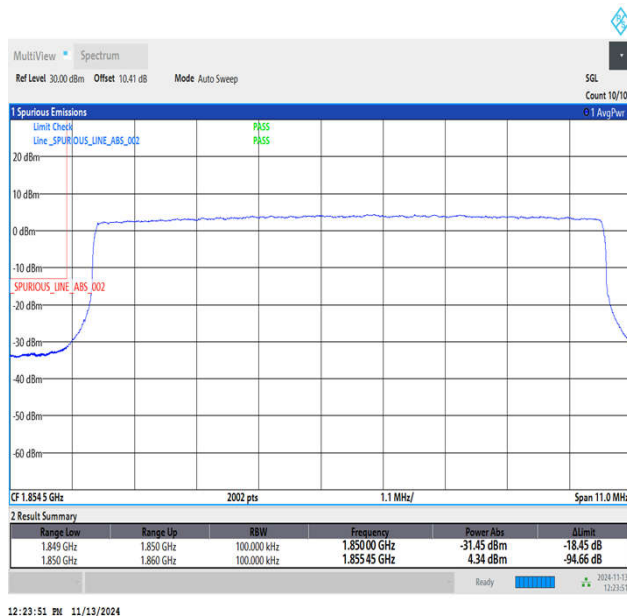
Band2_10MHz_16QAM_18650_50RB#0
