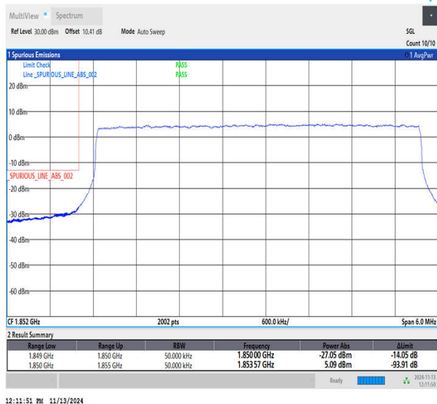
Band2_5MHz_QPSK_18625_25RB#0
