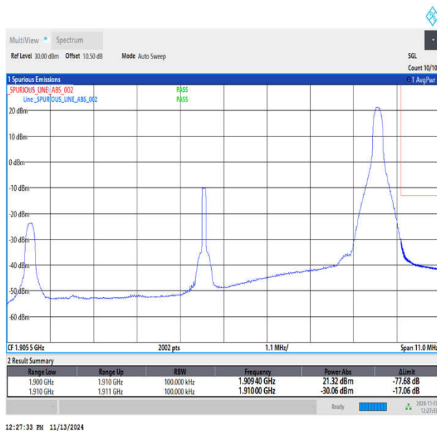
Band2_10MHz_16QAM_19150_1RB#49
