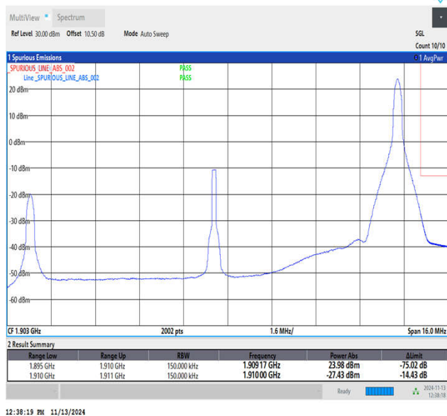
Band2_15MHz_QPSK_19125_1RB#74
