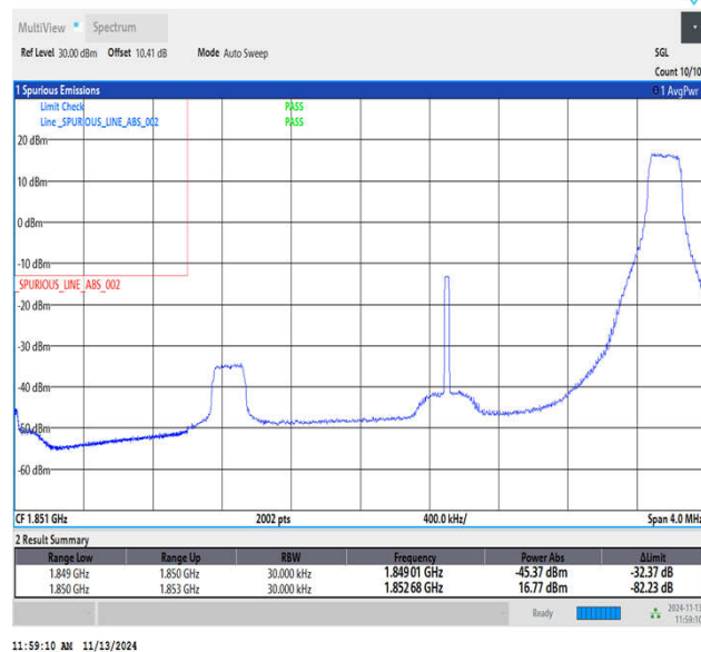
Band2_3MHz_16QAM_18615_1RB#14
