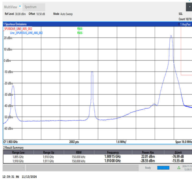
Band2_15MHz_64QAM_19125_1RB#74
