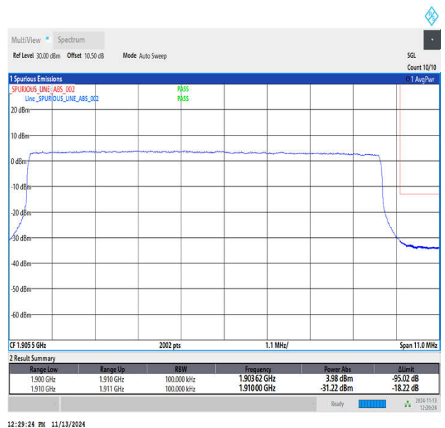
Band2_10MHz_16QAM_19150_50RB#0
