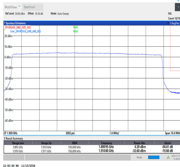
Band2_15MHz_16QAM_19125_75RB#0
