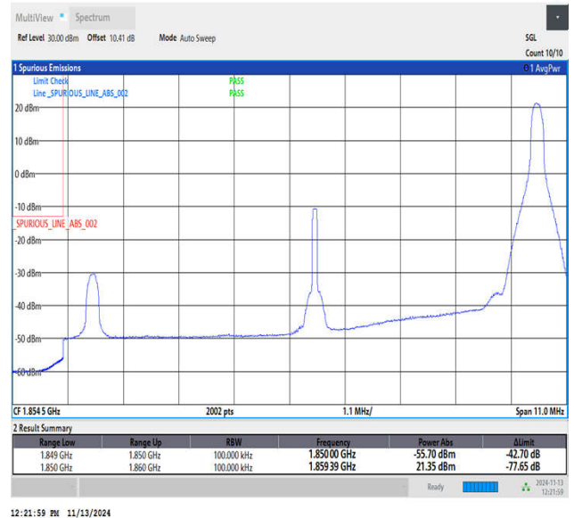
Band2_10MHz_16QAM_18650_1RB#49
