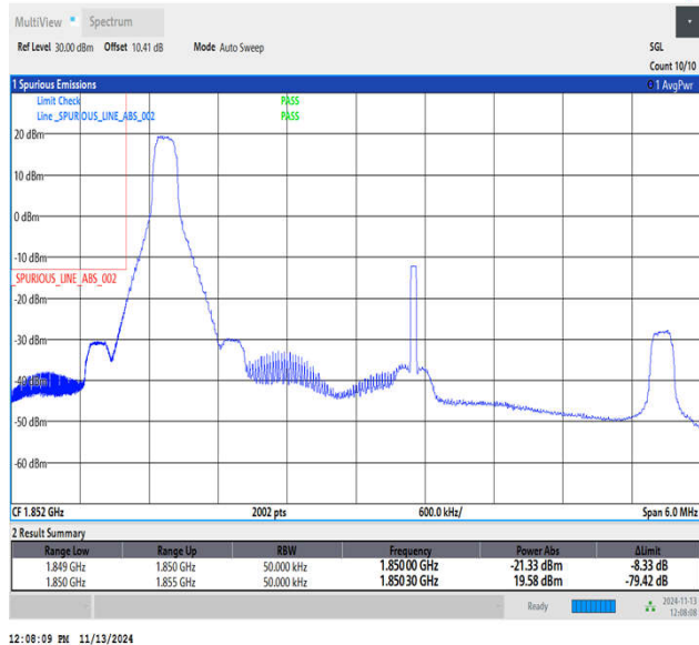
Band2_5MHz_QPSK_18625_1RB#0
