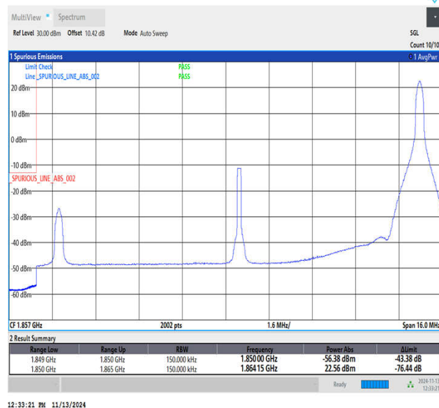
Band2_15MHz_16QAM_18675_1RB#74
