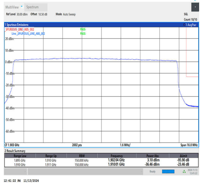
Band2_15MHz_64QAM_19125_75RB#0
