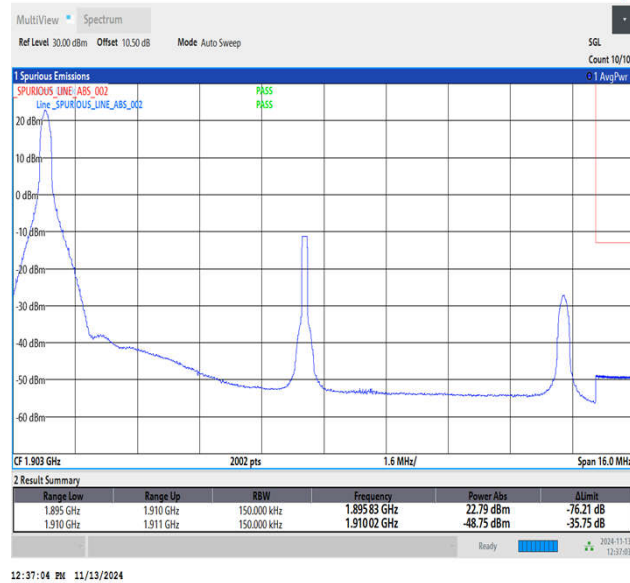
Band2_15MHz_16QAM_19125_1RB#0
