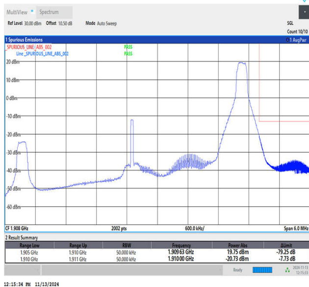
Band2_5MHz_QPSK_19175_1RB#24
