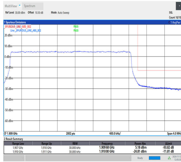
Band2_3MHz_QPSK_19185_15RB#0
