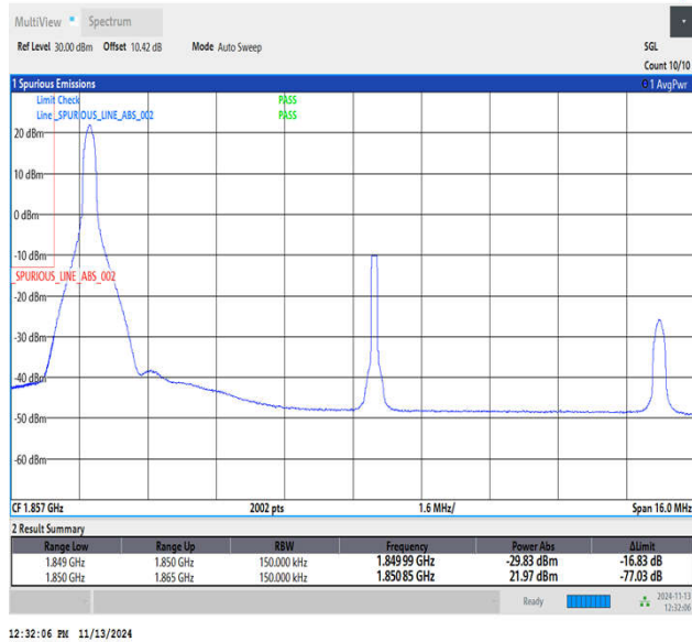
Band2_15MHz_64QAM_18675_1RB#0
