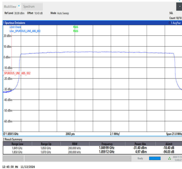
Band2_20MHz_QPSK_18700_100RB#0
