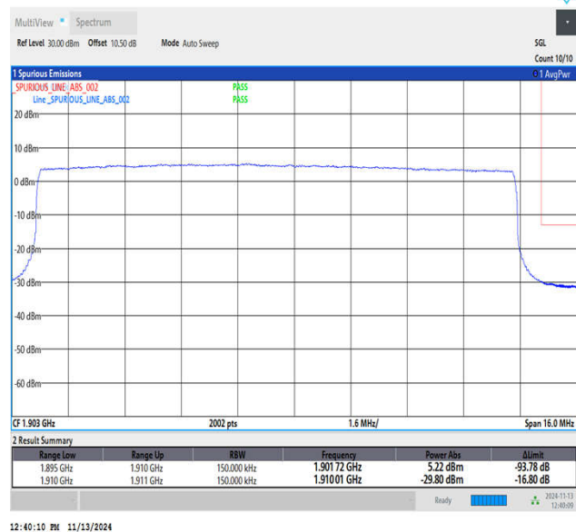
Band2_15MHz_QPSK_19125_75RB#0
