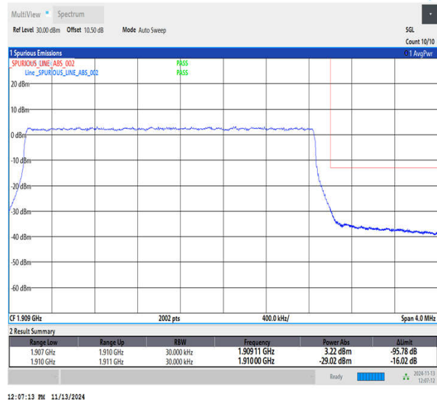
Band2_3MHz_64QAM_19185_15RB#0
