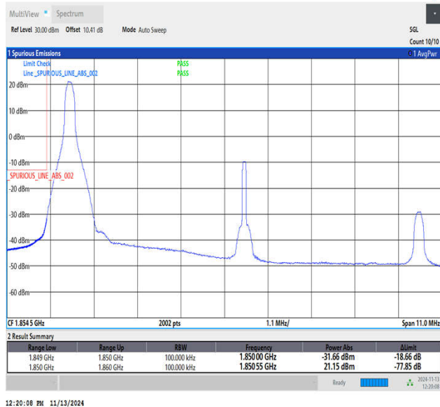
Band2_10MHz_16QAM_18650_1RB#0
