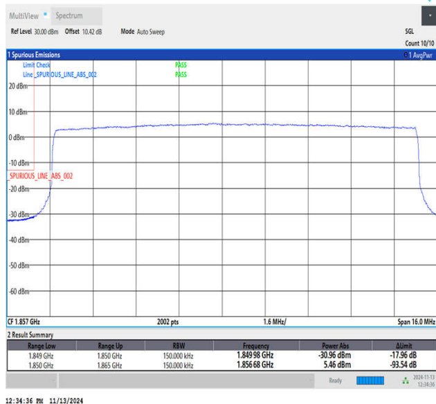
Band2_15MHz_QPSK_18675_75RB#0
