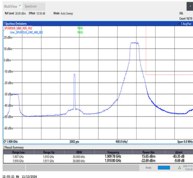
Band2_3MHz_64QAM_19185_1RB#14
