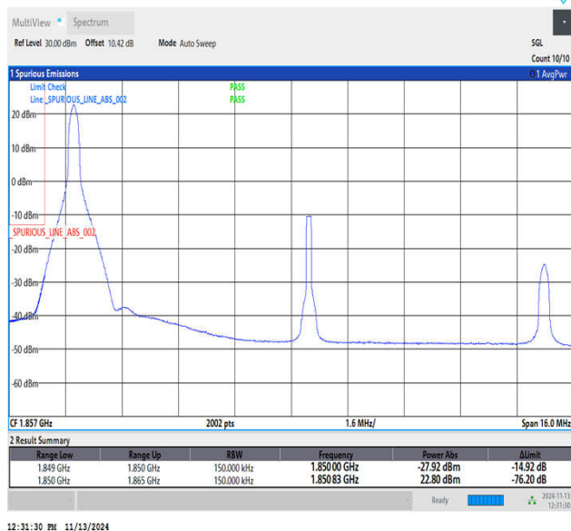
Band2_15MHz_16QAM_18675_1RB#0
