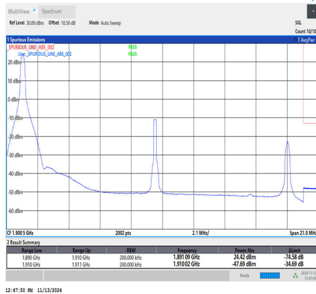
Band2_20MHz_QPSK_19100_1RB#0
