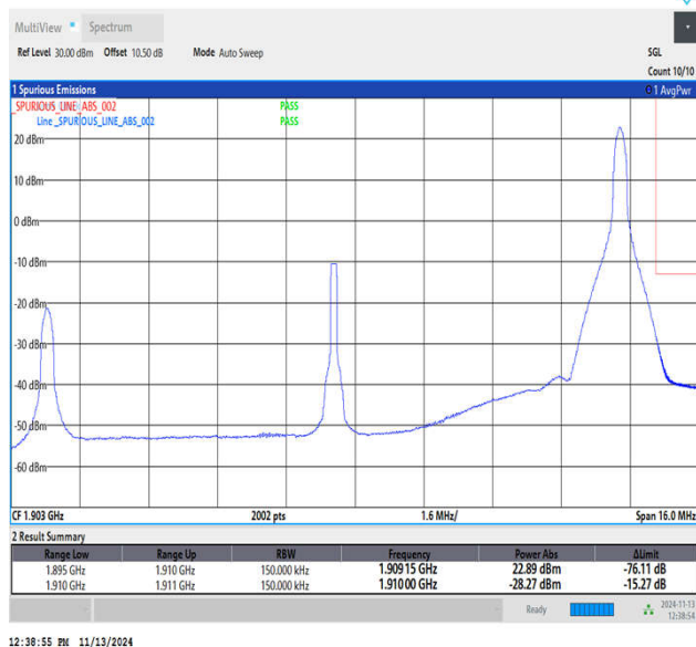
Band2_15MHz_16QAM_19125_1RB#74
