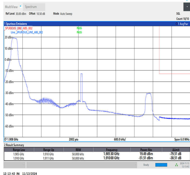
Band2_5MHz_QPSK_19175_1RB#0
