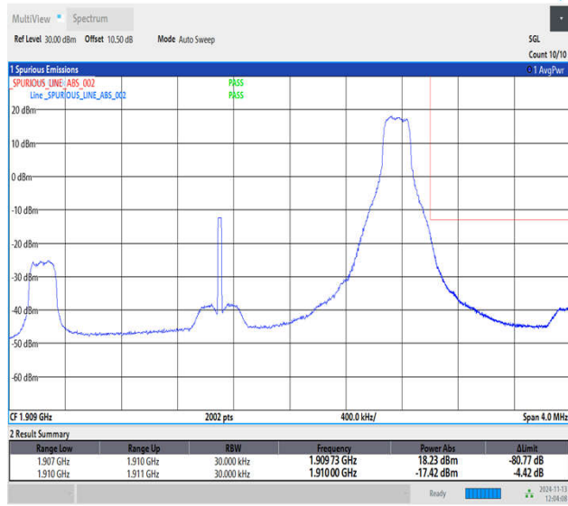
Band2_3MHz_QPSK_19185_1RB#14
