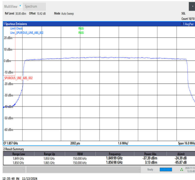
Band2_15MHz_64QAM_18675_75RB#0
