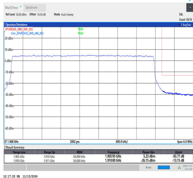
Band2_5MHz_QPSK_19175_25RB#0
