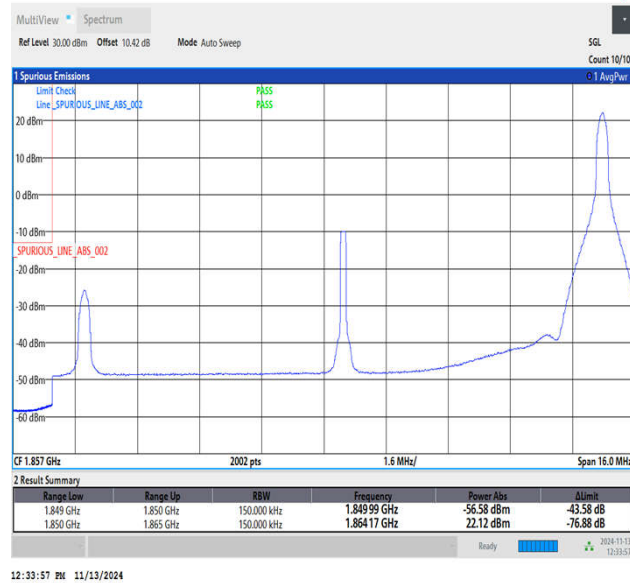
Band2_15MHz_64QAM_18675_1RB#74
