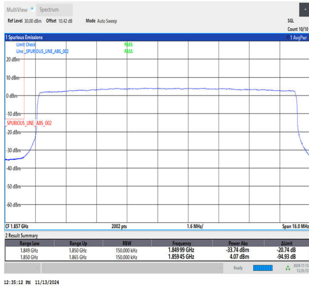
Band2_15MHz_16QAM_18675_75RB#0
