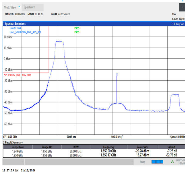
Band2_3MHz_16QAM_18615_1RB#0
