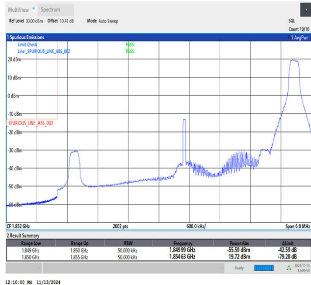
Band2_5MHz_QPSK_18625_1RB#24
