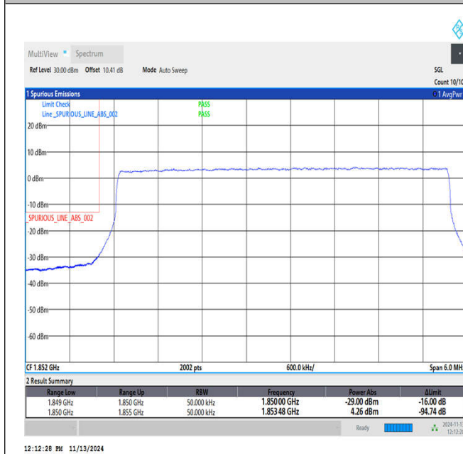
Band2_5MHz_16QAM_18625_1RB#0
