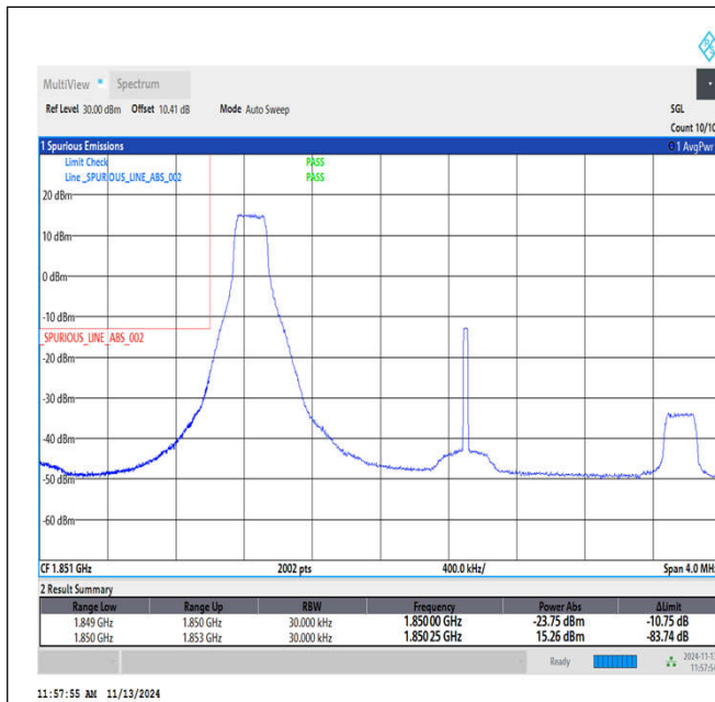
Band2_3MHz_64QAM_18615_1RB#0
