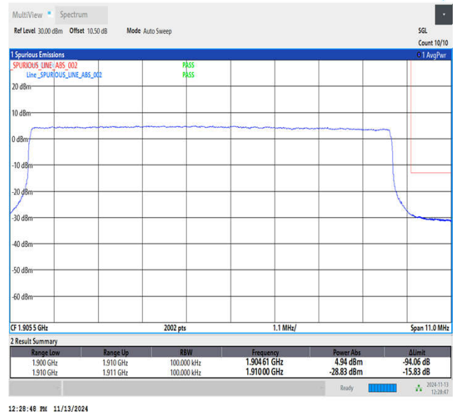
Band2_10MHz_QPSK_19150_50RB#0
