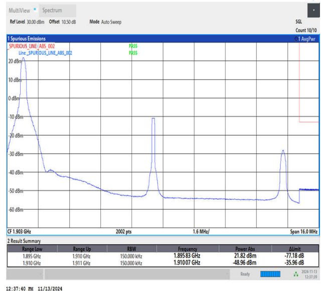
Band2_15MHz_64QAM_19125_1RB#0
