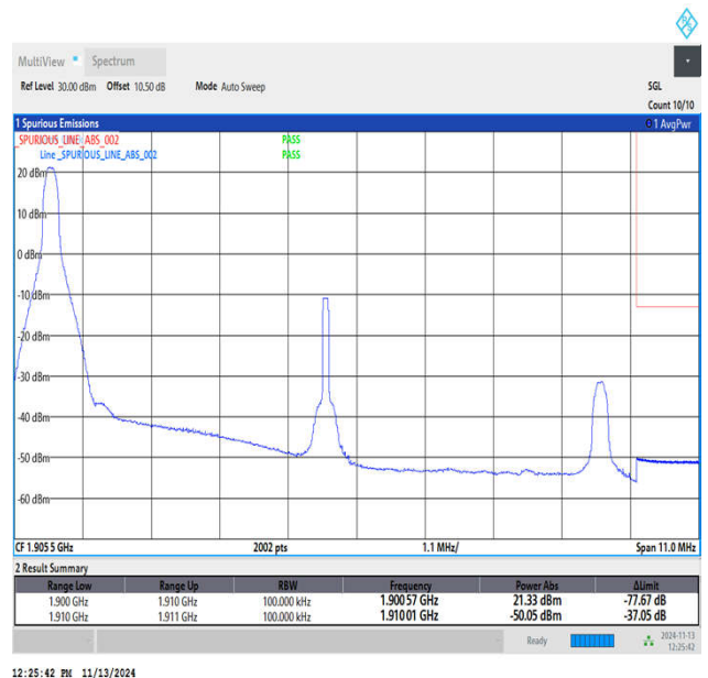
Band2_10MHz_16QAM_19150_1RB#0
