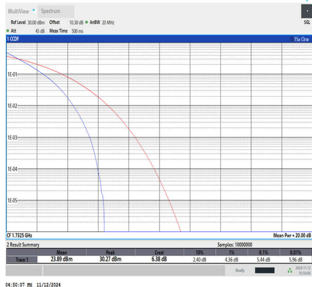
Band4-15MHz-QPSK-20175-75RB#0-PASS
