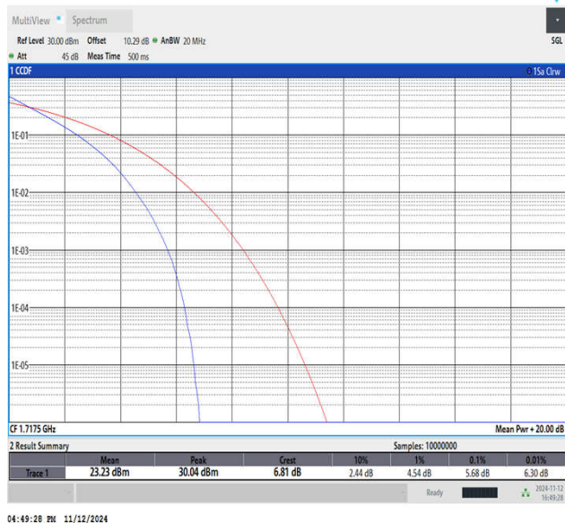
Band4-15MHz-QPSK-20025-75RB#0-PASS
