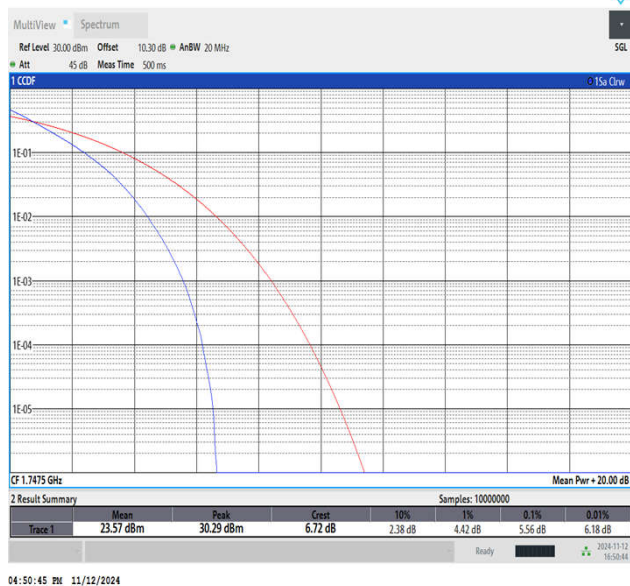
Band4-15MHz-QPSK-20325-75RB#0-PASS
