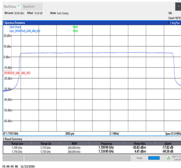
Band4_20MHz_QPSK_20050_100RB#0
