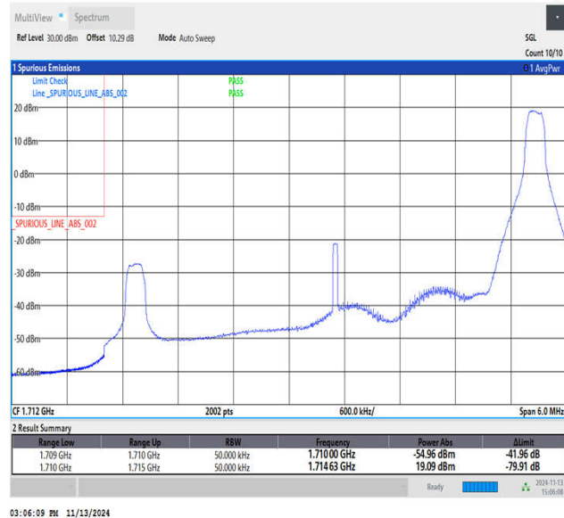
Band4_5MHz_QPSK_19975_1RB#24
