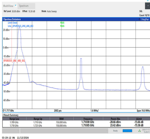
Band4_15MHz_QPSK_20025_1RB#0
