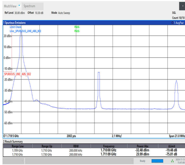
Band4_20MHz_QPSK_20050_1RB#0
