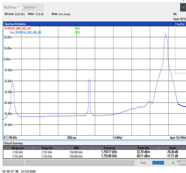
Band4_15MHz_QPSK_20325_1RB#74
