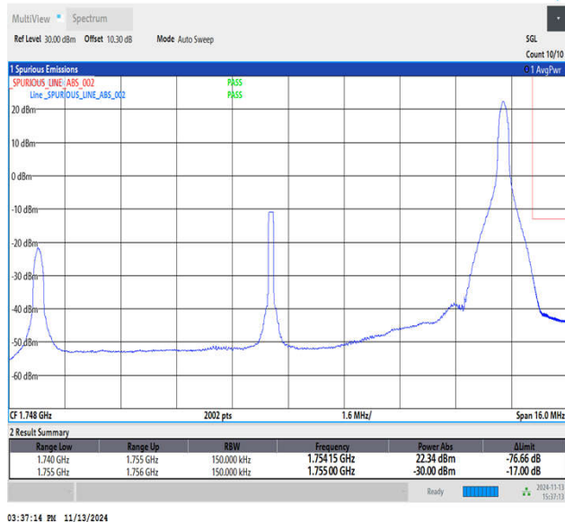
Band4_15MHz_16QAM_20325_1RB#74
