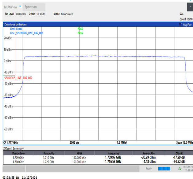
Band4_15MHz_QPSK_20025_75RB#0
