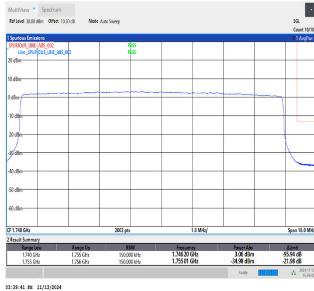
Band4_15MHz_64QAM_20325_75RB#0
