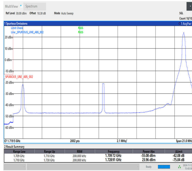
Band4_20MHz_QPSK_20050_1RB#99
