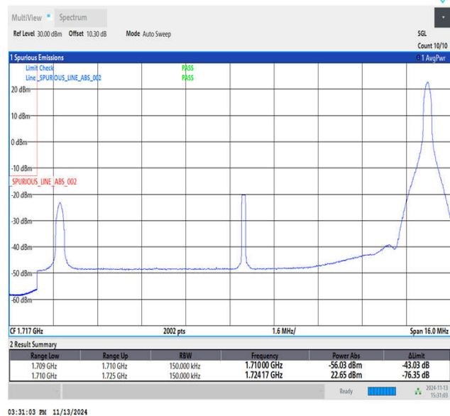
Band4_15MHz_QPSK_20025_1RB#74
