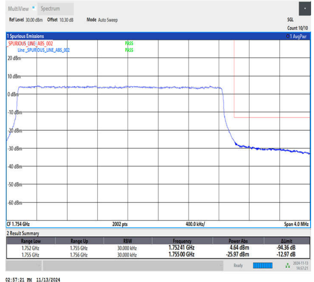
Band4_3MHz_QPSK_20385_15RB#0
