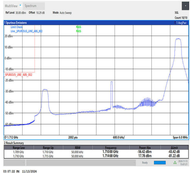
Band4_5MHz_64QAM_19975_1RB#24
