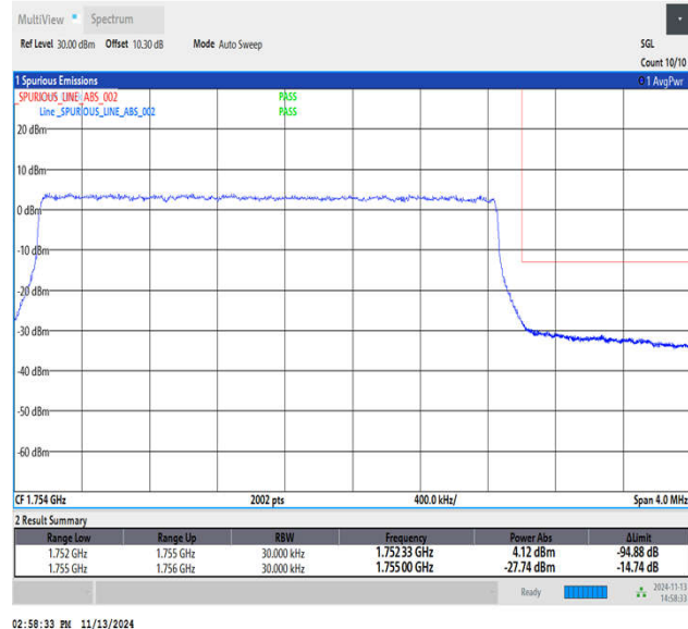
Band4_3MHz_64QAM_20385_15RB#0
