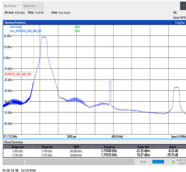
Band4_5MHz_QPSK_19975_1RB#0
