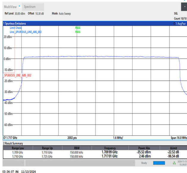
Band4_15MHz_64QAM_20025_75RB#0
