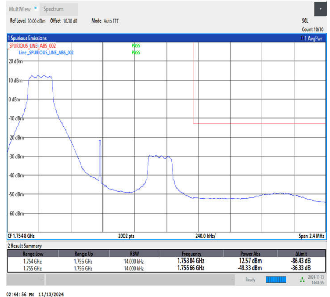
Band4_1.4MHz_64QAM_20393_1RB#0
