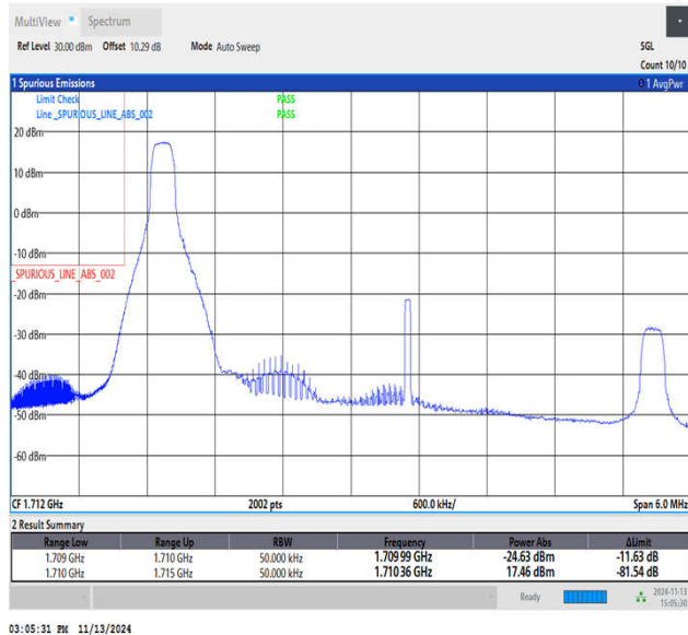
Band4_5MHz_64QAM_19975_1RB#0
