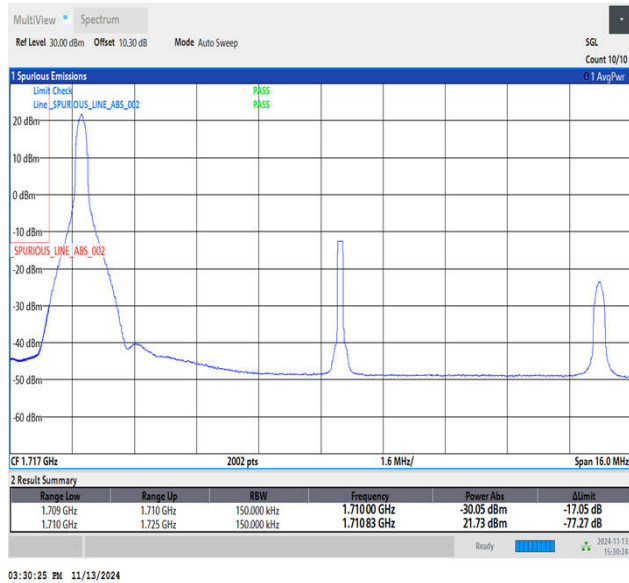
Band4_15MHz_64QAM_20025_1RB#0
