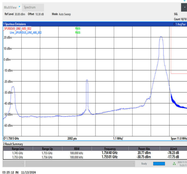
Band4_10MHz_16QAM_20350_1RB#49
