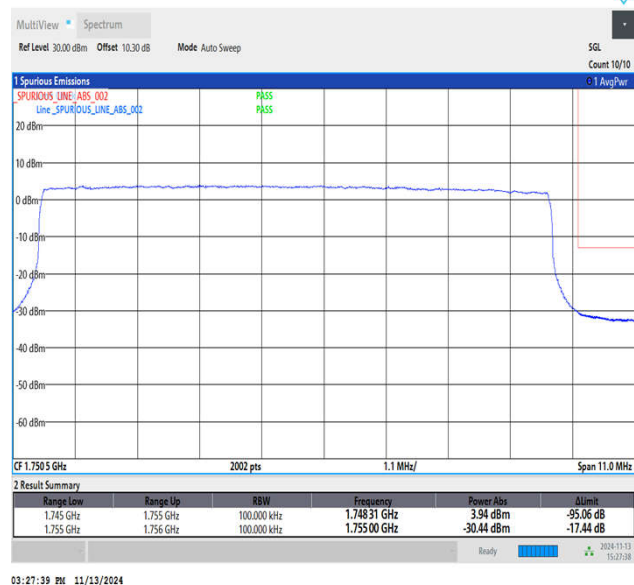
Band4_10MHz_64QAM_20350_50RB#0
