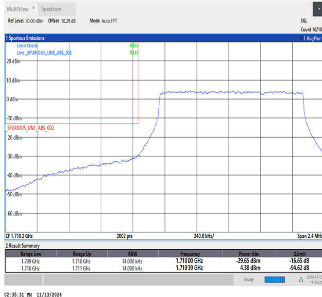
Band4_1.4MHz_64QAM_19957_6RB#0
