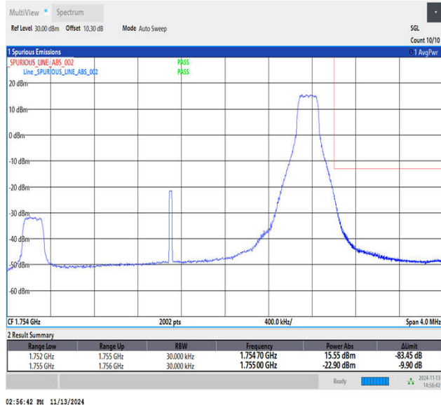
Band4_3MHz_64QAM_20385_1RB#14
