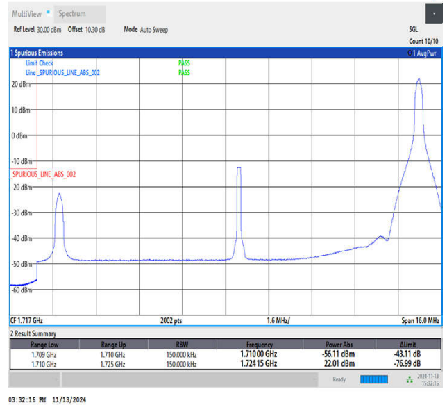
Band4_15MHz_64QAM_20025_1RB#74
