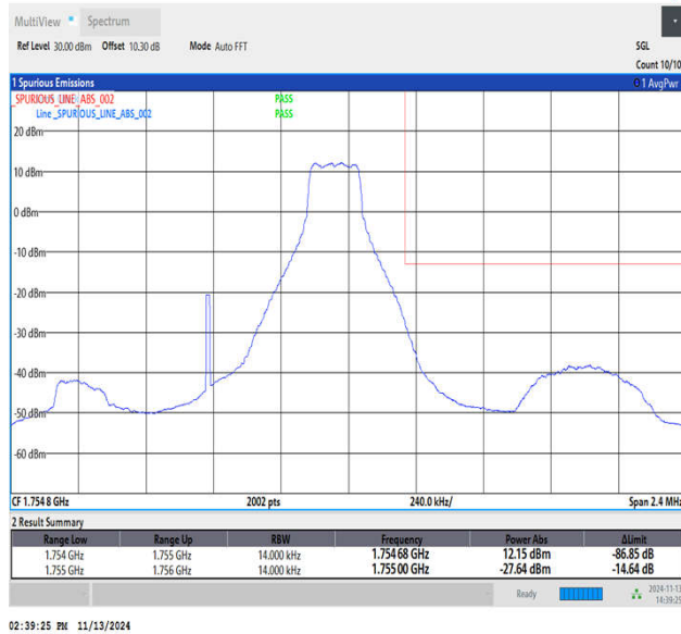
Band4_1.4MHz_64QAM_20393_1RB#5
