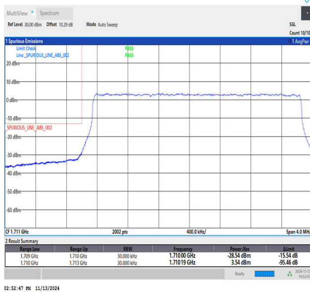
Band4_3MHz_64QAM_19965_15RB#0
