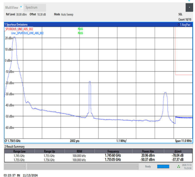
Band4_10MHz_64QAM_20350_1RB#0
