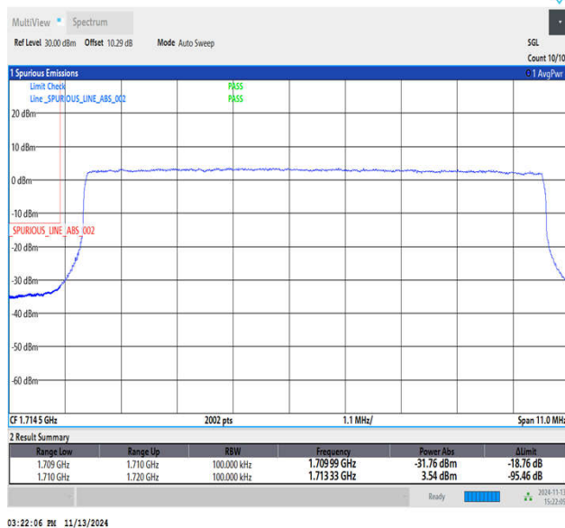
Band4_10MHz_64QAM_20000_50RB#0
