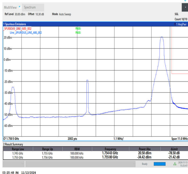
Band4_10MHz_64QAM_20350_1RB#49
