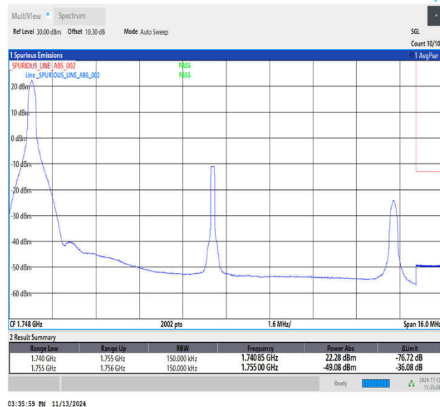
Band4_15MHz_64QAM_20325_1RB#0
