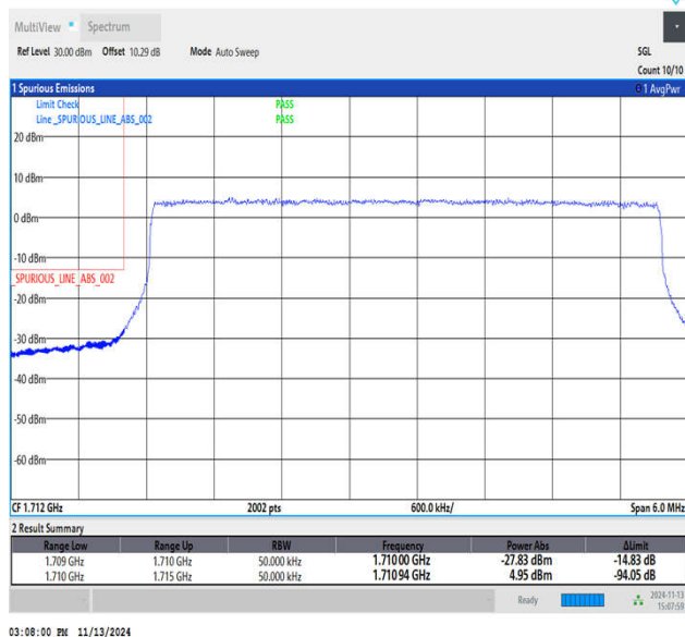
Band4_5MHz_QPSK_19975_25RB#0
