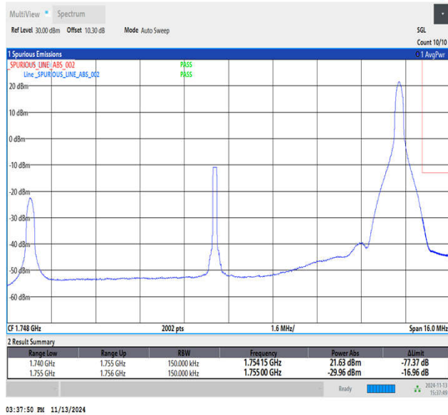
Band4_15MHz_64QAM_20325_1RB#74
