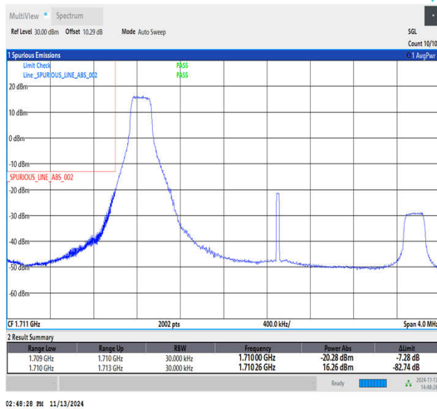
Band4_3MHz_16QAM_19965_1RB#0
