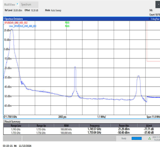
Band4_10MHz_16QAM_20350_1RB#0
