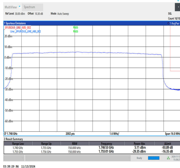
Band4_15MHz_QPSK_20325_75RB#0
