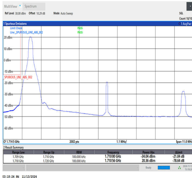
Band4_10MHz_64QAM_20000_1RB#0
