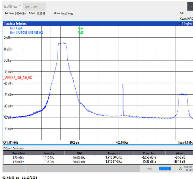
Band4_3MHz_64QAM_19965_1RB#0
