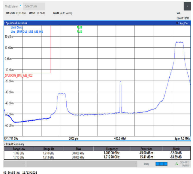
Band4_3MHz_64QAM_19965_1RB#14
