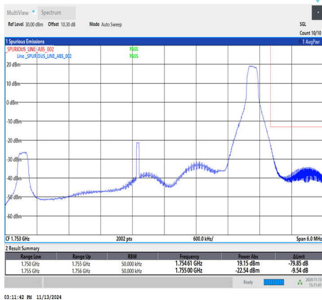
Band4_5MHz_QPSK_20375_1RB#24
