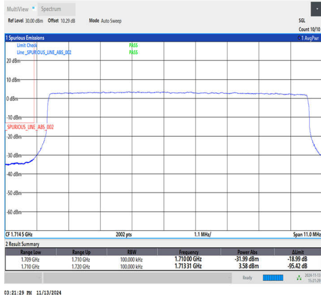
Band4_10MHz_16QAM_20000_50RB#0
