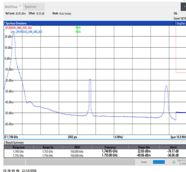
Band4_15MHz_QPSK_20325_1RB#0
