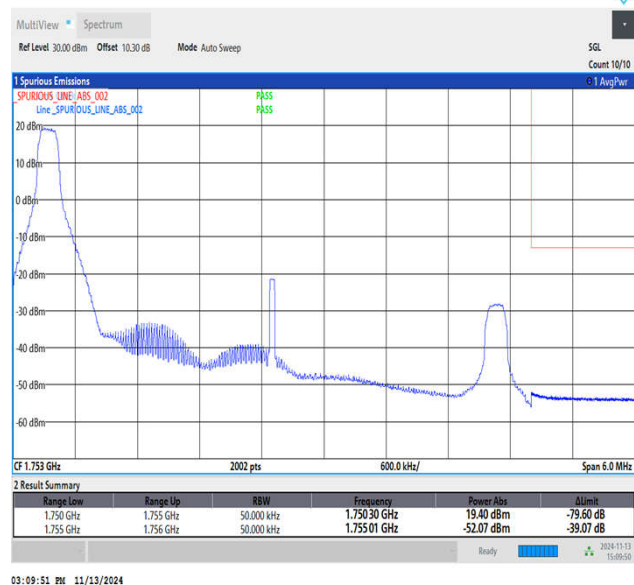
Band4_5MHz_QPSK_20375_1RB#0
