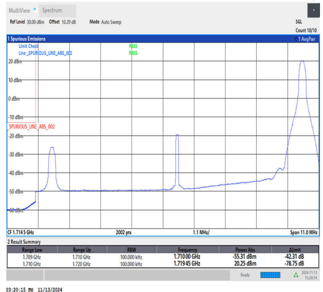
Band4_10MHz_64QAM_20000_1RB#49
