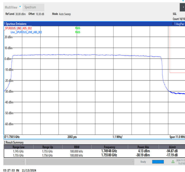
Band4_10MHz_16QAM_20350_50RB#0
