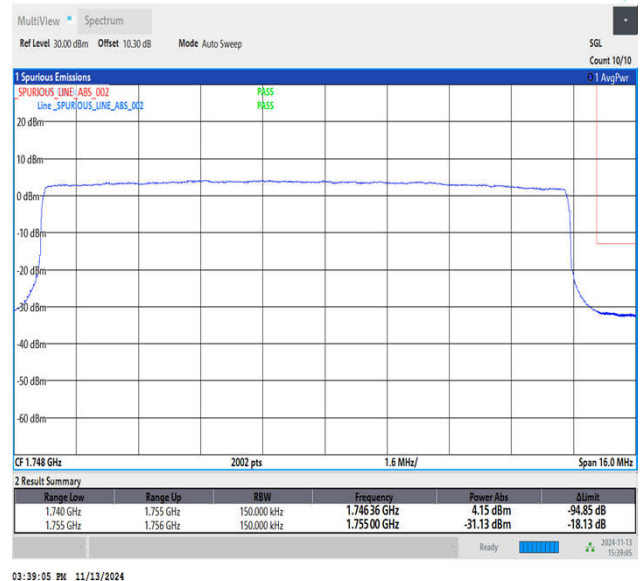
Band4_15MHz_16QAM_20325_75RB#0
