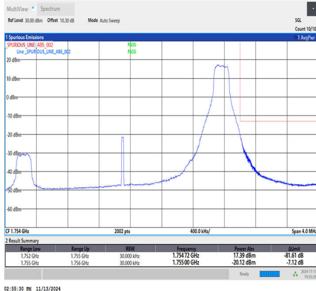
Band4_3MHz_QPSK_20385_1RB#14
