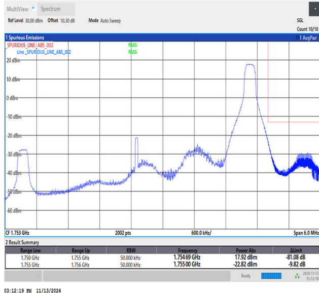
Band4_5MHz_16QAM_20375_1RB#24
