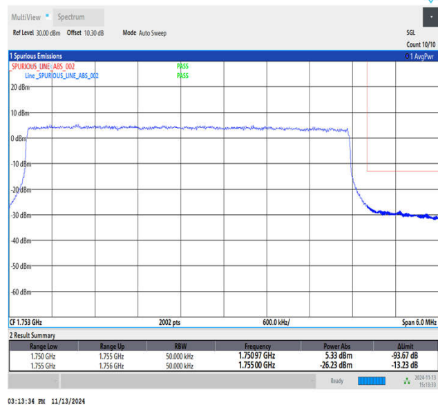
Band4_5MHz_QPSK_20375_25RB#0
