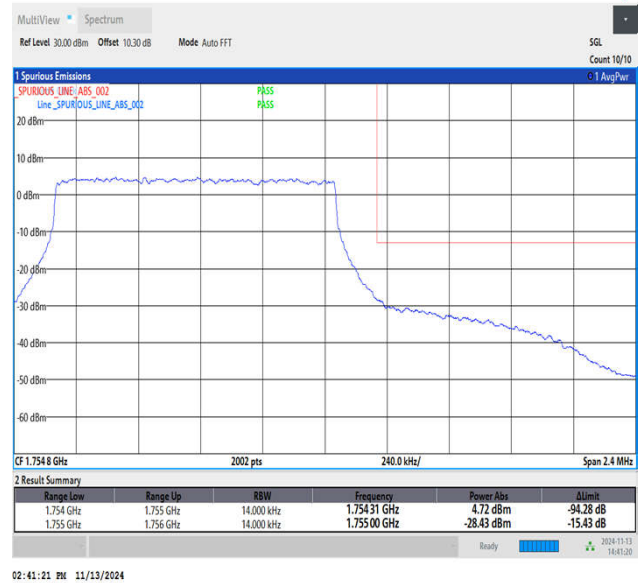
Band4_1.4MHz_64QAM_20393_6RB#0
