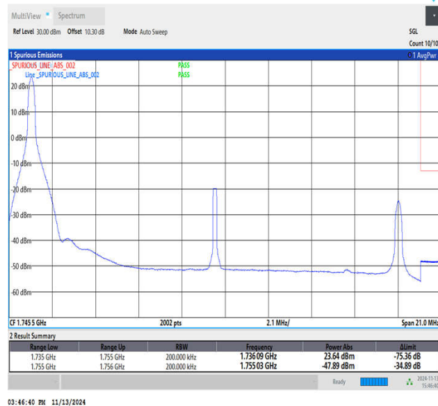
Band4_20MHz_QPSK_20300_1RB#0
