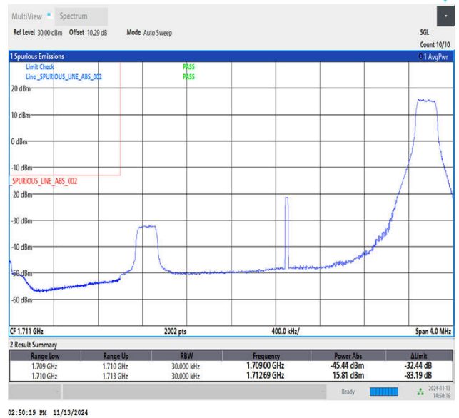
Band4_3MHz_16QAM_19965_1RB#14
