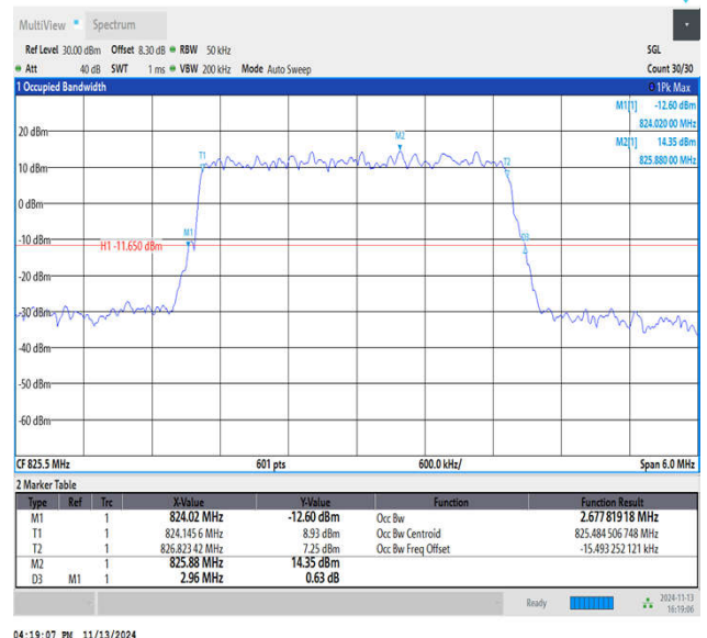
Band5-3MHz-QPSK-20415-15RB#0-PASS
