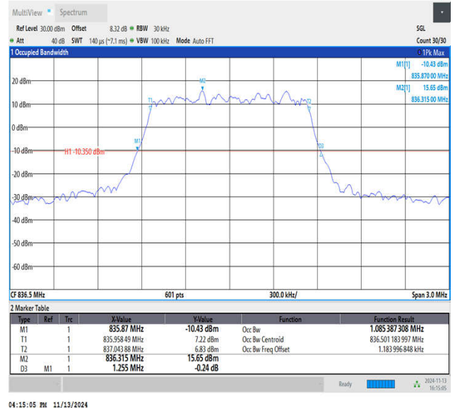
Band5-1.4MHz-64QAM-20525-6RB#0-PASS
