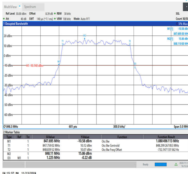
Band5-1.4MHz-64QAM-20643-6RB#0-PASS
