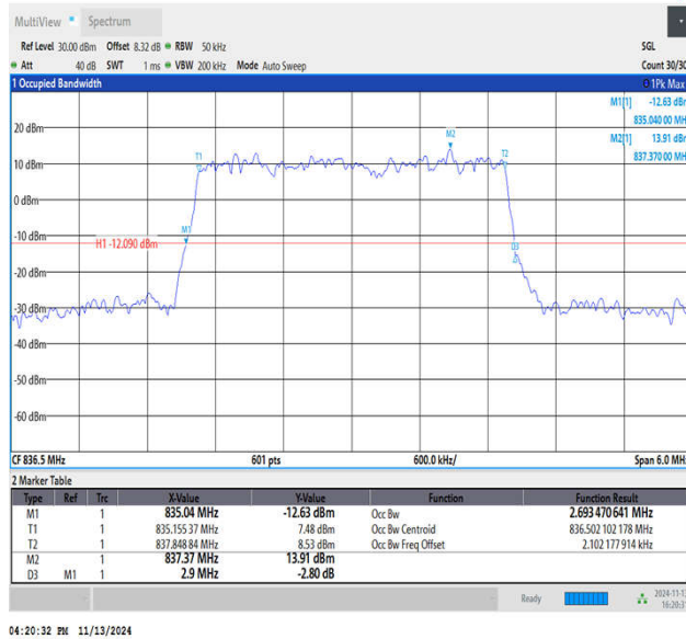
Band5-3MHz-64QAM-20525-15RB#0-PASS
