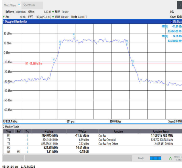
Band5-1.4MHz-64QAM-20407-6RB#0-PASS
