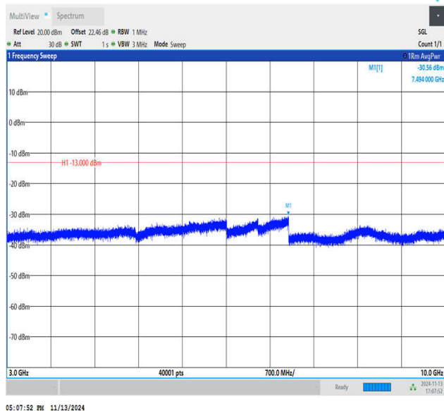
Band5_1.4MHz_QPSK_20407_1RB#0_3000~10000_3000~10000
