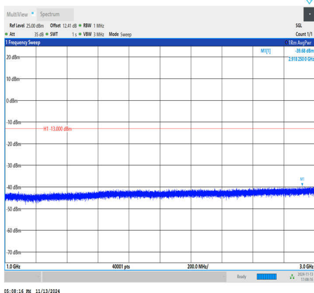
Band5_1.4MHz_QPSK_20525_1RB#0_1000~3000_1000~3000
