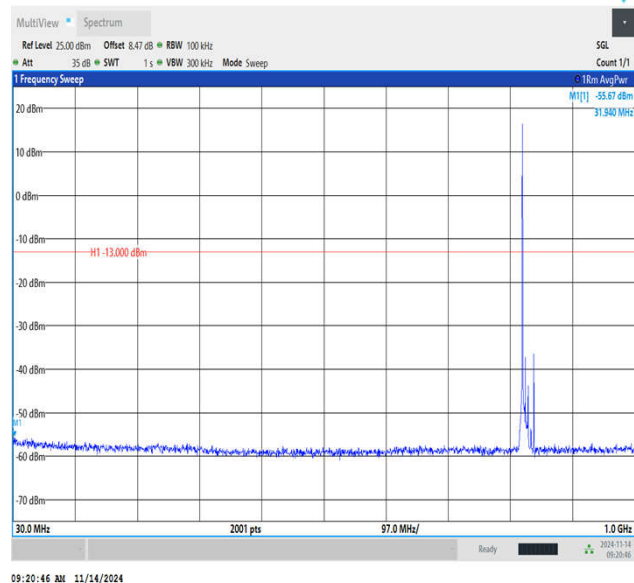
Band5_10MHz_QPSK_20450_1RB#0_30~1000_30~1000
