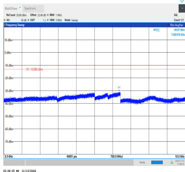
Band5_1.4MHz_QPSK_20525_1RB#0_3000~10000_3000~10000
