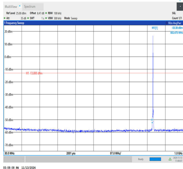
Band5_1.4MHz_QPSK_20525_1RB#0_30~1000_30~1000
