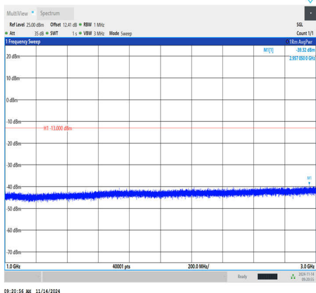
Band5_10MHz_QPSK_20450_1RB#0_1000~3000_1000~3000
