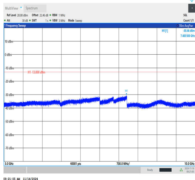
Band5_10MHz_QPSK_20450_1RB#0_3000~10000_3000~10000
