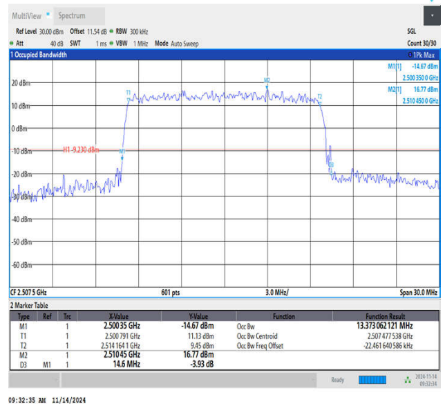
Band7-15MHz-16QAM-20825-75RB#0-PASS
