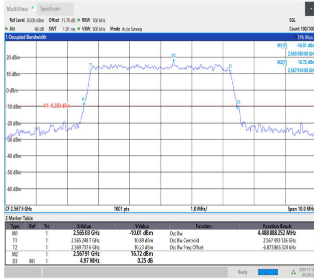
Band7-5MHz-QPSK-21425-25RB#0-PASS
