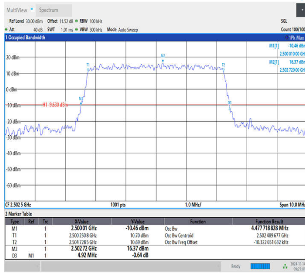
Band7-5MHz-64QAM-20775-25RB#0-PASS
