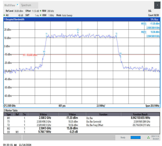
Band7-10MHz-64QAM-20800-50RB#0-PASS
