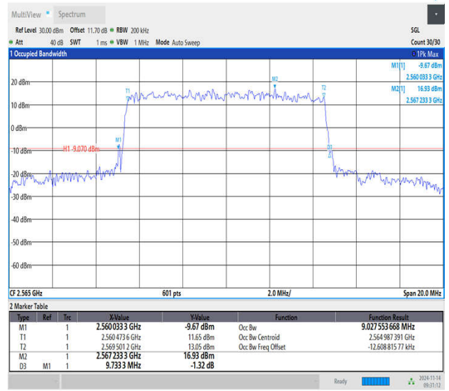
Band7-10MHz-QPSK-21400-50RB#0-PASS
