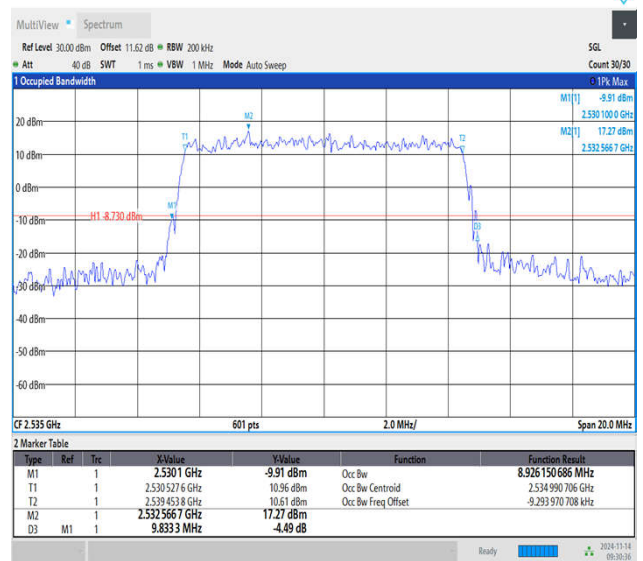
Band7-10MHz-16QAM-21100-50RB#0-PASS
