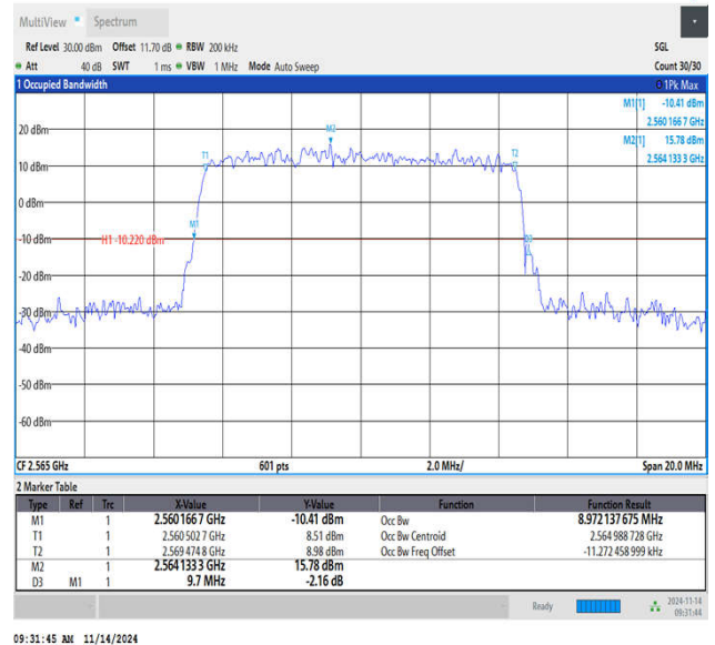
Band7-10MHz-64QAM-21400-50RB#0-PASS
