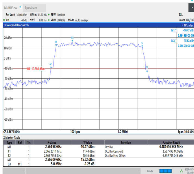
Band7-5MHz-64QAM-21425-25RB#0-PASS
