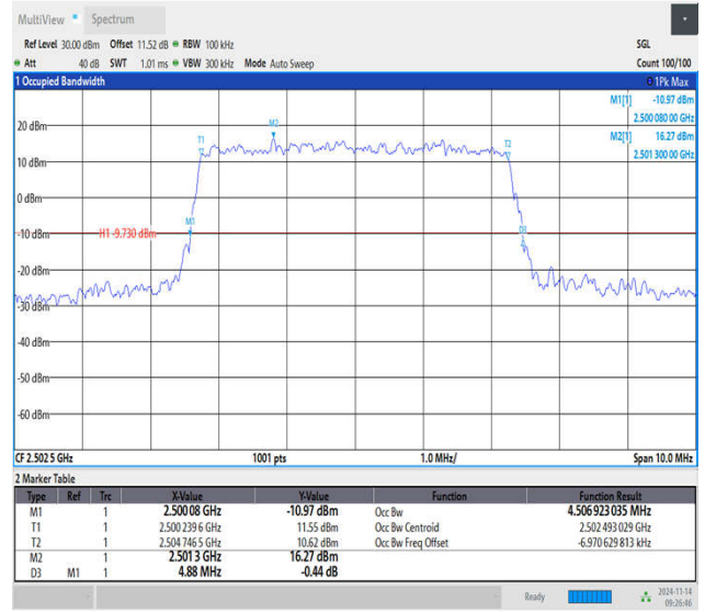
Band7-5MHz-16QAM-20775-25RB#0-PASS
