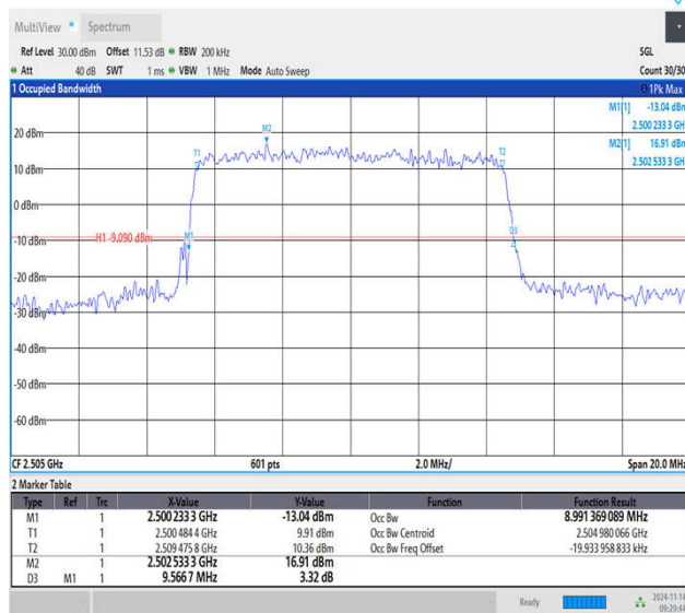
Band7-10MHz-16QAM-20800-50RB#0-PASS
