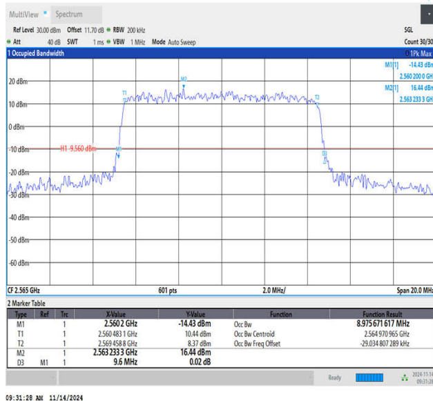
Band7-10MHz-16QAM-21400-50RB#0-PASS
