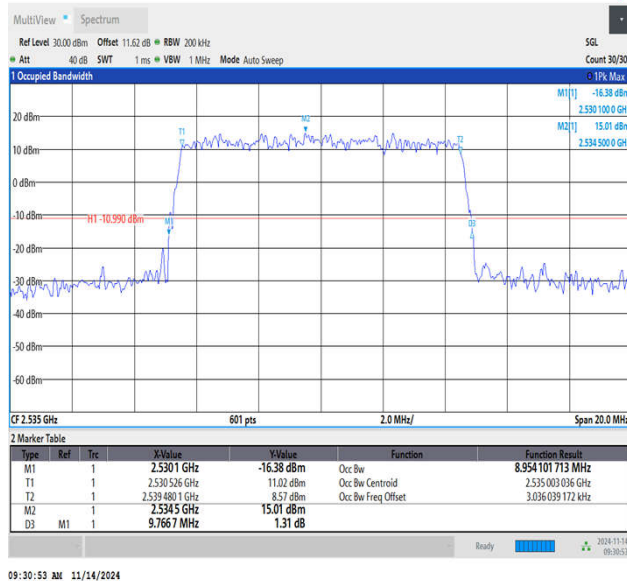
Band7-10MHz-64QAM-21100-50RB#0-PASS
