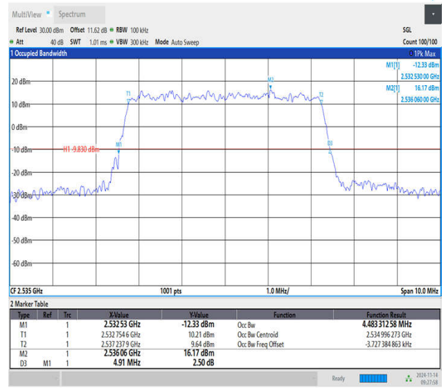
Band7-5MHz-64QAM-21100-25RB#0-PASS
