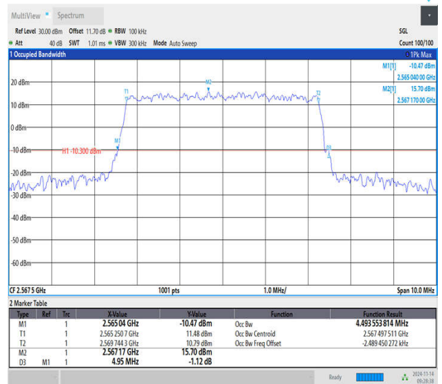
Band7-5MHz-16QAM-21425-25RB#0-PASS
