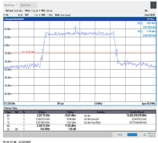
Band7-15MHz-QPSK-21100-75RB#0-PASS
