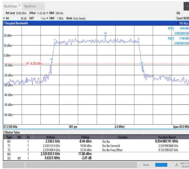
Band7-10MHz-QPSK-21100-50RB#0-PASS
