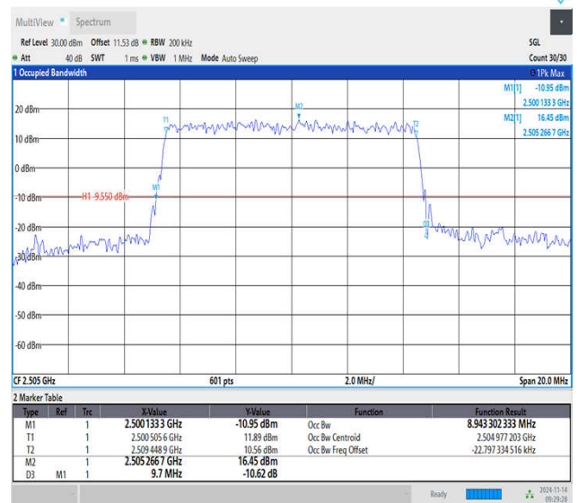
Band7-10MHz-QPSK-20800-50RB#0-PASS
