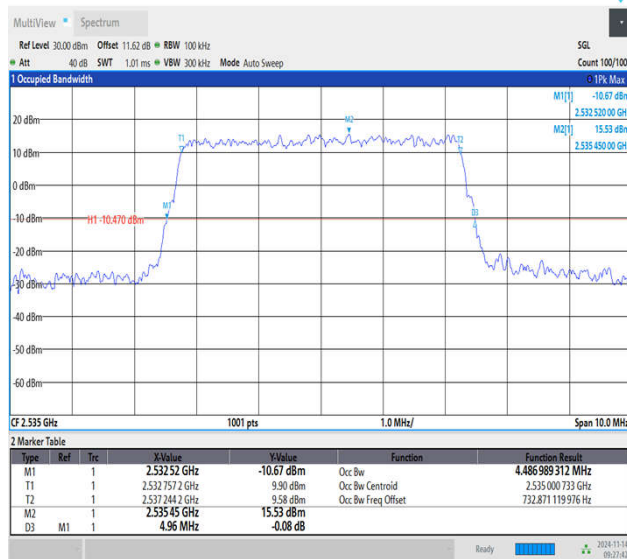
Band7-5MHz-16QAM-21100-25RB#0-PASS
