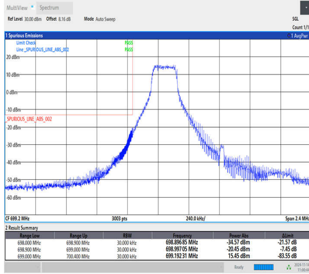
Band12_1.4MHz_16QAM_23017_1RB#0
