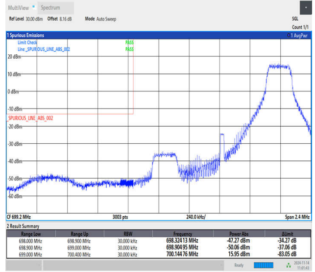
Band12_1.4MHz_16QAM_23017_1RB#5
