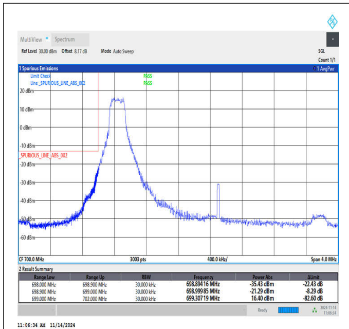
Band12_3MHz_QPSK_23025_1RB#0
