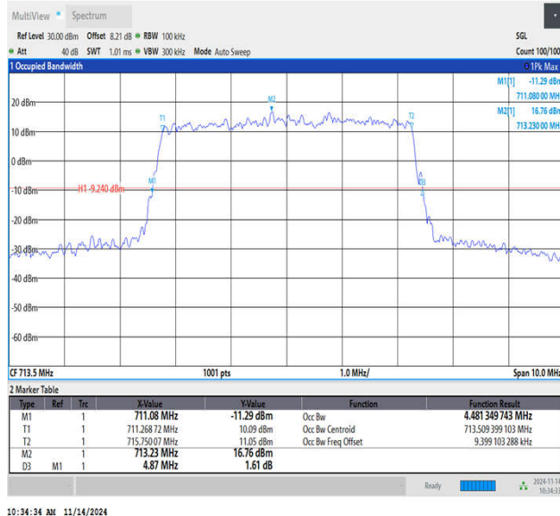
Band12-5MHz-64QAM-23155-25RB#0-PASS
