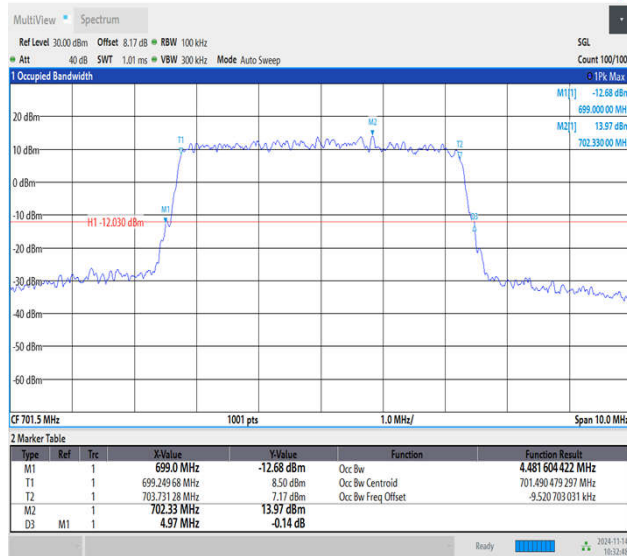
Band12-5MHz-64QAM-23035-25RB#0-PASS
