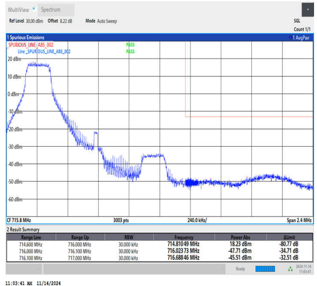
Band12_1.4MHz_16QAM_23173_1RB#0
