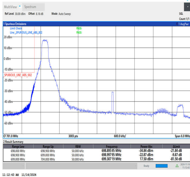
Band12_5MHz_QPSK_23035_1RB#0
