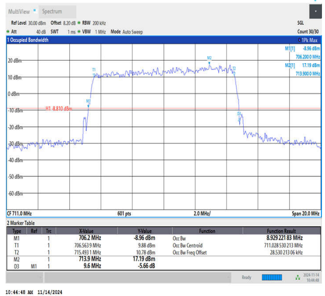
Band12-10MHz-QPSK-23130-50RB#0-PASS
