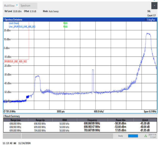
Band12_5MHz_QPSK_23035_1RB#24
