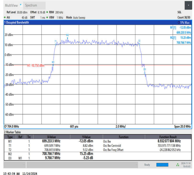
Band12-10MHz-QPSK-23060-50RB#0-PASS
