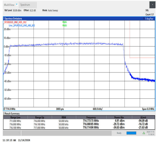
Band12_5MHz_64QAM_23155_25RB#0
