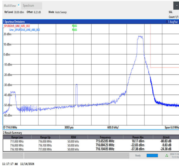
Band12_5MHz_64QAM_23155_1RB#24
