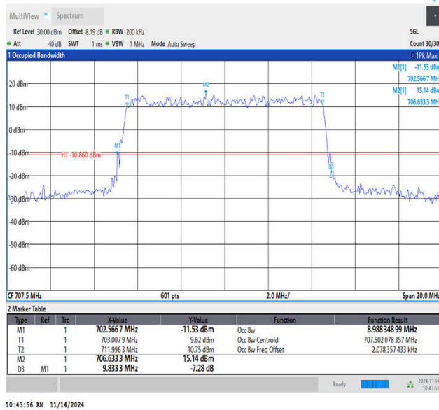
Band12-10MHz-QPSK-23095-50RB#0-PASS
