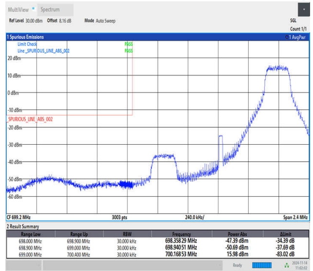
Band12_1.4MHz_64QAM_23017_1RB#5
