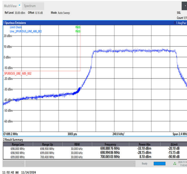
Band12_1.4MHz_16QAM_23017_6RB#0
