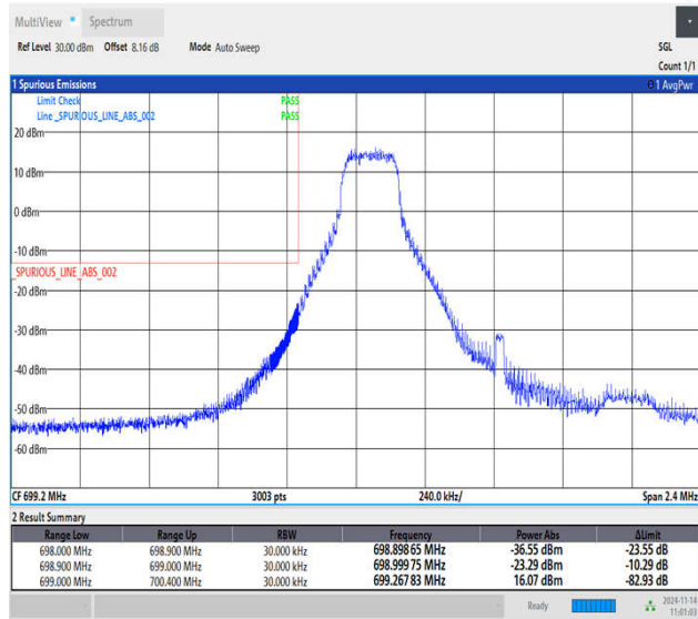
Band12_1.4MHz_64QAM_23017_1RB#0
