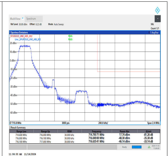
Band12_1.4MHz_64QAM_23173_1RB#0
