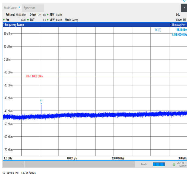
Band12_1.4MHz_QPSK_23095_1RB#0_1000~3000_1000~3000 3000
