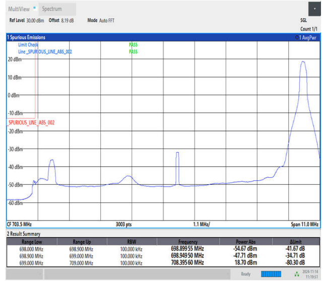
Band12_10MHz_QPSK_23060_1RB#49
