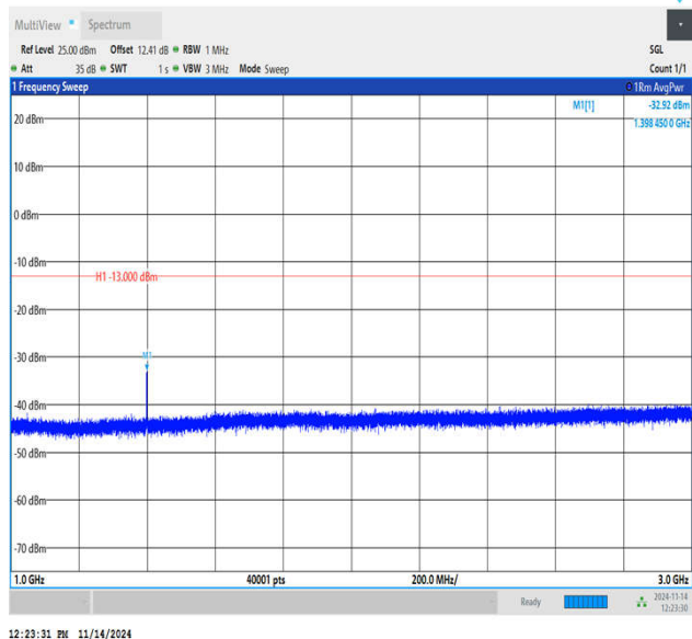
Band12_3MHz_QPSK_23025_1RB#0_1000~3000_1000~30 00
