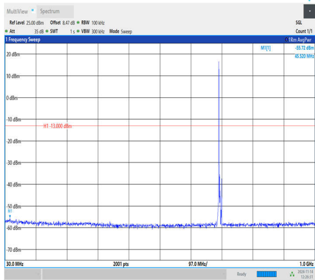
Band12_5MHz_QPSK_23035_1RB#0_30~1000_30~1000
