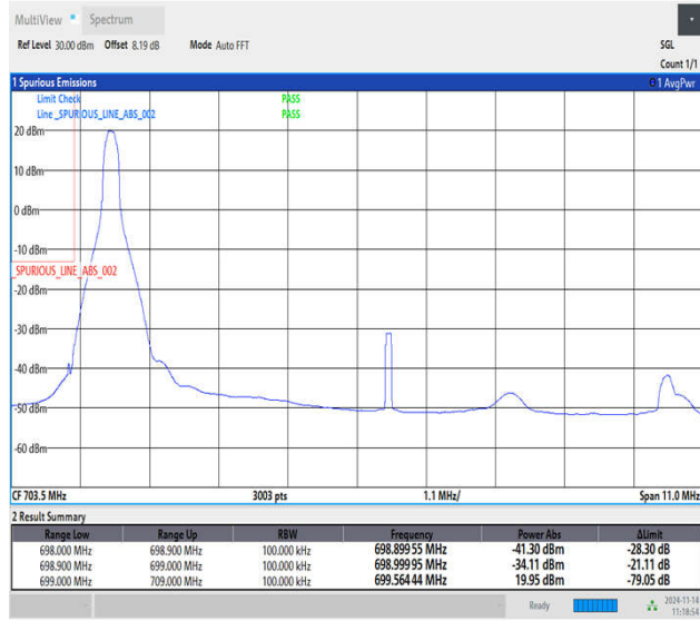
Band12_10MHz_QPSK_23060_1RB#0
