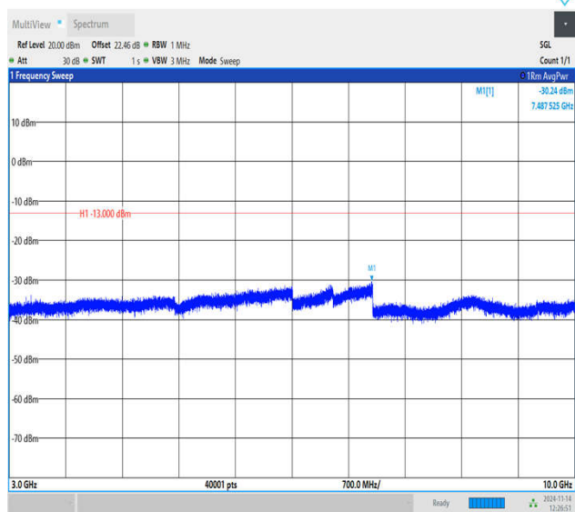
Band12_5MHz_QPSK_23035_1RB#0_3000~10000_3000~10000
