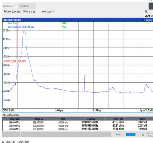
Band12_10MHz_16QAM_23060_1RB#0
