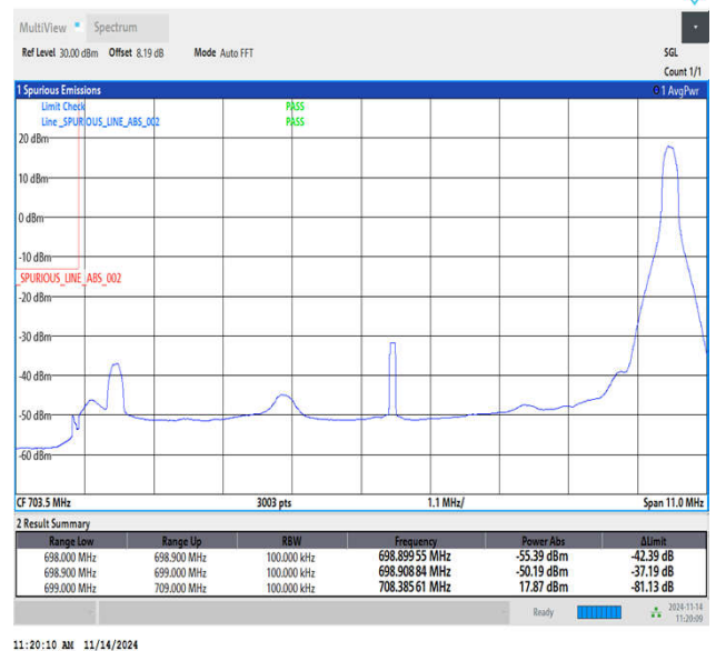
Band12_10MHz_16QAM_23060_1RB#49
