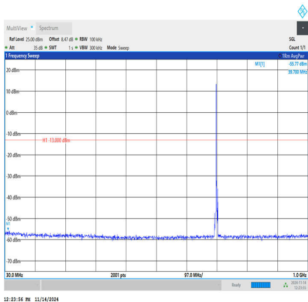
Band12_3MHz_QPSK_23025_1RB#0_1000~3000_1000~30 00
