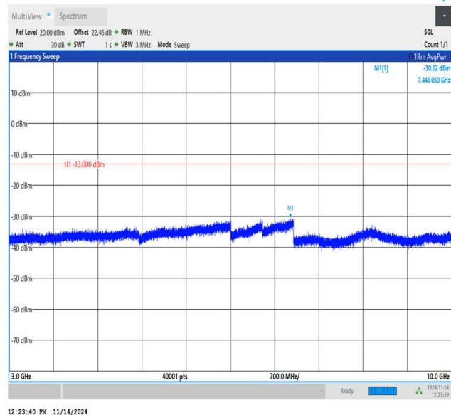
Band12_3MHz_QPSK_23025_1RB#0_3000~10000_3000~1 0000
