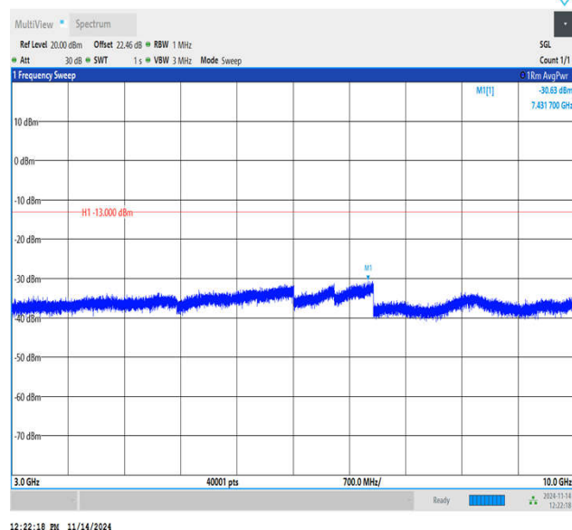
Band12_1.4MHz_QPSK_23095_1RB#0_3000~10000_3000~10000 ~10000
