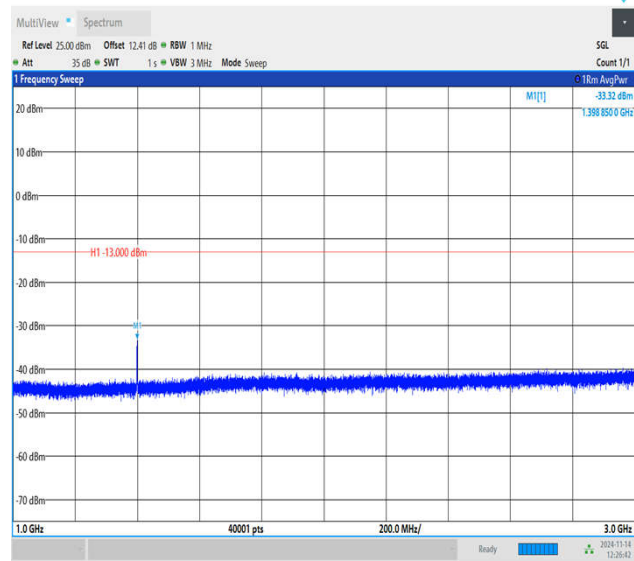
Band12_5MHz_QPSK_23035_1RB#0_1000~3000_1000~3000
