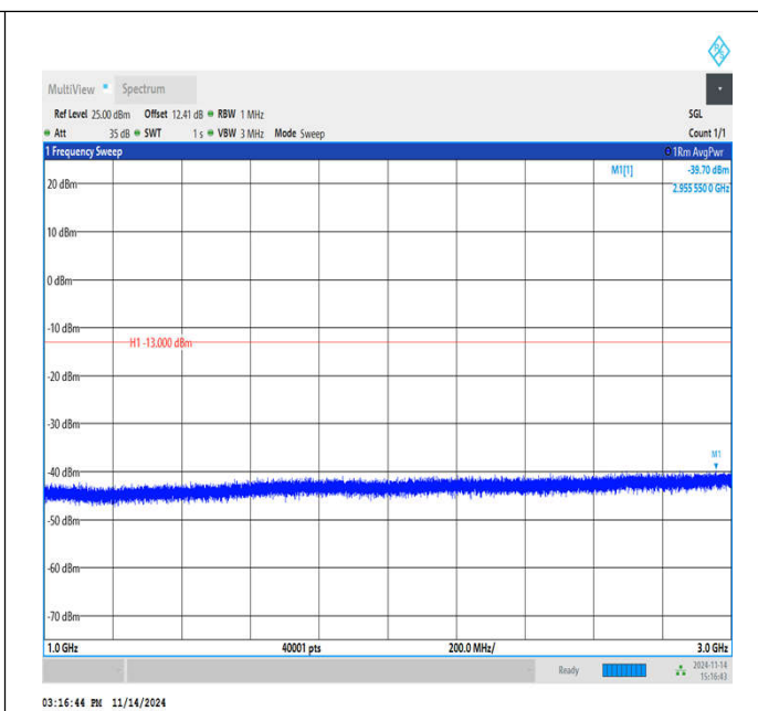
Band13_10MHz_QPSK_23230_1RB#0_1000~3000_1000~3000
