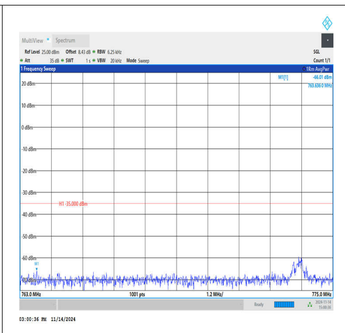
Band13_5MHz_QPSK_23255_1RB#0_763~775_763~775
