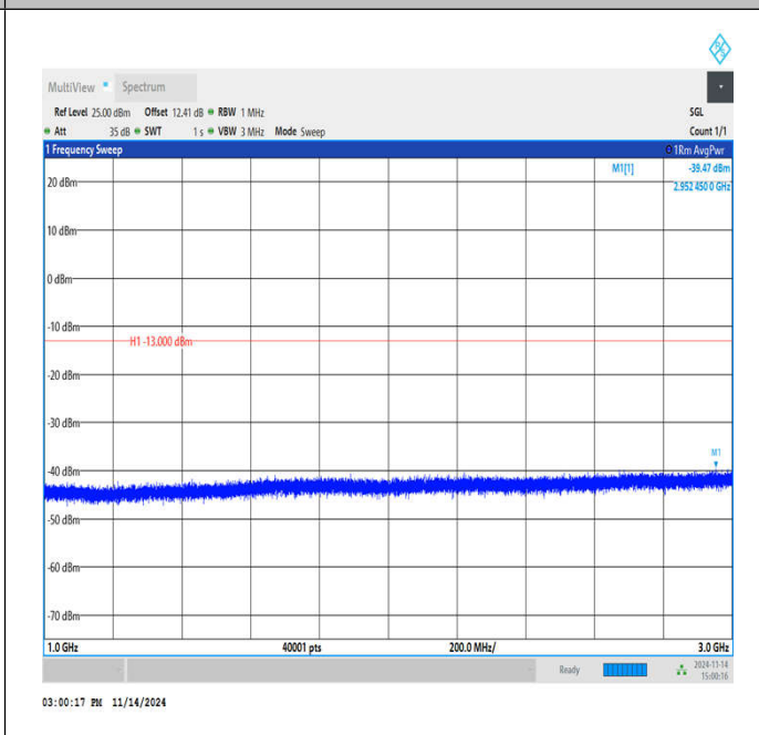
Band13_5MHz_QPSK_23255_1RB#0_1000~3000_1000~3000
