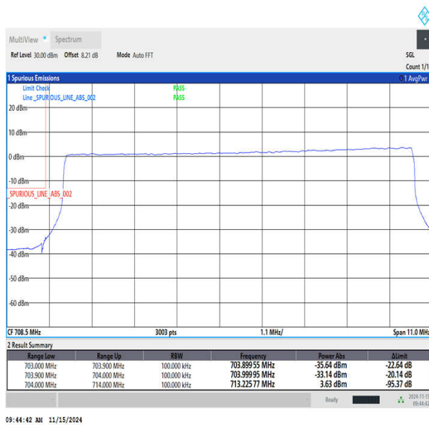
Band17_10MHz_64QAM_23780_50RB#0
