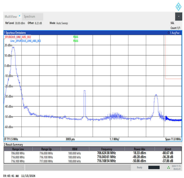
Band17_10MHz_64QAM_23800_1RB#0
