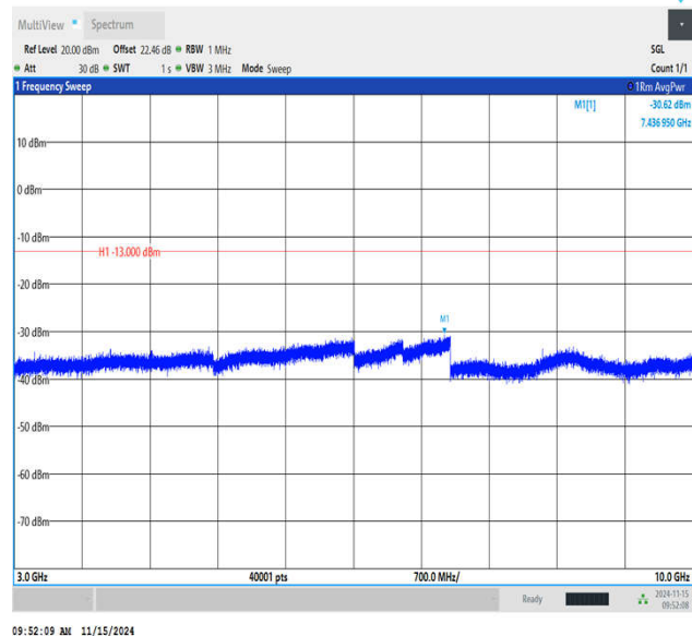
Band17_5MHz_QPSK_23790_1RB#0_3000~10000_3000~1 0000
