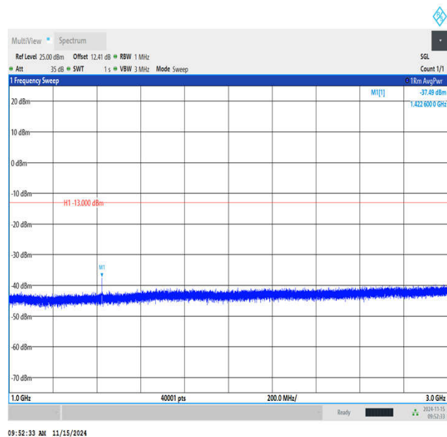
Band17_5MHz_QPSK_23825_1RB#0_1000~3000_1000~30 00
