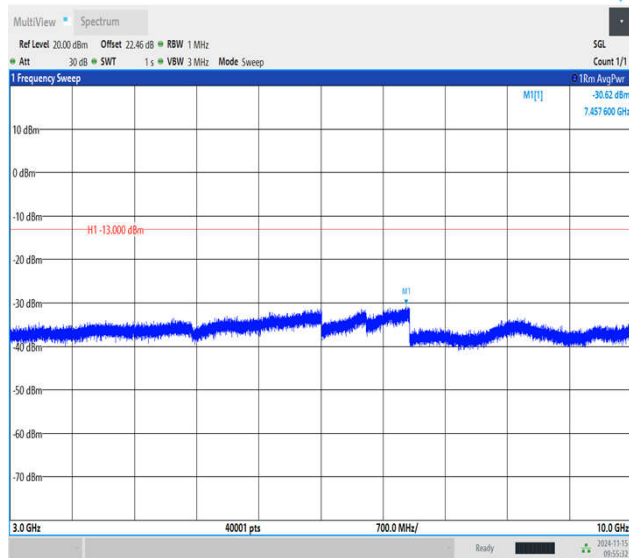
Band17_10MHz_QPSK_23790_1RB#0_3000~10000_3000~10000
