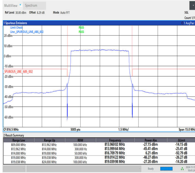
Band26_5MHz_QPSK_26715_25RB#0
