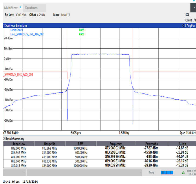
Band26_5MHz_16QAM_26715_25RB#0
