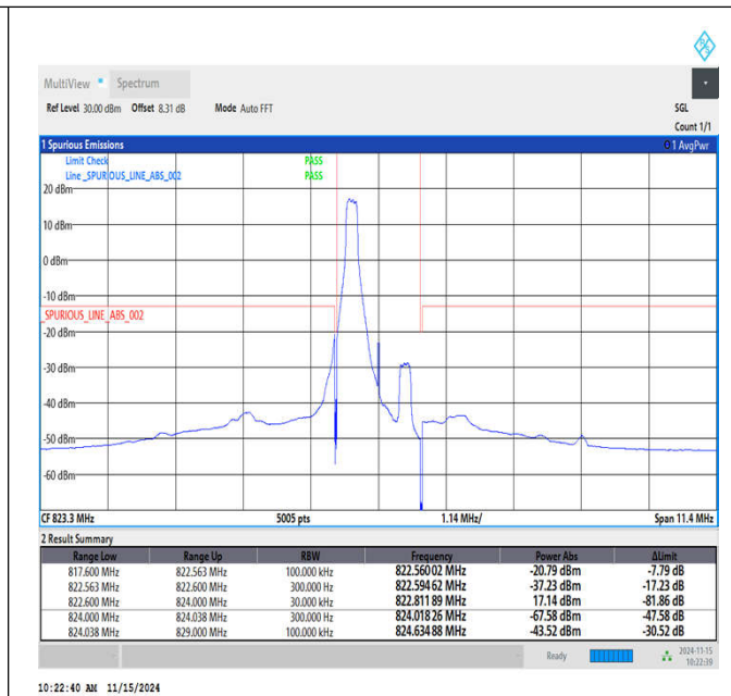
Band26_1.4MHz_QPSK_26783_1RB#0
