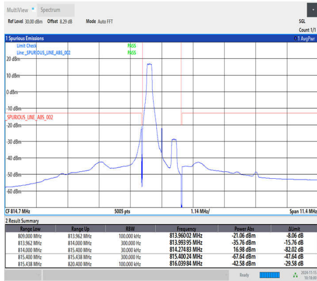
Band26_1.4MHz_64QAM_26697_1RB#0
