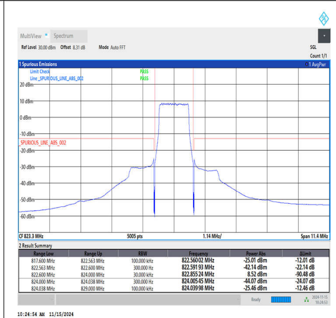
Band26_1.4MHz_QPSK_26783_6RB#0
