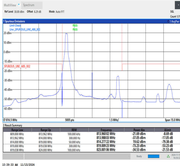
Band26_5MHz_16QAM_26715_1RB#0
