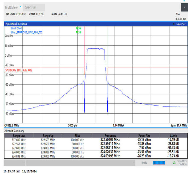
Band26_1.4MHz_64QAM_26783_6RB#0
