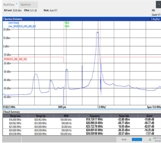
Band26_3MHz_QPSK_26775_1RB#14
