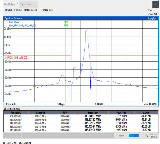
Band26_1.4MHz_16QAM_26697_1RB#5
