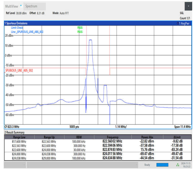
Band26_1.4MHz_64QAM_26783_1RB#0
