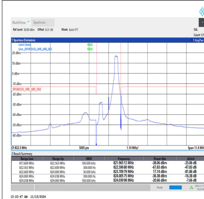
Band26_1.4MHz_QPSK_26783_1RB#5
