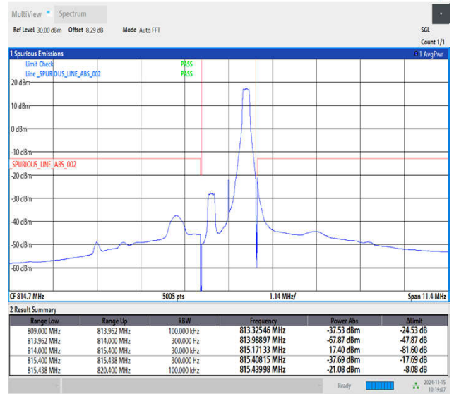
Band26_1.4MHz_64QAM_26697_1RB#5
