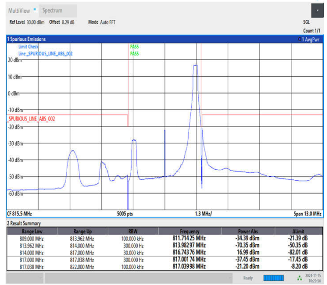
Band26_3MHz_64QAM_26705_1RB#14
