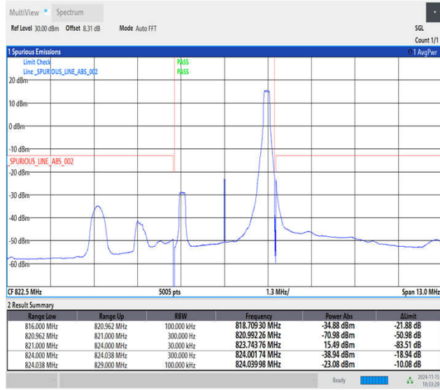
Band26_3MHz_64QAM_26775_1RB#14
