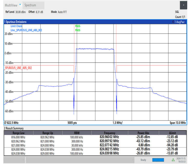
Band26_3MHz_QPSK_26775_15RB#0
