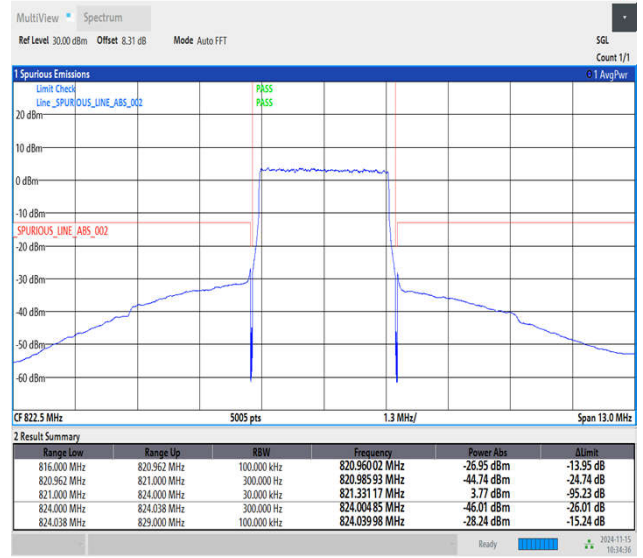
Band26_3MHz_64QAM_26775_15RB#0
