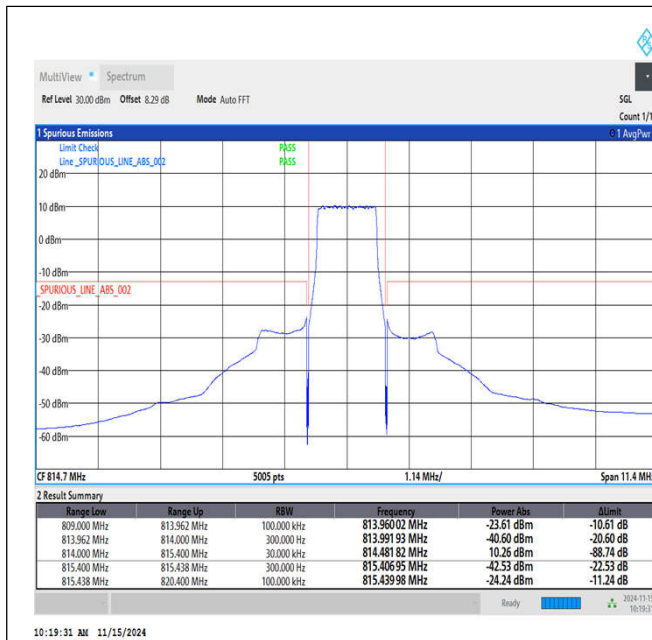
Band26_1.4MHz_QPSK_26697_6RB#0
