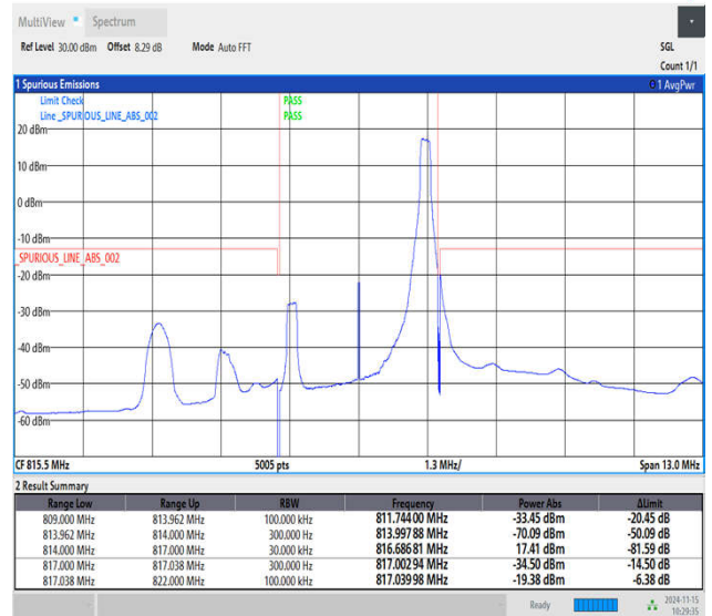
Band26_3MHz_16QAM_26705_1RB#14
