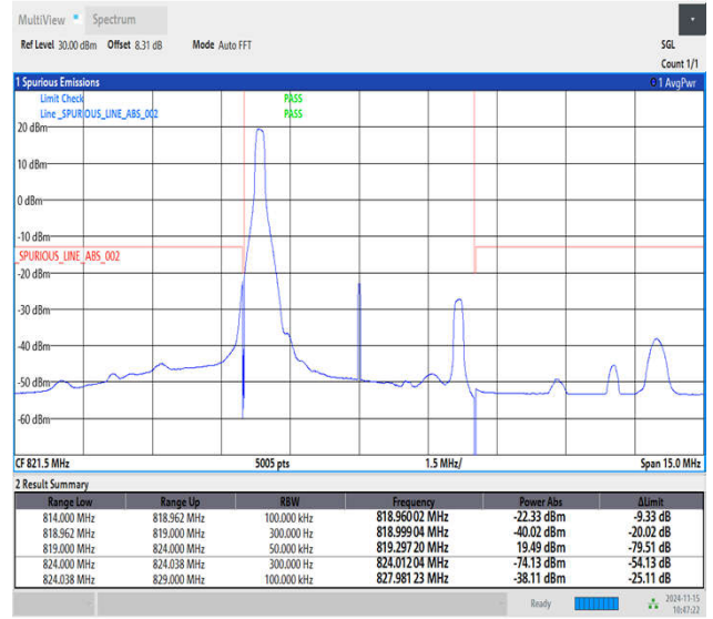
Band26_5MHz_QPSK_26765_1RB#0
