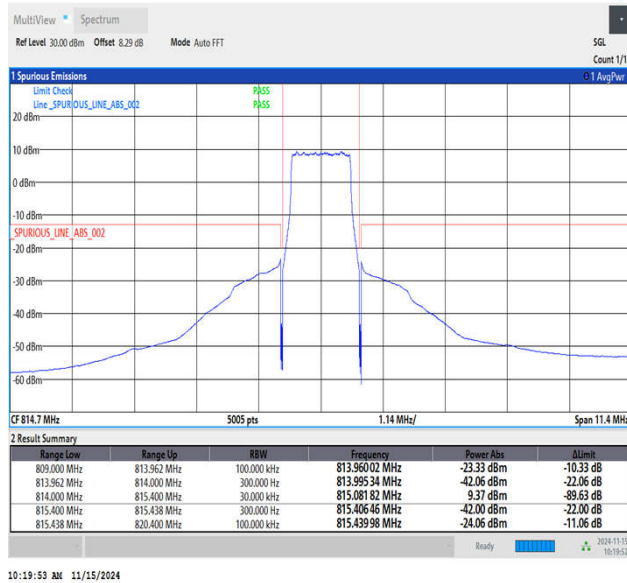
Band26_1.4MHz_16QAM_26697_6RB#0
