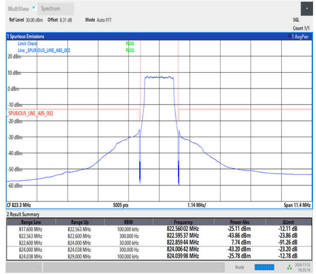
Band26_1.4MHz_16QAM_26783_6RB#0
