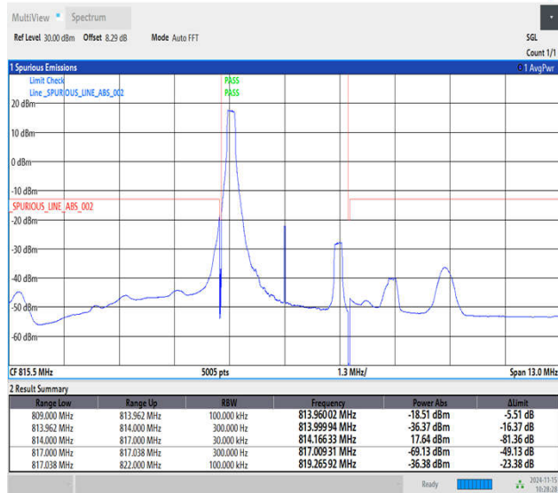
Band26_3MHz_16QAM_26705_1RB#0
