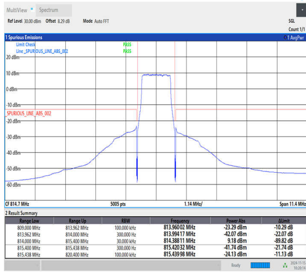
Band26_1.4MHz_64QAM_26697_6RB#0
