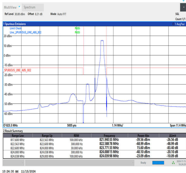
Band26_1.4MHz_64QAM_26783_1RB#5
