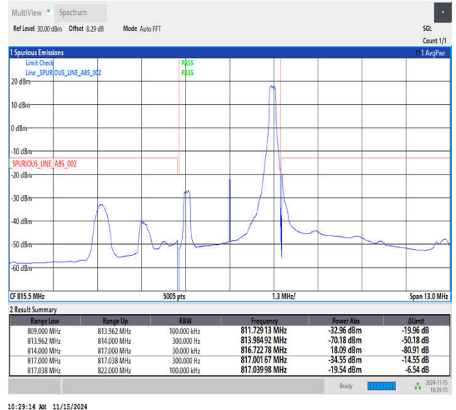
Band26_3MHz_QPSK_26705_1RB#14
