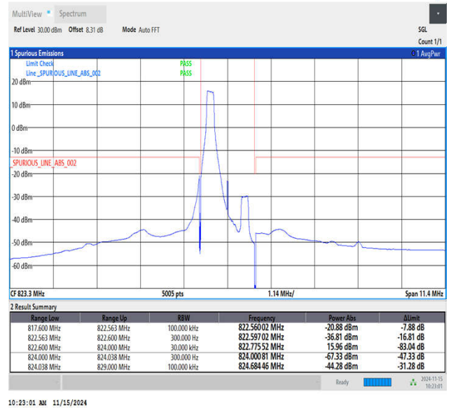
Band26_1.4MHz_16QAM_26783_1RB#0
