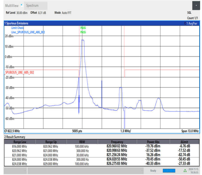
Band26_3MHz_16QAM_26775_1RB#0
