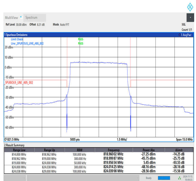
Band26_5MHz_QPSK_26765_1RB#0
