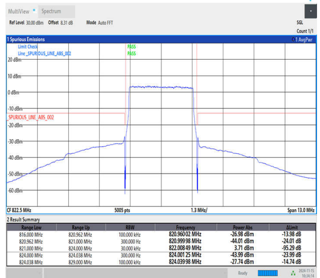
Band26_3MHz_16QAM_26775_15RB#0
