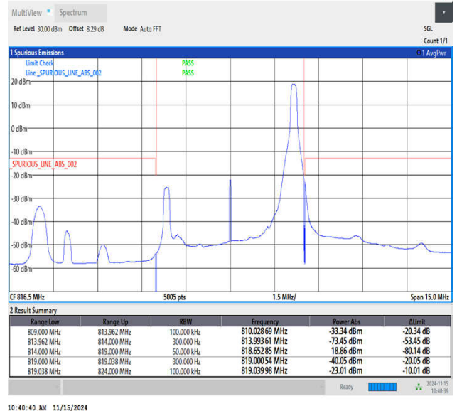
Band26_5MHz_16QAM_26715_1RB#24
