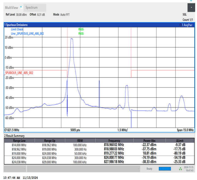
Band26_5MHz_16QAM_26765_1RB#0
