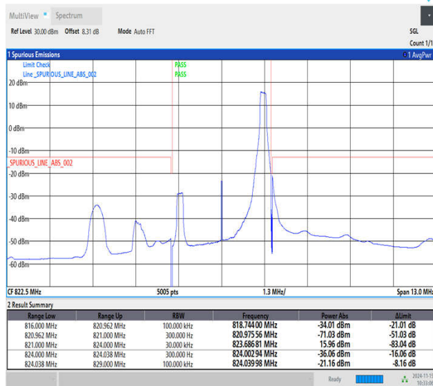
Band26_3MHz_16QAM_26775_1RB#14
