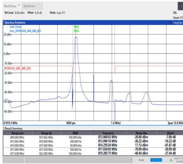
Band26_3MHz_64QAM_26705_1RB#0
