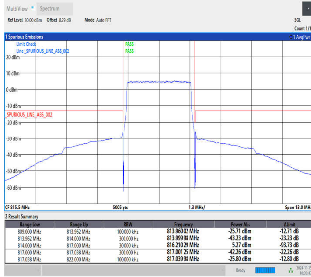
Band26_3MHz_16QAM_26705_15RB#0
