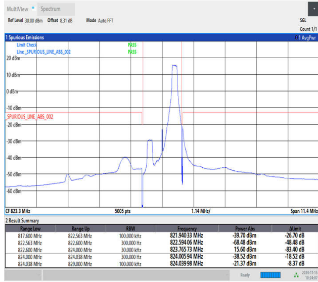
Band26_1.4MHz_16QAM_26783_1RB#5
