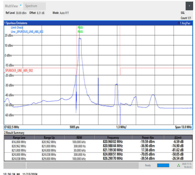
Band26_3MHz_QPSK_26775_1RB#0
