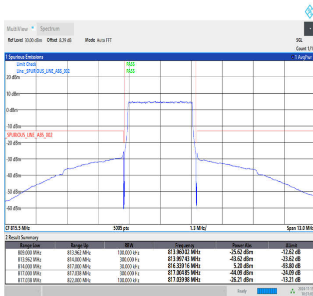
Band26_3MHz_64QAM_26705_1RB#0
