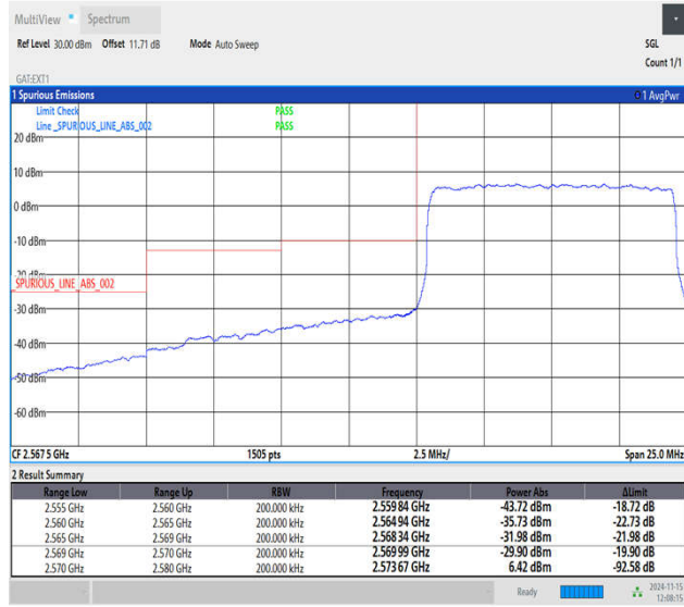
Band38_10MHz_16QAM_37800_50RB#0
