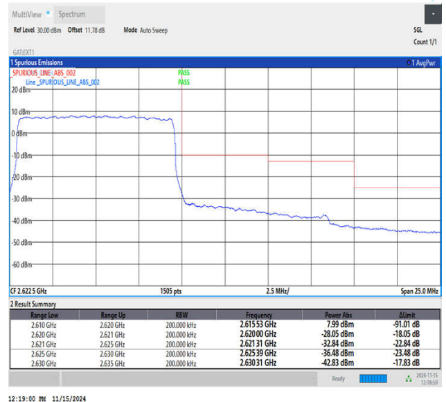
Band38_10MHz_QPSK_38200_50RB#0
