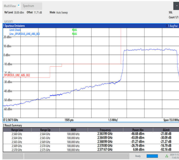
Band38_5MHz_64QAM_37775_25RB#0
