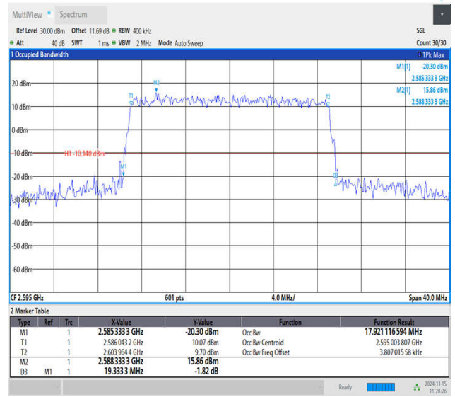
Band38-20MHz-16QAM-38000-100RB#0-PASS
