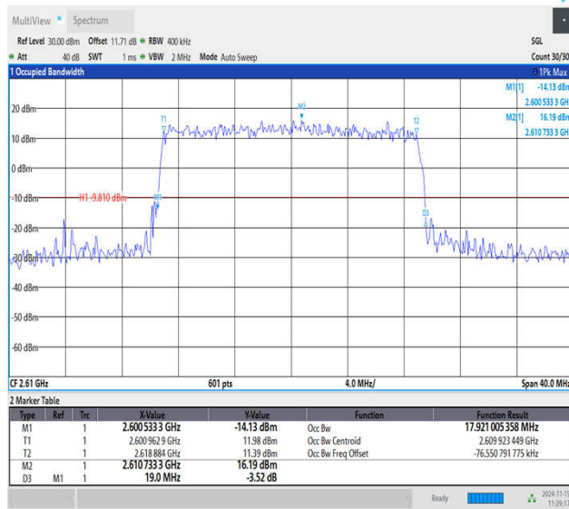
Band38-20MHz-16QAM-38150-100RB#0-PASS
