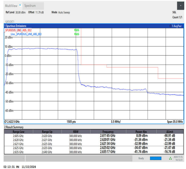
Band38_15MHz_QPSK_38175_75RB#0
