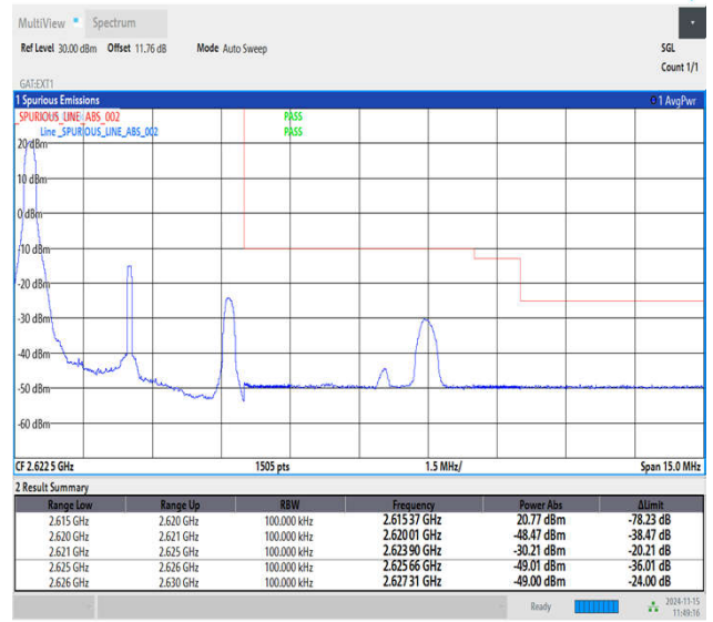
Band38_5MHz_64QAM_38225_1RB#0
