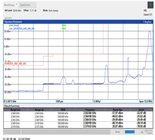
Band38_5MHz_16QAM_37775_1RB#24
