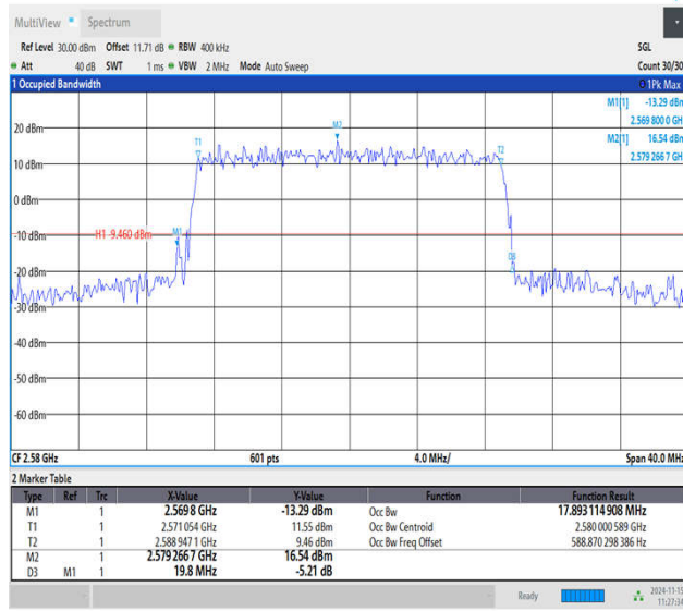
Band38-20MHz-16QAM-37850-100RB#0-PASS
