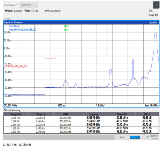
Band38_5MHz_64QAM_37775_1RB#24
