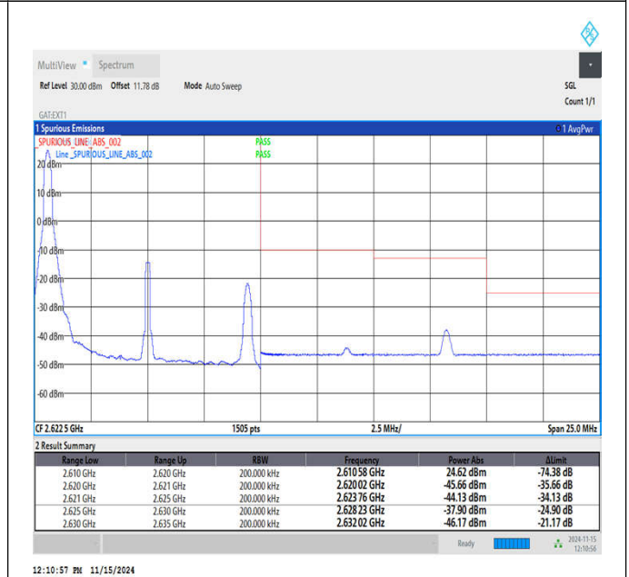
Band38_10MHz_QPSK_38200_1RB#0
