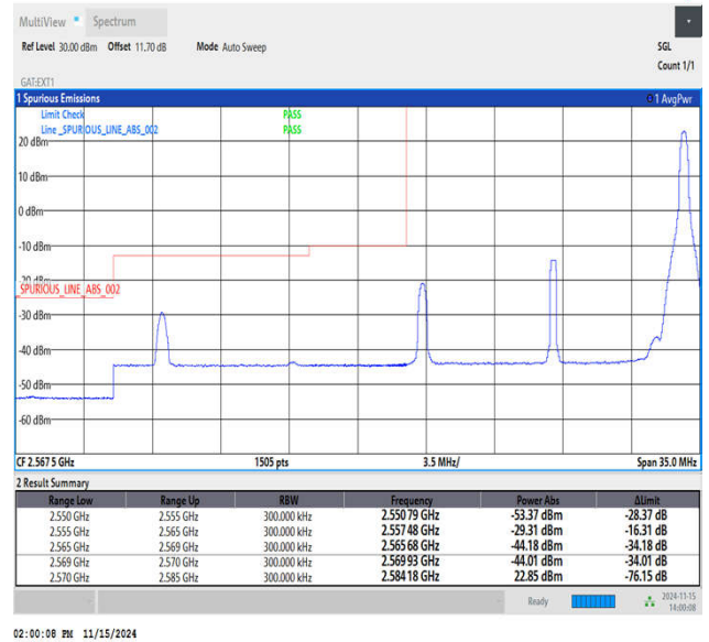
Band38_15MHz_64QAM_37825_1RB#74
