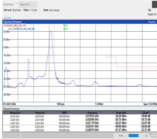
Band38_5MHz_16QAM_38225_1RB#24
