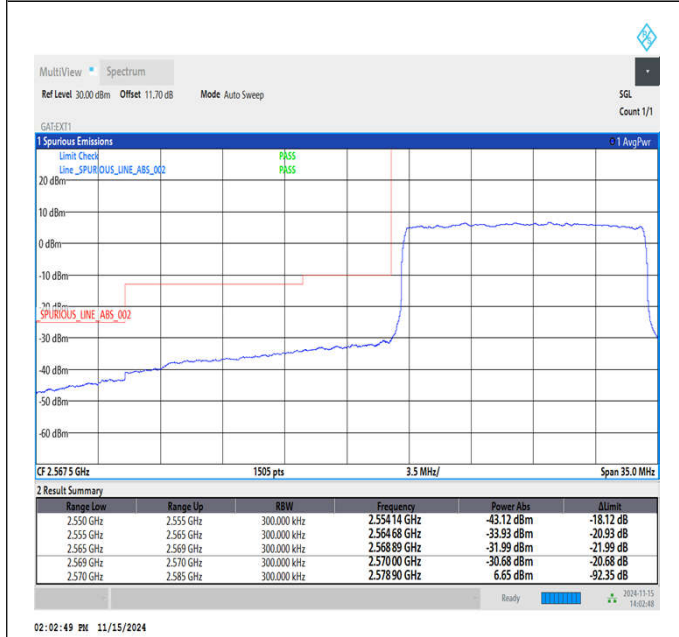
Band38_15MHz_16QAM_37825_75RB#0
