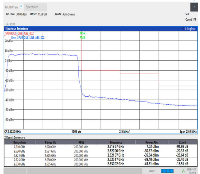
Band38_10MHz_16QAM_38200_50RB#0
