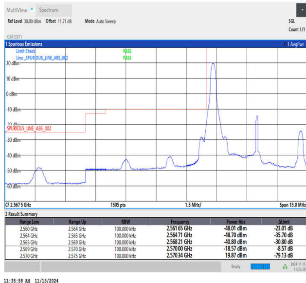
Band38_5MHz_16QAM_37775_1RB#0
