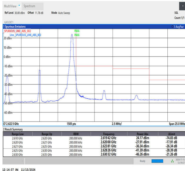
Band38_10MHz_QPSK_38200_1RB#49
