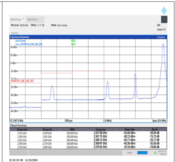
Band38_10MHz_QPSK_37800_1RB#49
