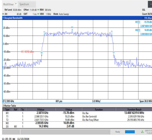
Band38-15MHz-16QAM-38000-75RB#0-PASS
