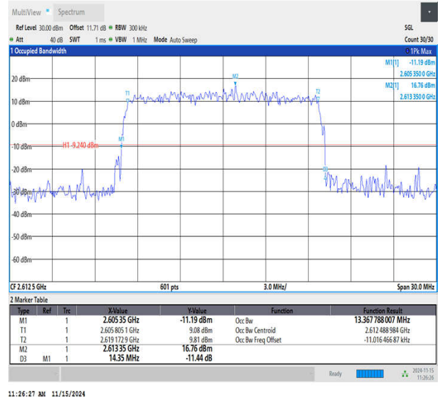
Band38-15MHz-16QAM-38175-75RB#0-PASS
