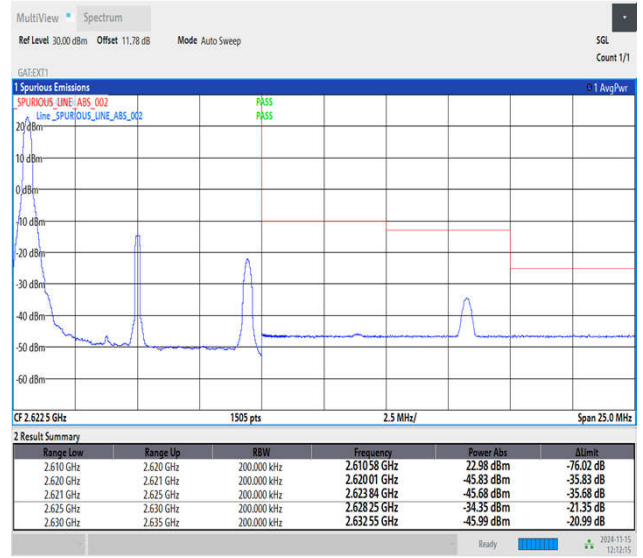
Band38_10MHz_16QAM_38200_1RB#0
