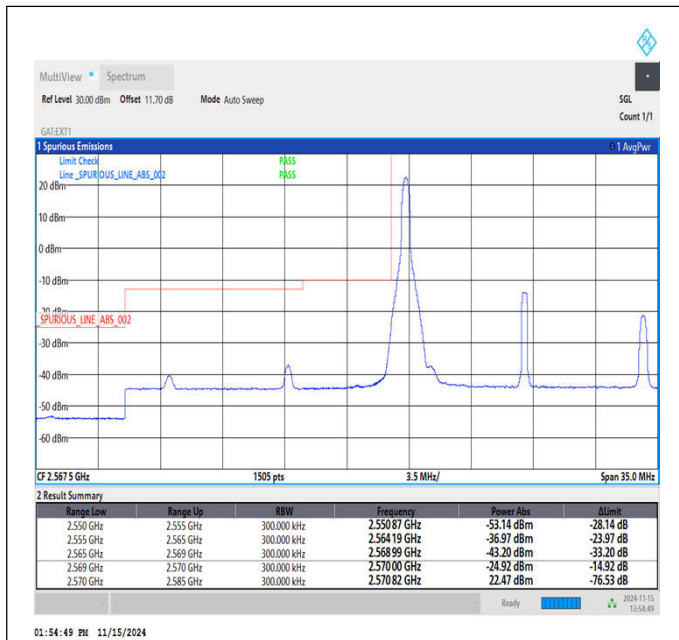
Band38_15MHz_16QAM_37825_1RB#0
