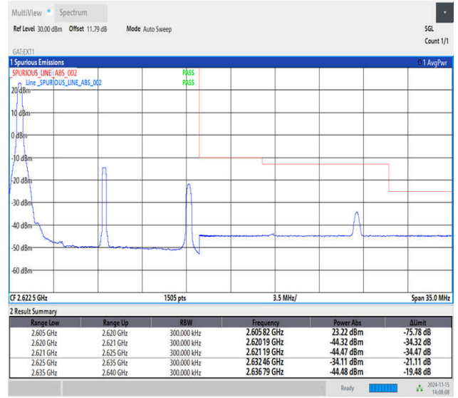
Band38_15MHz_64QAM_38175_1RB#0
