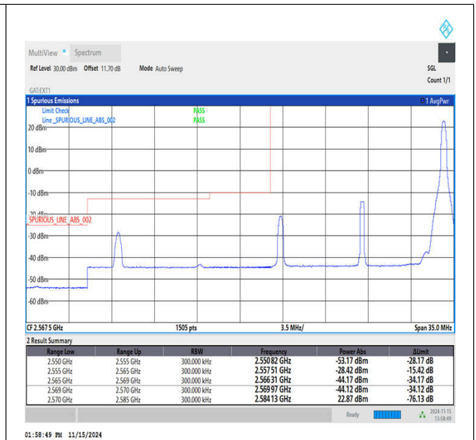
Band38_15MHz_16QAM_37825_1RB#74
