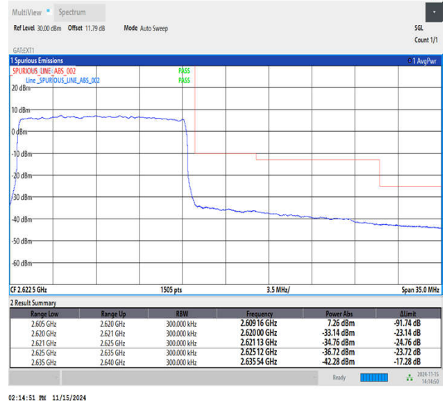
Band38_15MHz_16QAM_38175_75RB#0
