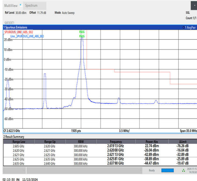
Band38_15MHz_16QAM_38175_1RB#74
