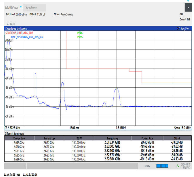
Band38_5MHz_16QAM_38225_1RB#0
