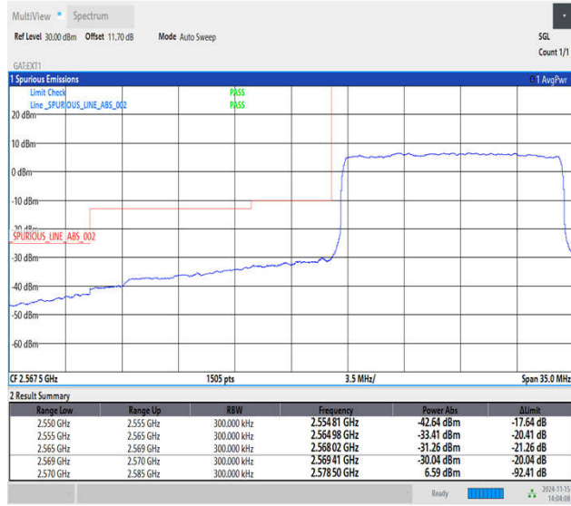
Band38_15MHz_64QAM_37825_75RB#0
