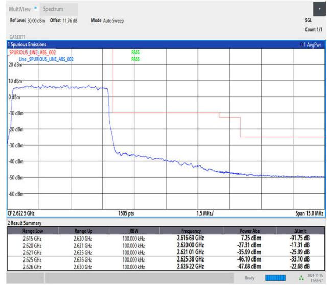
Band38_5MHz_16QAM_38225_25RB#0
