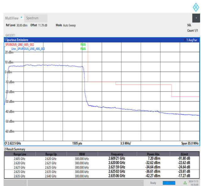
Band38_15MHz_64QAM_38175_1RB#0
