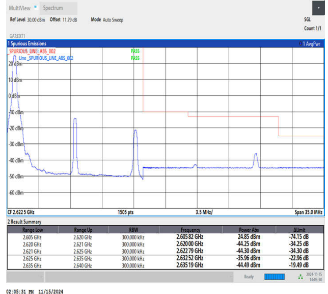
Band38_15MHz_QPSK_38175_1RB#0
