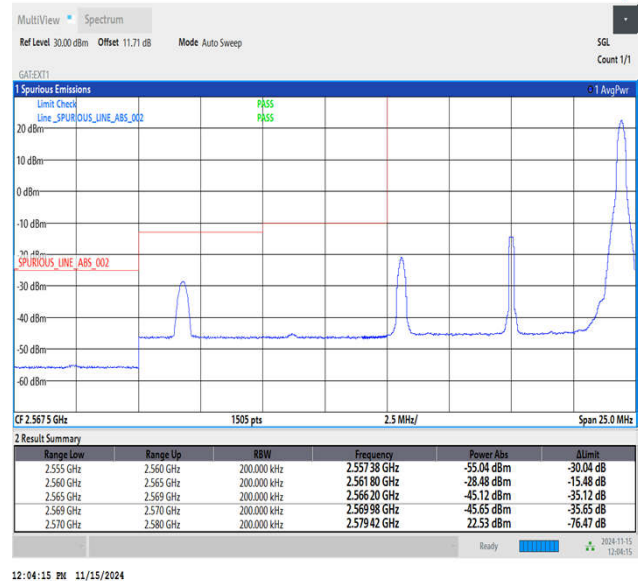
Band38_10MHz_16QAM_37800_1RB#49
