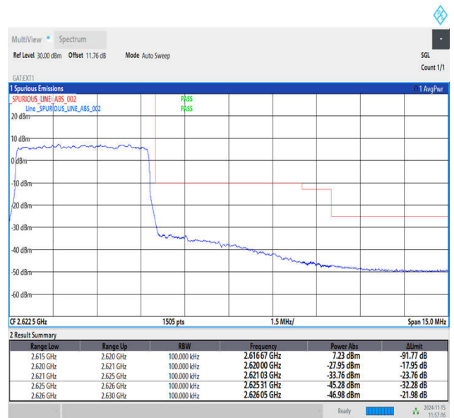
Band38_5MHz_64QAM_38225_1RB#0
