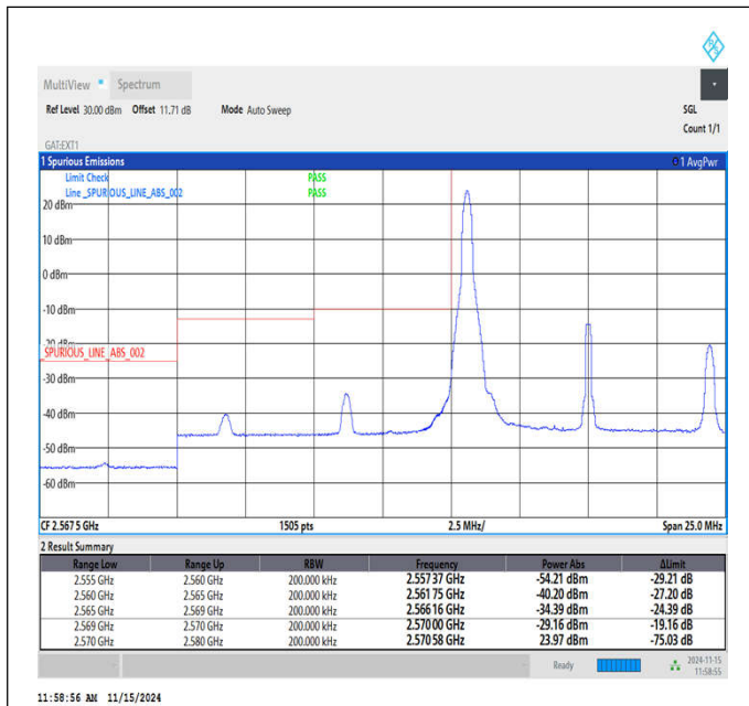
Band38_10MHz_QPSK_37800_1RB#0
