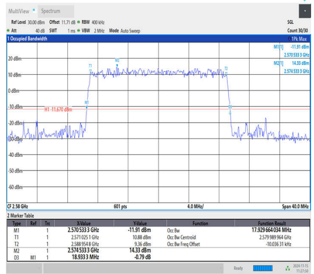
Band38-20MHz-64QAM-37850-100RB#0-PASS
