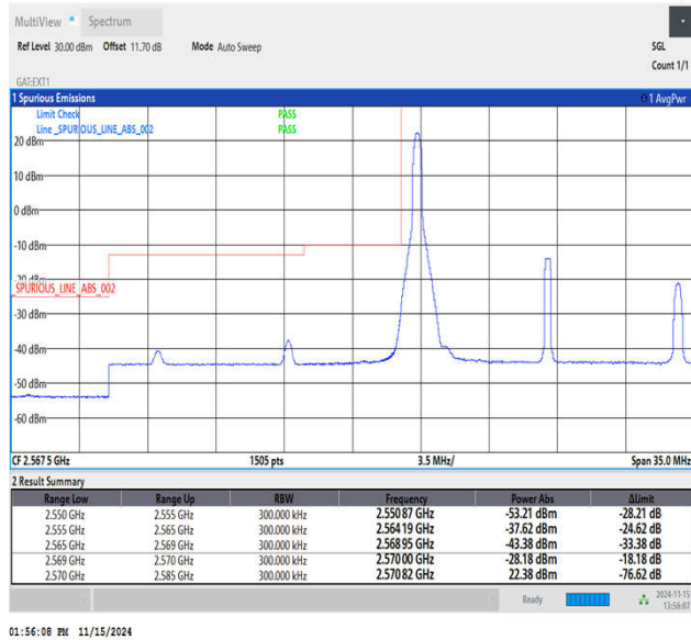
Band38_15MHz_64QAM_37825_1RB#0
