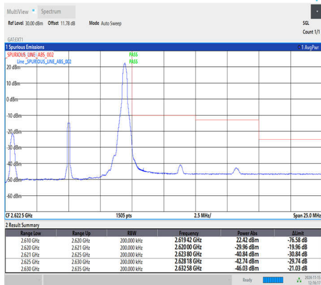
Band38_10MHz_16QAM_38200_1RB#49
