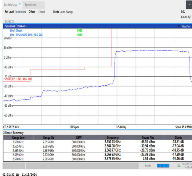
Band38_15MHz_QPSK_37825_75RB#0
