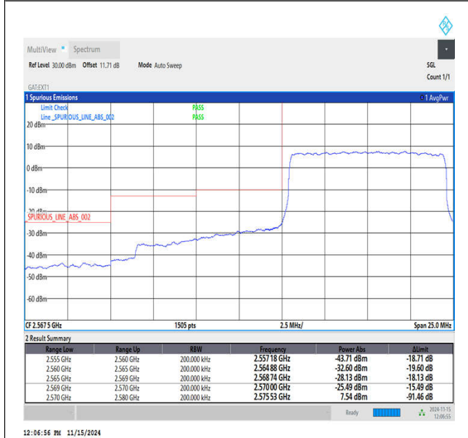
Band38_10MHz_QPSK_37800_50RB#0
