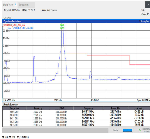
Band38_15MHz_QPSK_38175_1RB#74
