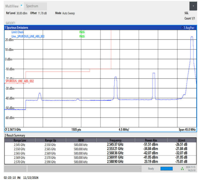
Band38_20MHz_16QAM_37850_1RB#99
