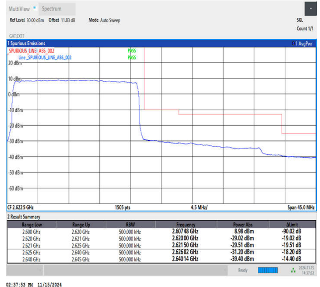
Band38_20MHz_QPSK_38150_100RB#0
