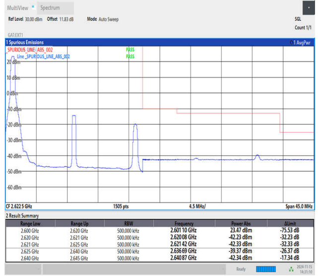
Band38_20MHz_16QAM_38150_1RB#0
