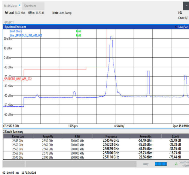
Band38_20MHz_16QAM_37850_1RB#0
