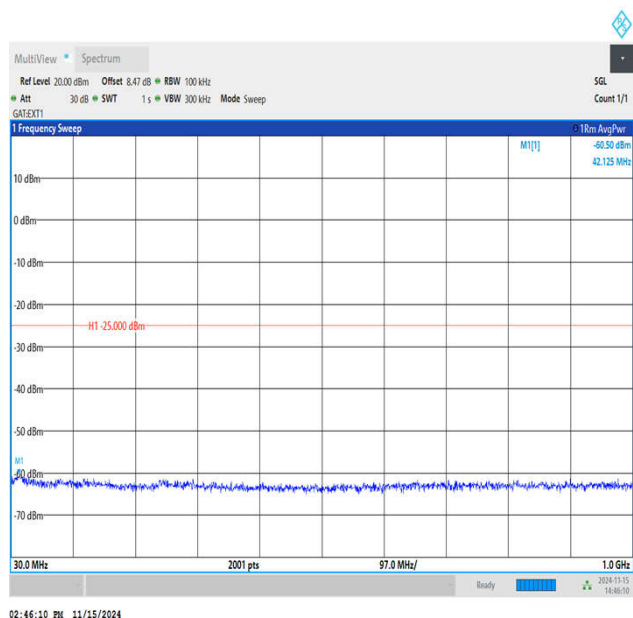
Band38_5MHz_QPSK_38000_1RB#0_30~1000_30~1000
