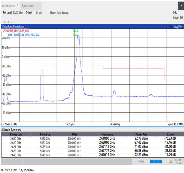
Band38_20MHz_16QAM_38150_1RB#99
