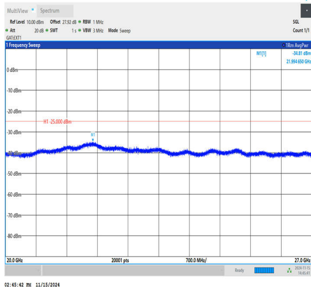
Band38_5MHz_QPSK_37775_1RB#0_20000~27000_20000~
