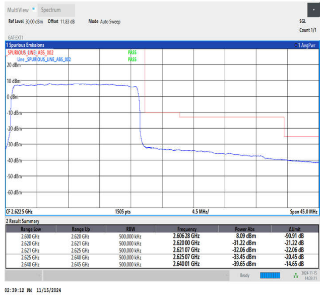
Band38_20MHz_16QAM_38150_100RB#0
