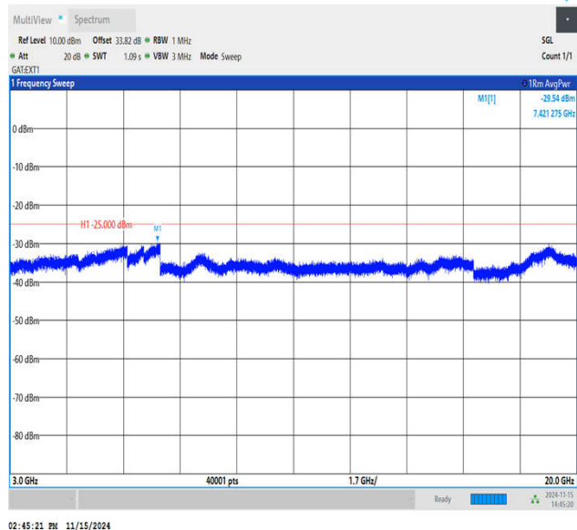
Band38_5MHz_QPSK_37775_1RB#0_3000~20000_3000~
