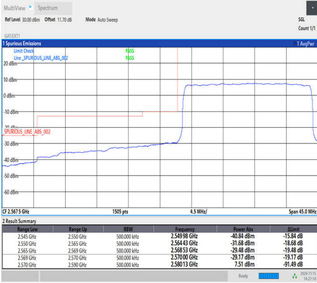
Band38_20MHz_16QAM_37850_100RB#0
