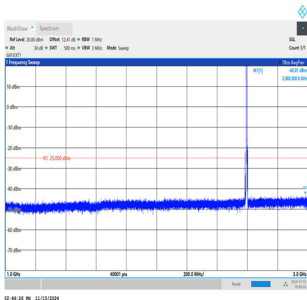
Band38_5MHz_QPSK_38000_1RB#0_1000~3000_1000~300
